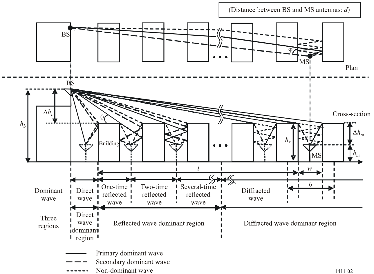
FIGURE 2 Definition of parameters for the NLoS1 case
