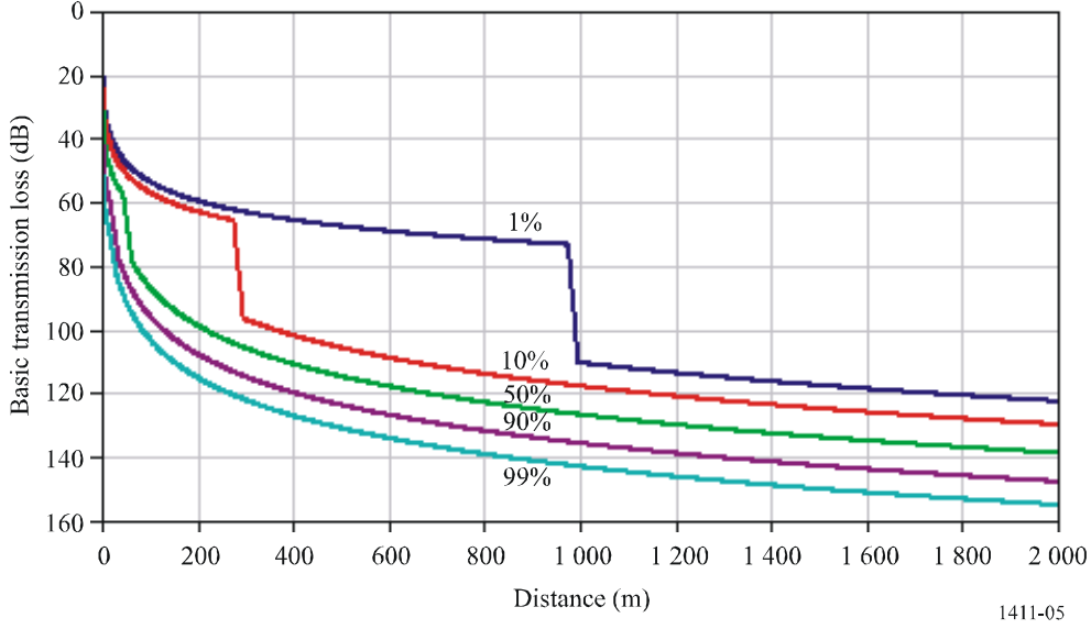
Curves of basic transmission loss not exceeded for 1, 10, 50, 90 and 99% of locations (frequency = 400 MHz, suburban)
