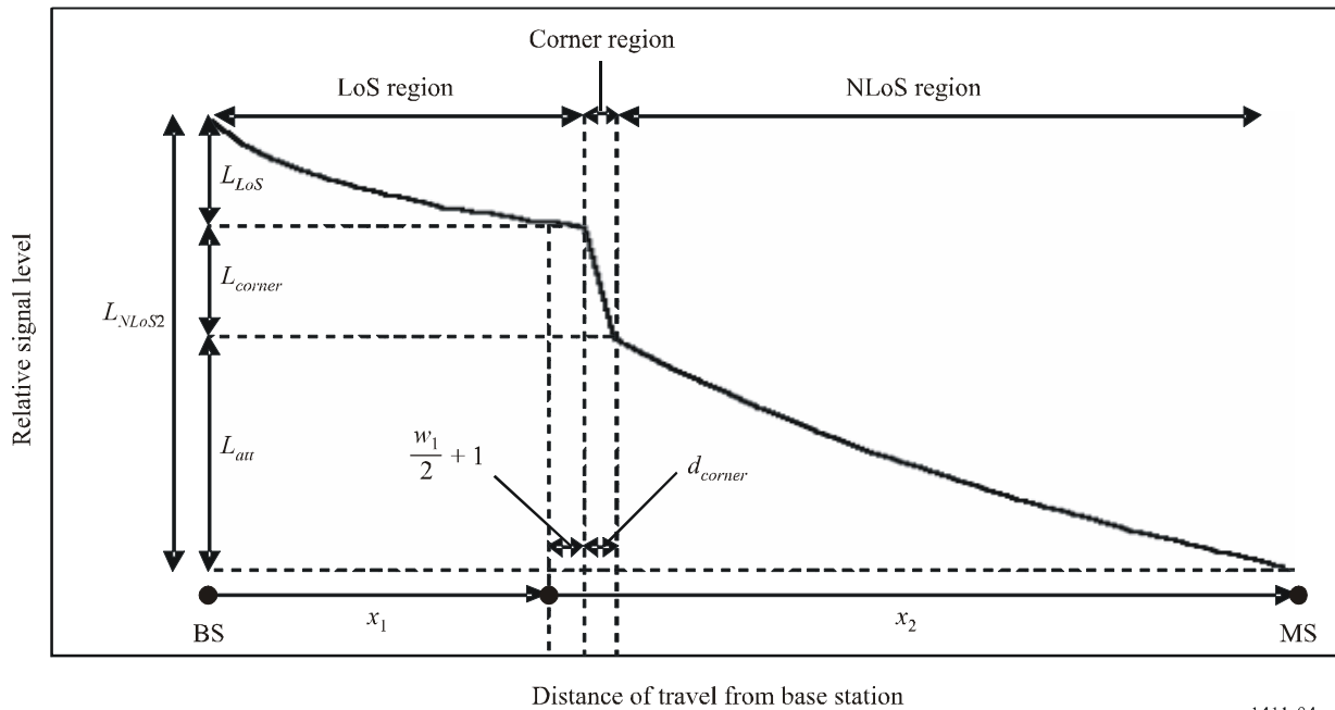
FIGURE 4 Typical trend of propagation along street canyons with low base station height for frequency range from 2 to 16 GHz
