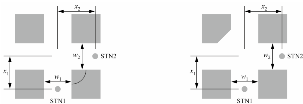
FIGURE 5 Case (1) Wedge shaped buildings layout Case (2) Chamfered shape buildings layout
