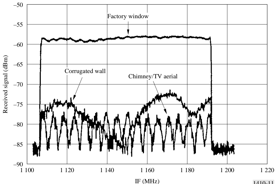
Frequency response for measured reflections at three different locations
