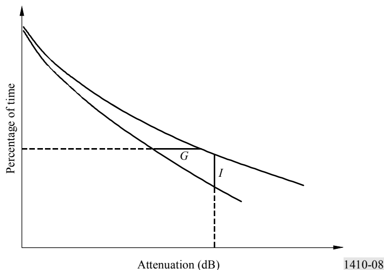
Example of attenuation statistics of path-angle diversity
