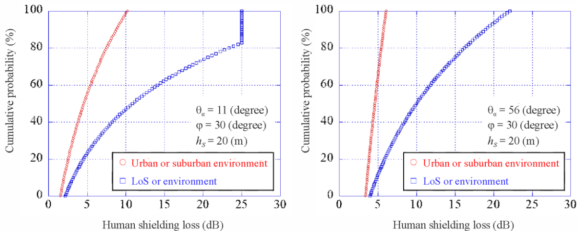
FIGURE 3 Cumulative distribution of the human shielding loss when antenna is at head height at f = 2 GHz
