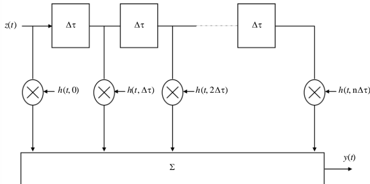
Tapped delay line model of multipath
