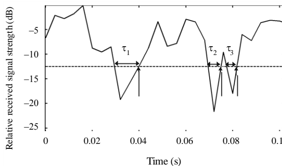
FIGURE 13 Received signal strength versus time
