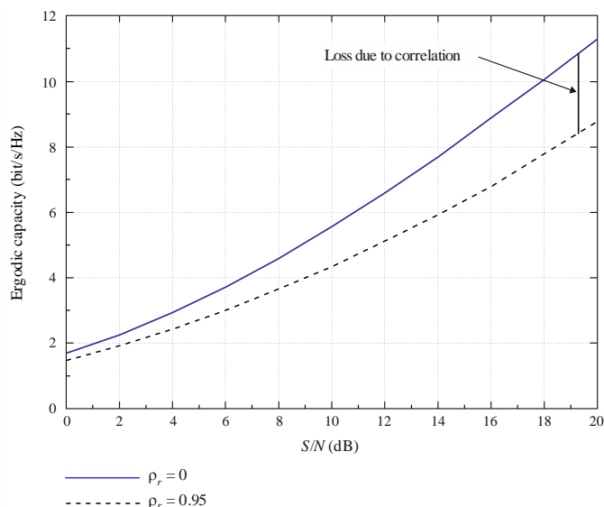
Ergodic capacity with low and high receive correlation
