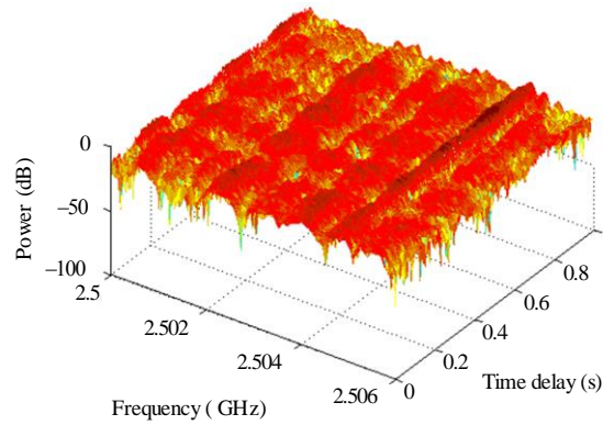
FIGURE 12 Small scale time variant frequency function
