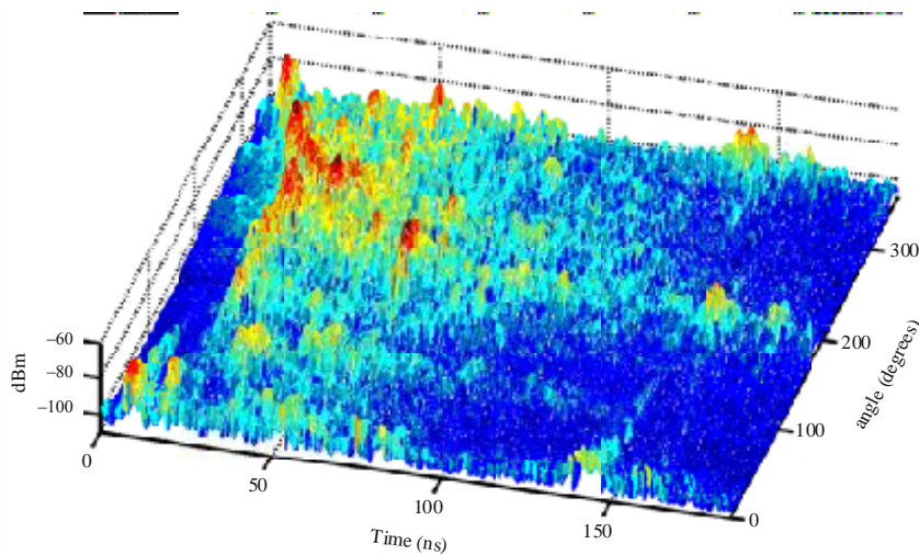
FIGURE 11 Directional power delay profiles
