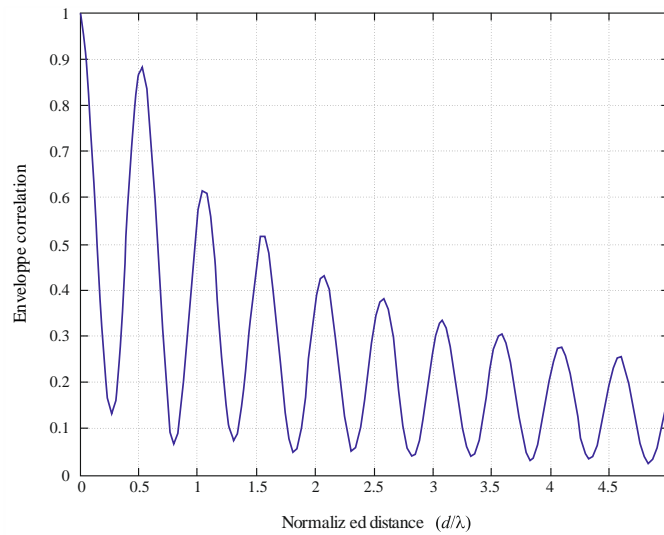
FIGURE 16 Resulting spatial correlation
