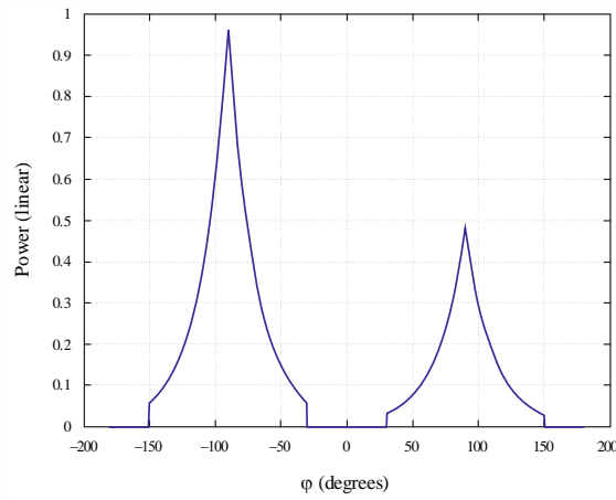
FIGURE 15 Ideal truncated Laplacian power-azimuth spectrum (PAS)
