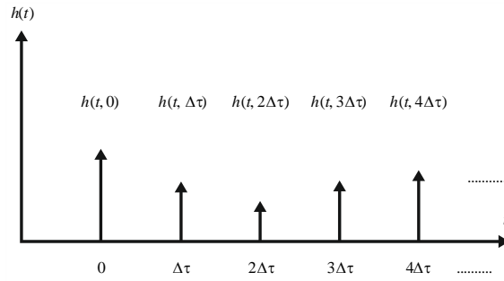
Example of multipaths used to generate the channel
