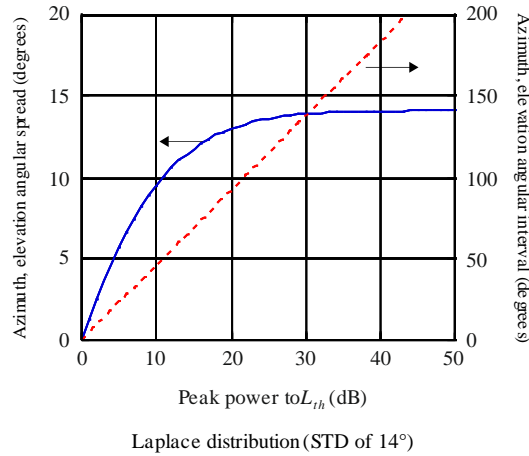
FIGURE 10 Example of effect for minimum peak-to- L_{th} ratio ( \Delta L )
