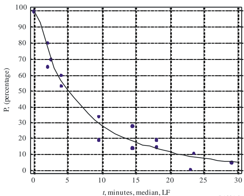
FIGURE 6 Number of excess durations (%) per hour for medium threshold on an LF link and integral distribution
