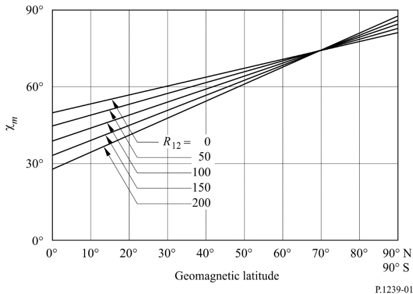
FIGURE 1 Variation of X_m with geomagnetic latitude and R_{12}
