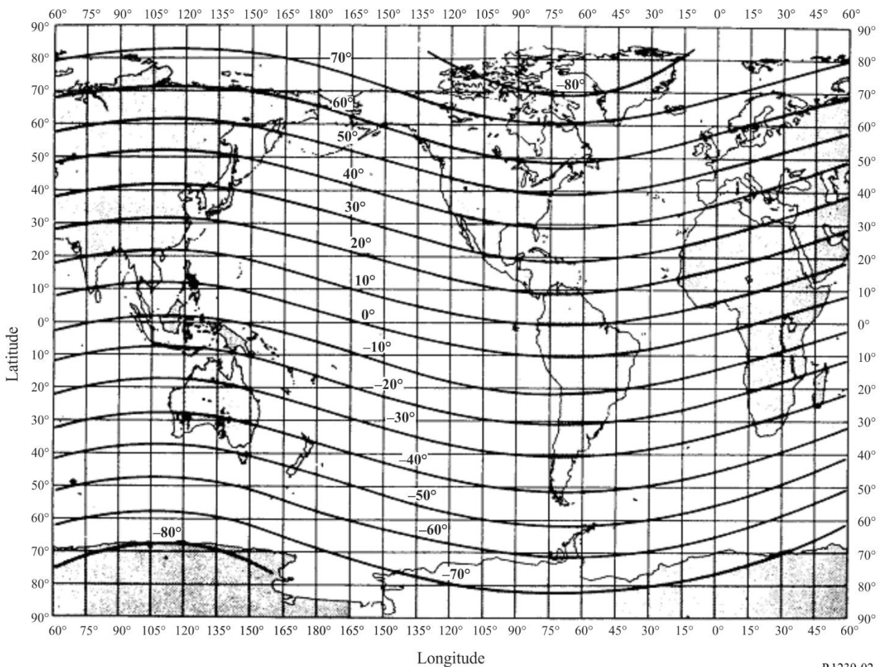
FIGURE 2 Geomagnetic latitudes
