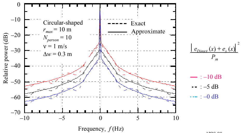
Power spectrum in circular room
