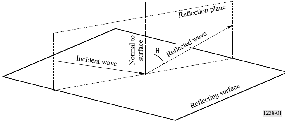
FIGURE 1 Geometry for calculating the reflection characteristics
