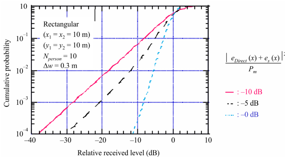
FIGURE 5 Cumulative probability of received level in circular room
