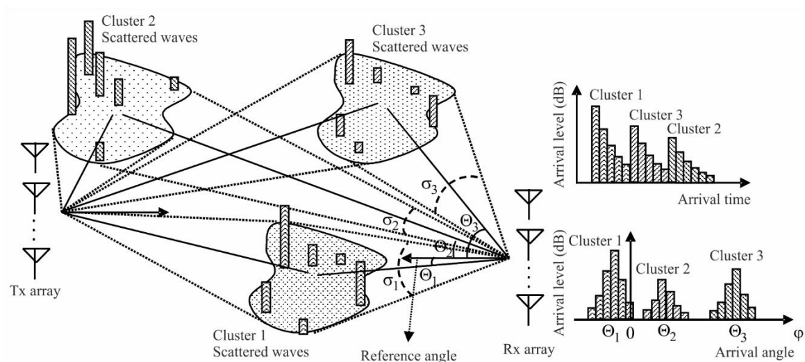
FIGURE 1 Image of cluster model
