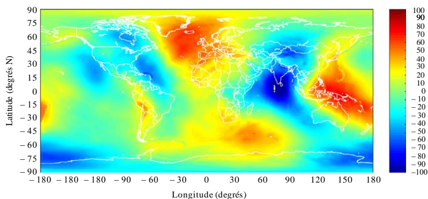
FIGURE 5 EGM2008 (m)
