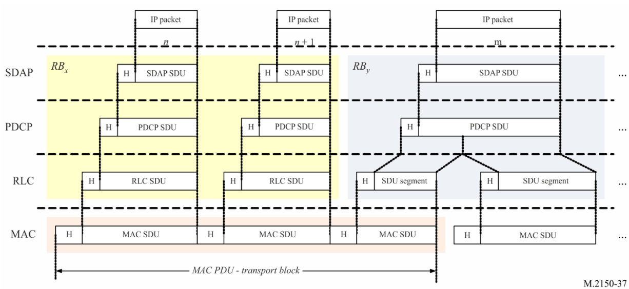
FIGURE 37 Data flow example
