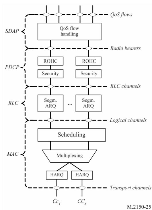
FIGURE 25 Layer 2 structure for UL with CA configured
