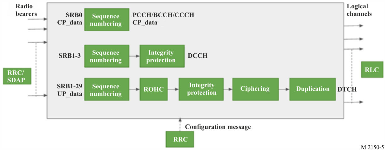
FIGURE 51 Downlink architecture of PDCP PDCP_DL_gNB
