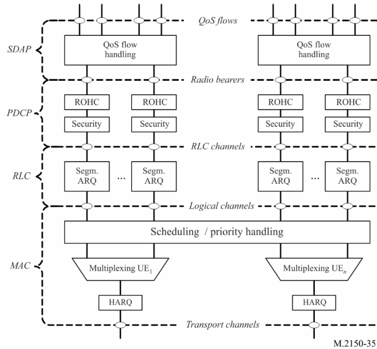
FIGURE 35 Downlink layer 2 structure
