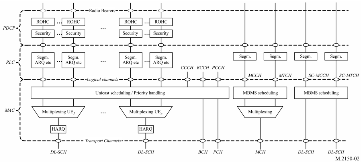
FIGURE 2 Downlink L2 protocol structure
