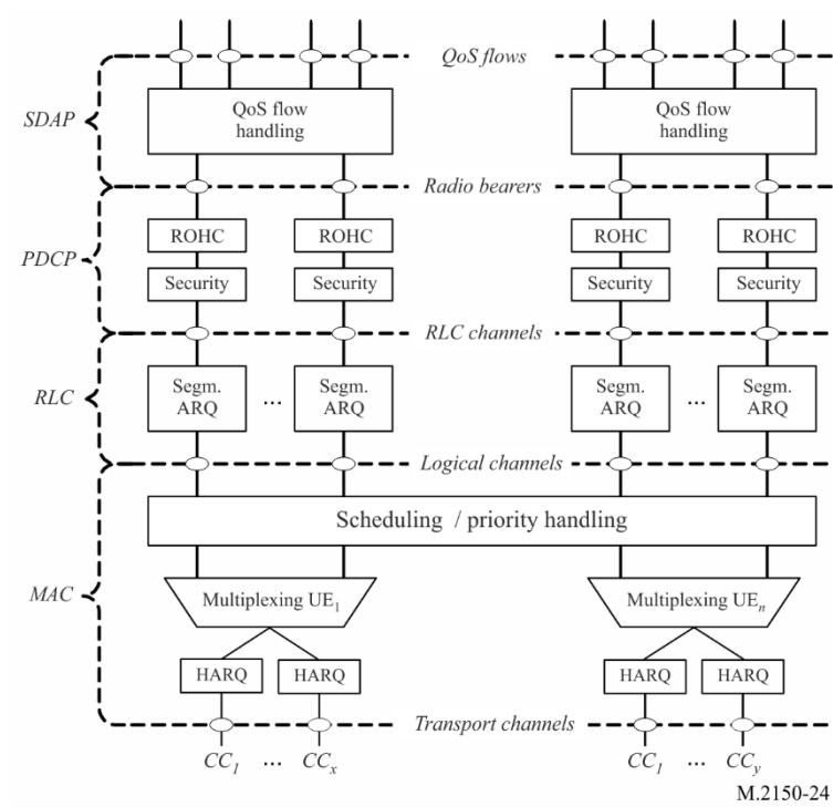
FIGURE 24 Layer 2 structure for DL with CA configured
