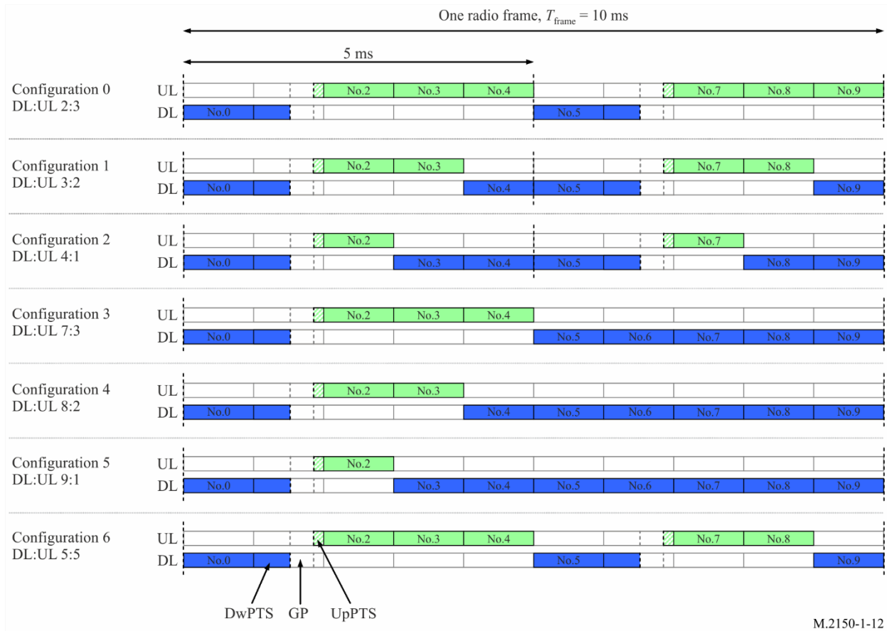
Uplink-downlink asymmetries supported by the E-UTRA/LTE RIT
