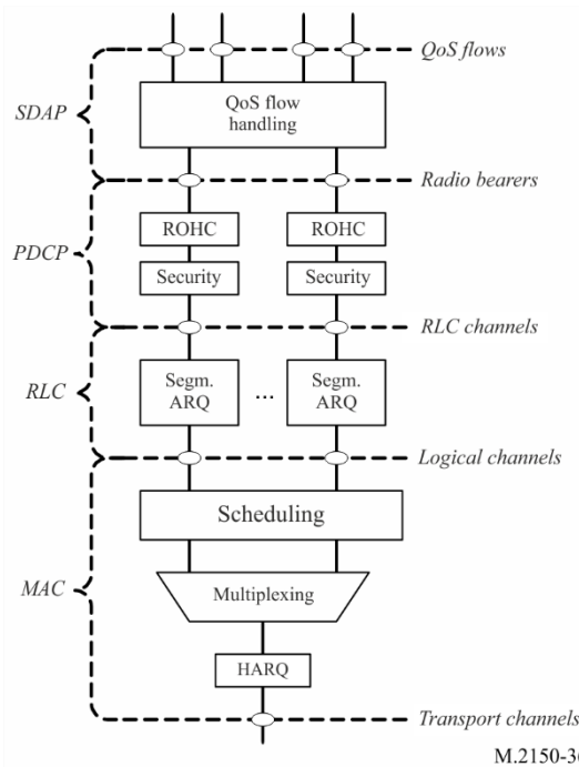
FIGURE 36 Uplink layer 2 structure
