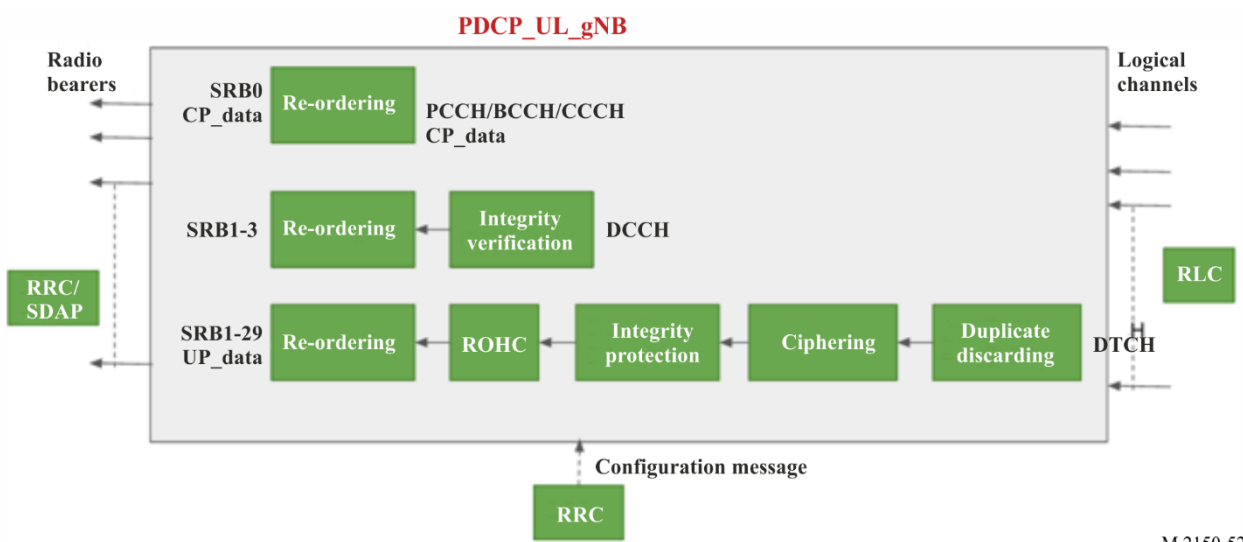
FIGURE 52 Uplink architecture of PDCP PDCP_UL_gNB
