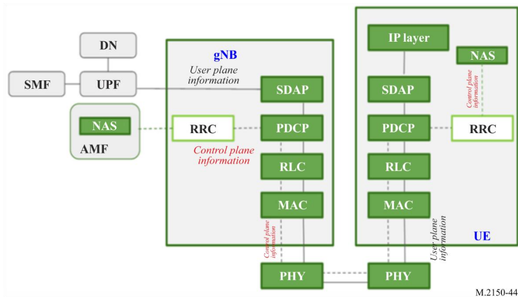
Architecture of TSDSI RIT logical layer
