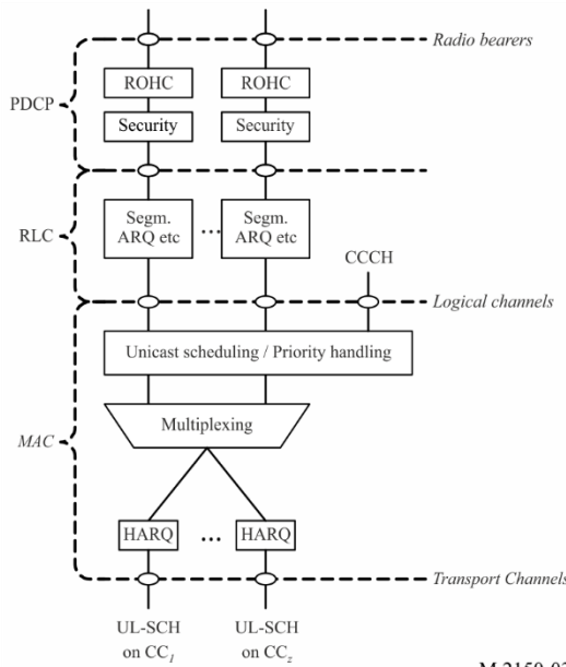
FIGURE 3 Uplink L2 protocol structure
