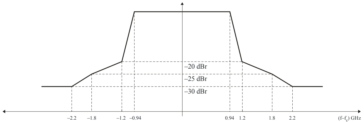
FIGURE 1 Spectral mask for single channel operation
