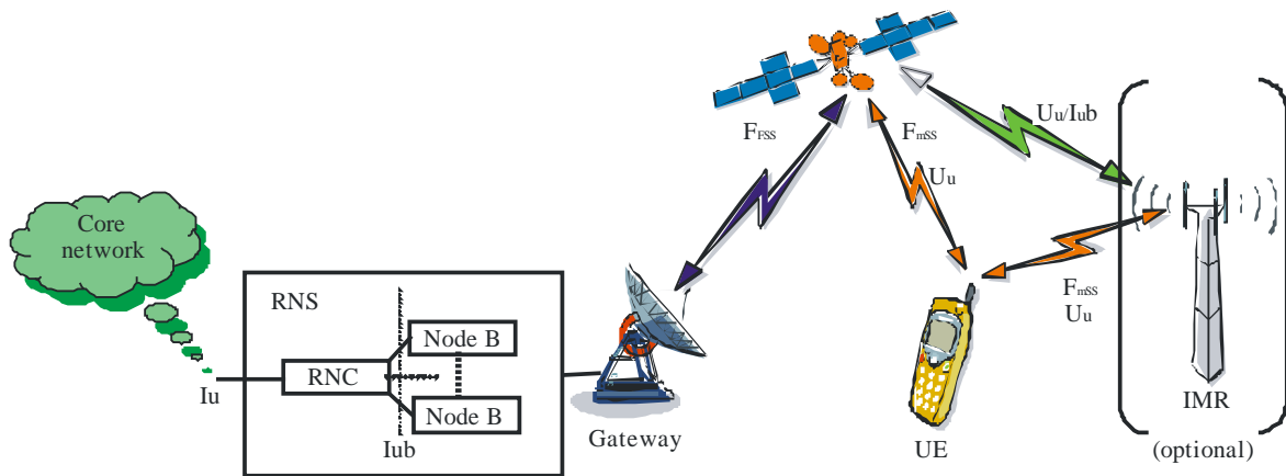
FIGURE 32 System architecture
