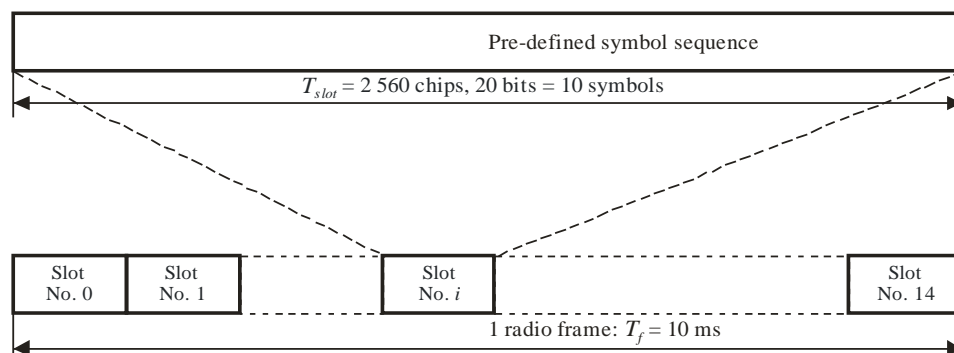
Frame structure of CPICH
