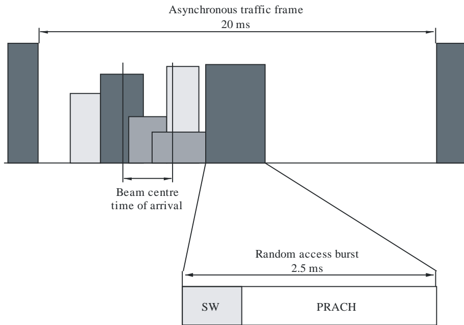
FIGURE 11 Asynchronous traffic in the return link, frame 0
