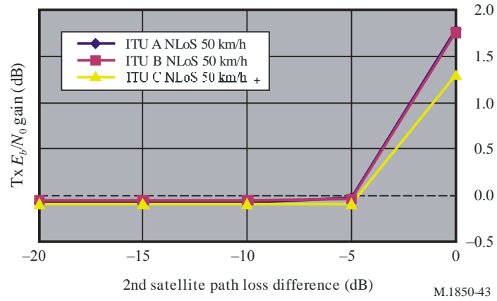
Satellite diversity gain; NLoS; Uplink; 64/144 kbit/s; 50 km/h
