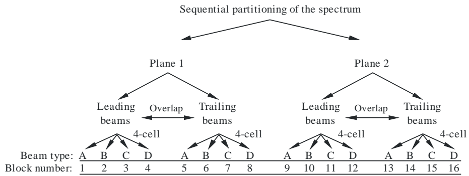
FIGURE 25 Example partitioning of the service link spectrum into frequency blocks
