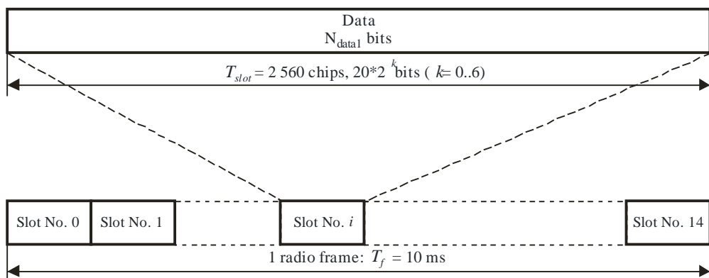
FIGURE 51 Frame structure of PDSCH
