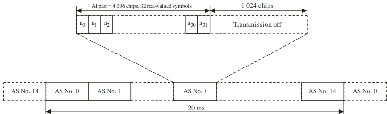
Structure of AICH
