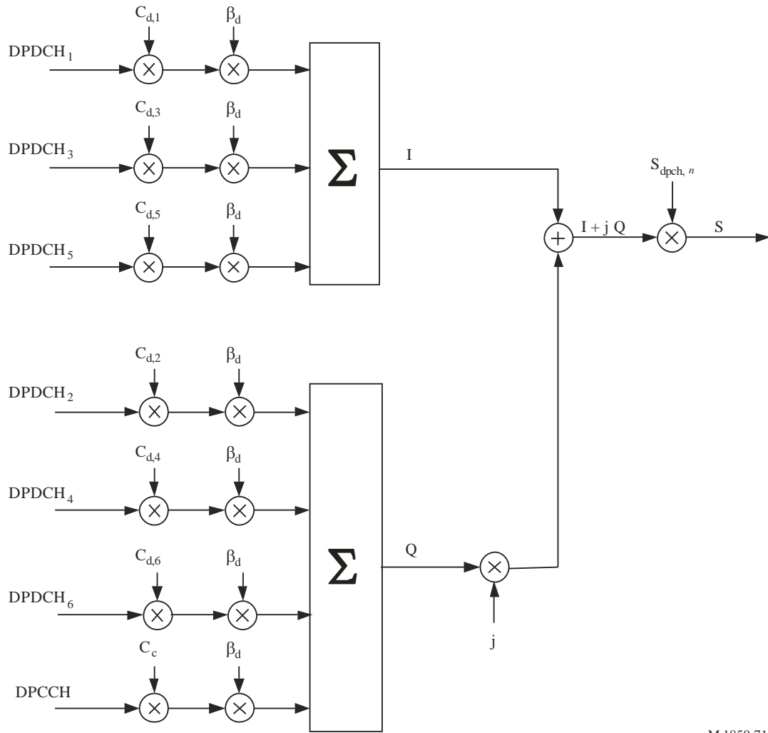
FIGURE 71 Uplink spreading
