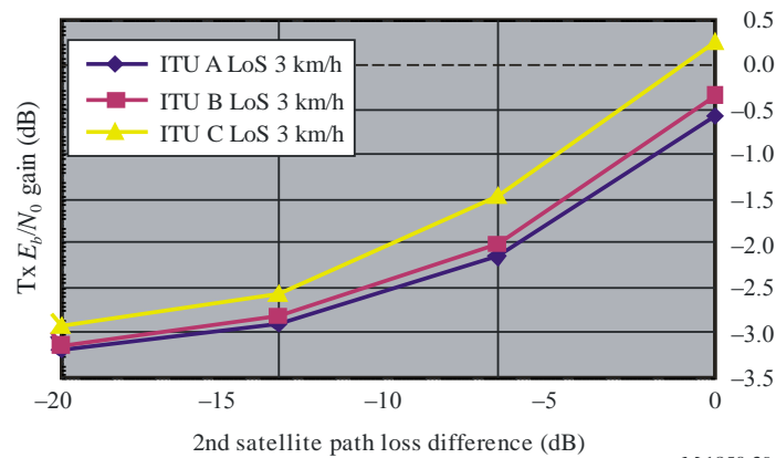
Satellite diversity gain; LoS; Downlink
