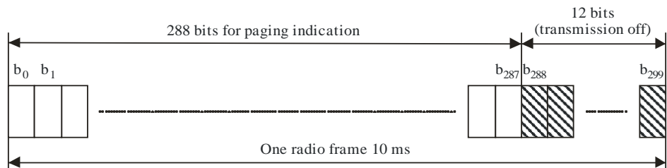
FIGURE 53 Structure of PICH
