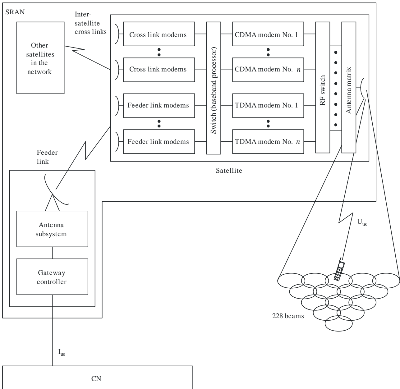
Architecture of Satcom2000
