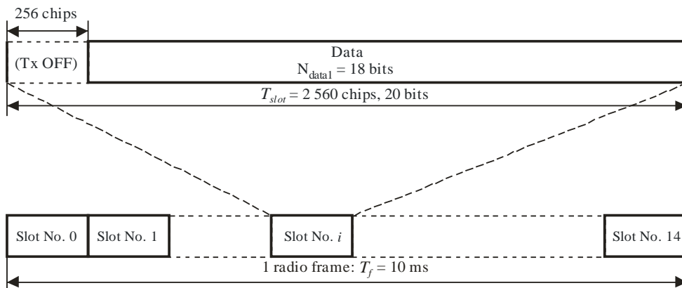
Frame structure of P-CCPCH
