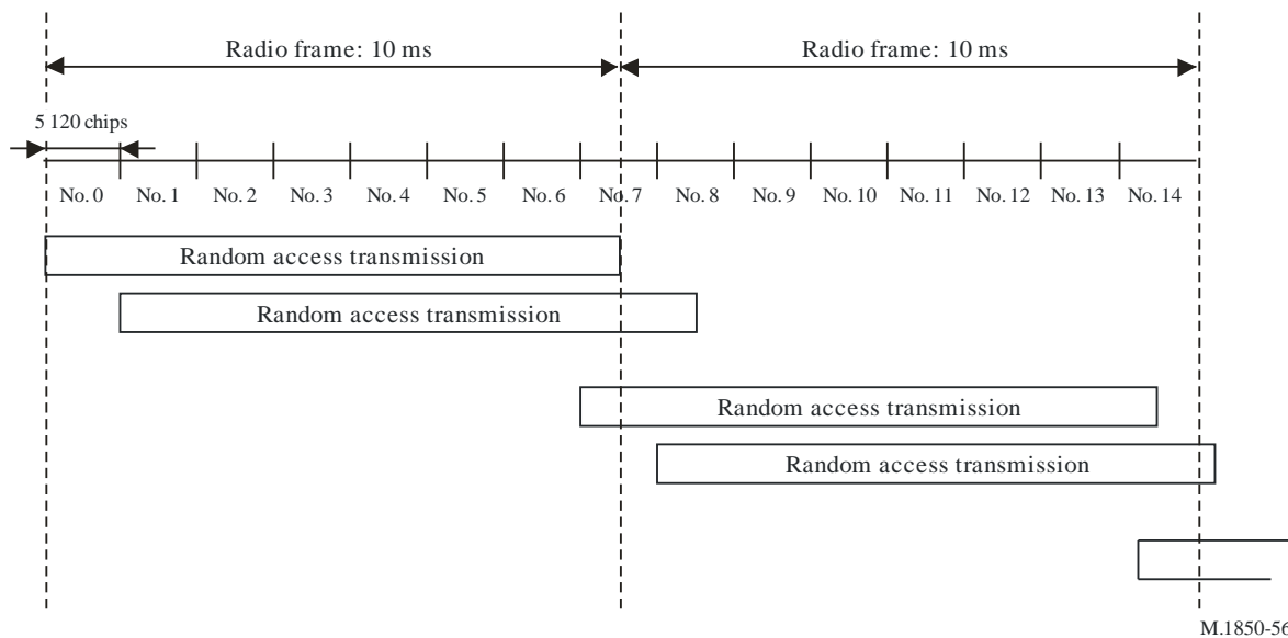
FIGURE 56 RACH access slot numbers and their spacing
