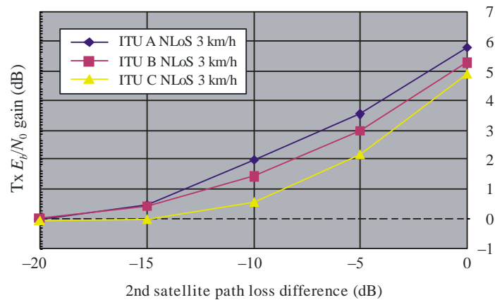
Satellite diversity gain; NLoS; Uplink; 12.2 kbit/s; 3 km/h
