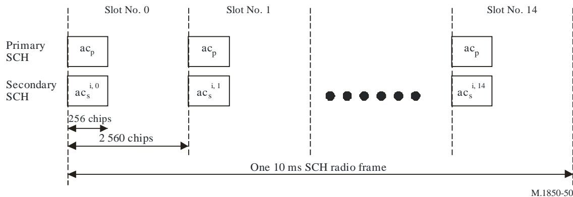
FIGURE 50 Structure of SCH
