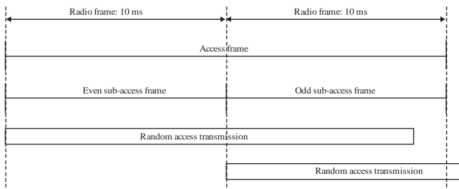
FIGURE 59 Structure of the random access transmission in optional mode C
