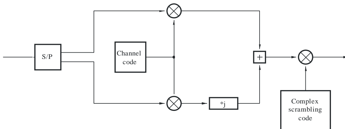
FIGURE 5 QPSK modulation/BPSK spreading for the forward link physical channels
