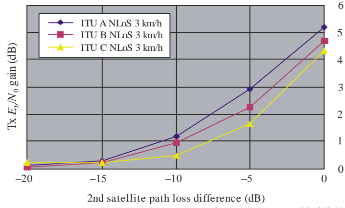
Satellite diversity gain; NLoS; Uplink; 64/144 kbit/s; 3 km/h
