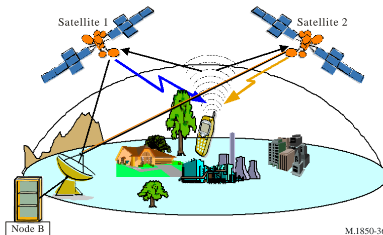
FIGURE 36 Satellite diversity
