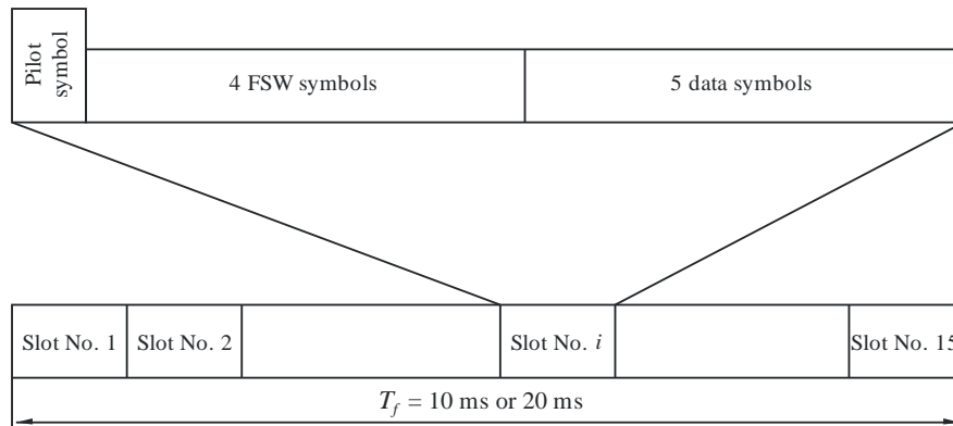
FIGURE 4 Frame structure for the CCPCH
