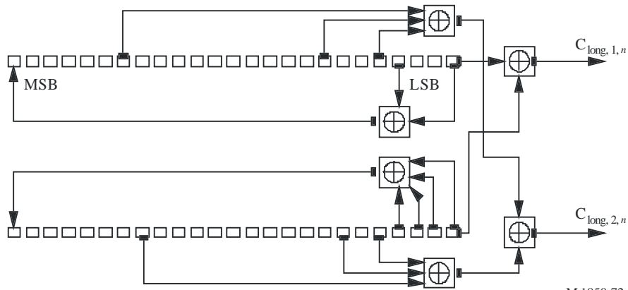
FIGURE 72 Long code generator for uplink
