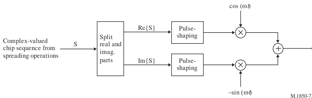
FIGURE 73 Uplink modulation
