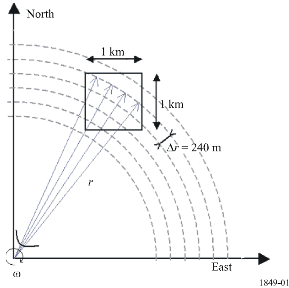
FIGURE 1 Pulse pair and range gate Cartesian projection
