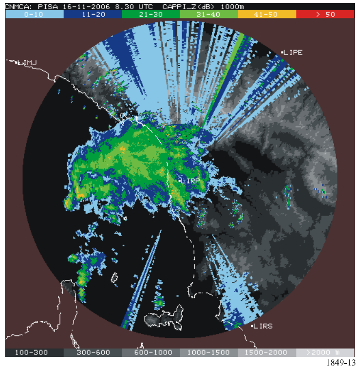
FIGURE 13 Interference to meteorological radar (precipitation mode)
