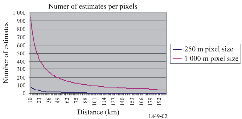
FIGURE 2 Pixel estimate versus distance
