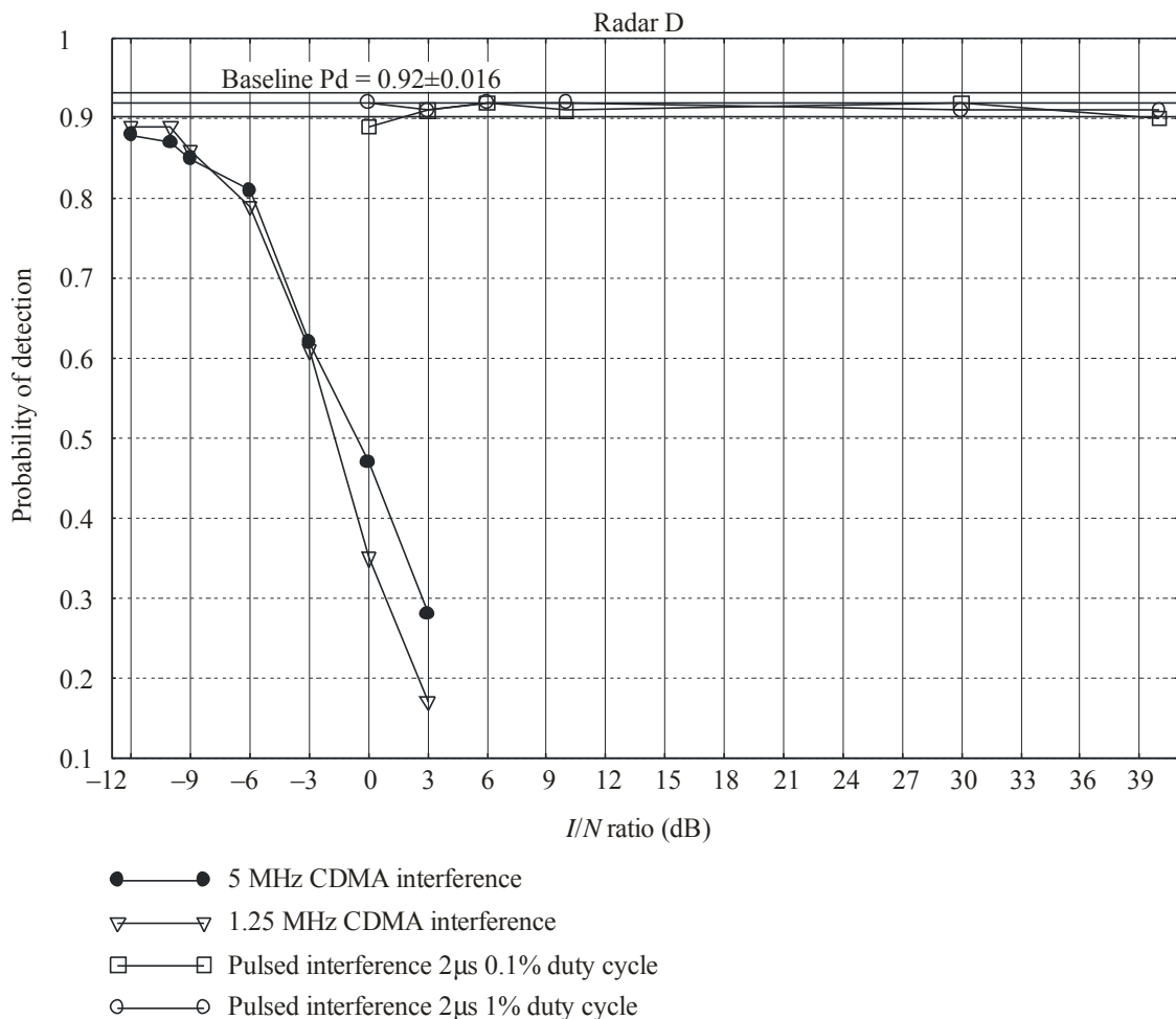
FIGURE 2 Radar D P_d curves
