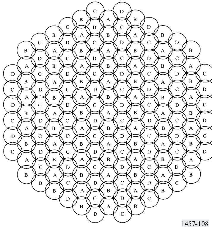
FIGURE 108 Typical 4-cell frequency reuse pattern
