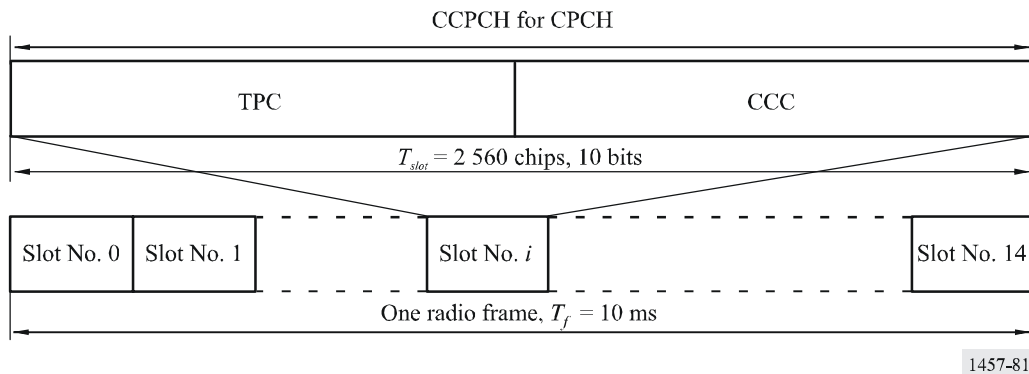
FIGURE 81 Frame structure for downlink CPCH-CCPCH
