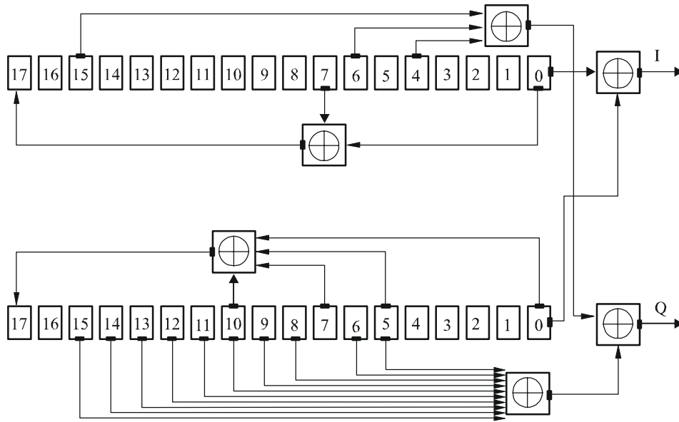
FIGURE 102 Downlink scrambling code generator
