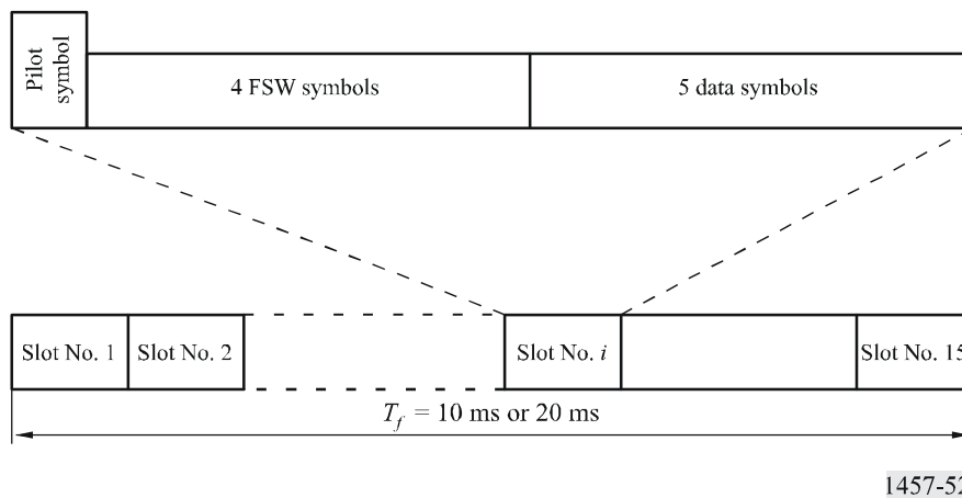
FIGURE 52 Frame structure for the common control physical channels (CCPCH)
