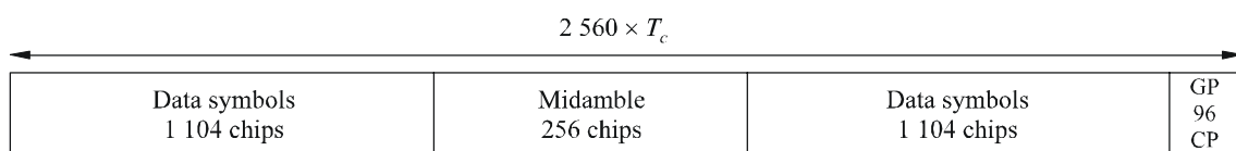
FIGURE 33 Burst structure of the burst type 2 (GP denotes the guard period and CP the chip periods)
