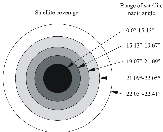
FIGURE 112 Definition of e.i.r.p. specification areas from a satellite
