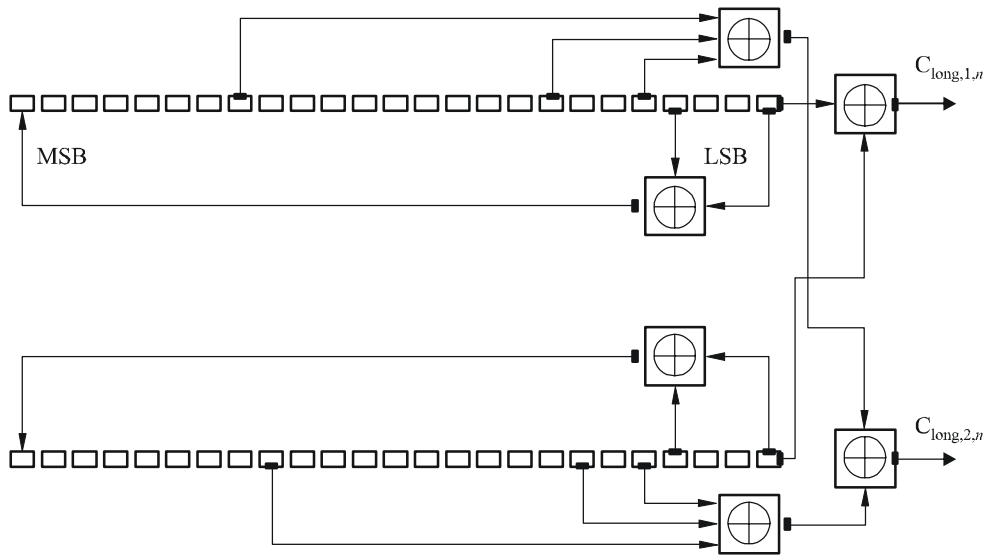
FIGURE 99 Uplink long code generator
