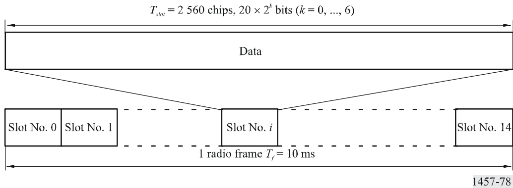
FIGURE 78 Frame structure for physical downlink shared channel (PDSCH)
