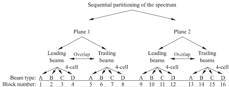
FIGURE 109 Example partitioning of the service link spectrum into frequency blocks
