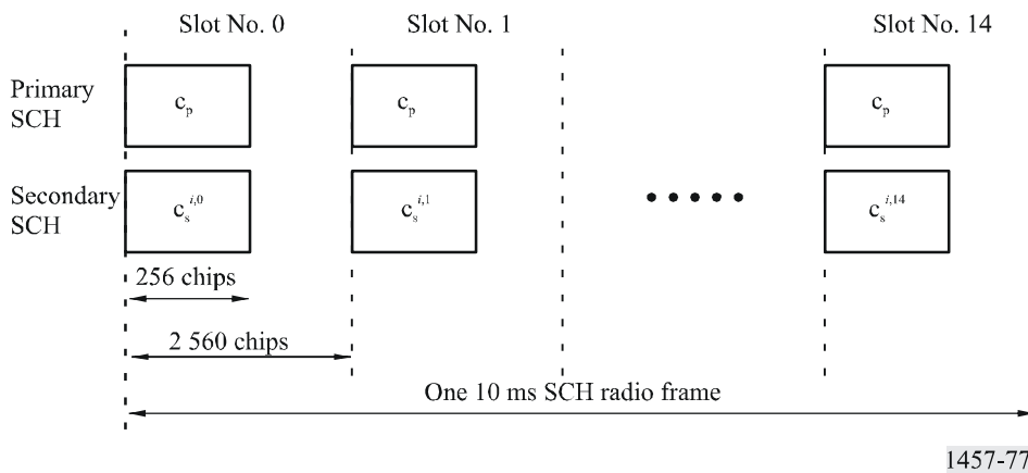
FIGURE 77 Structure of synchronization channel (SCH)
