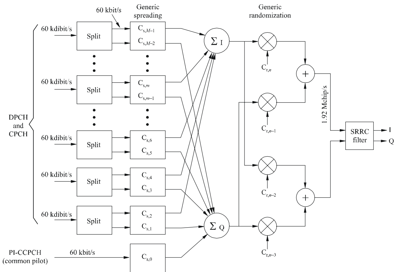
Forward link generic spreader and modulator (rates indicated refer to the 1.920 Mchip/s option and a spreading factor of 32)
