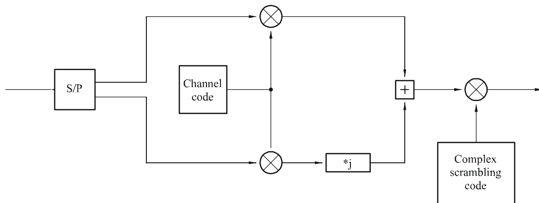
FIGURE 53 QPSK modulation/BPSK spreading for the forward link physical channels
