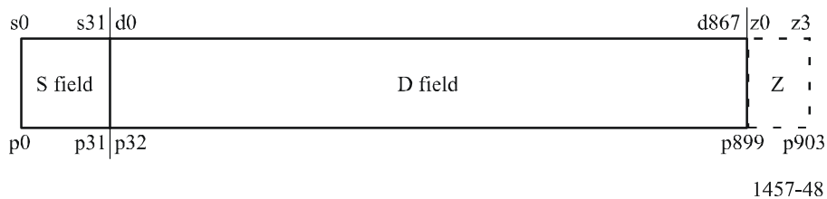
FIGURE 48 Packet P80
