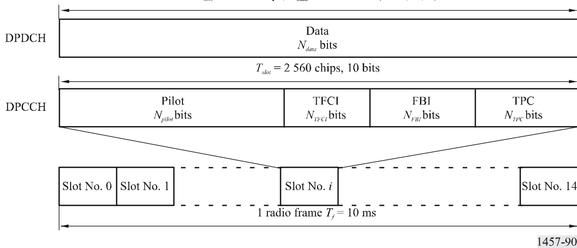
Frame structure of uplink DPCH
