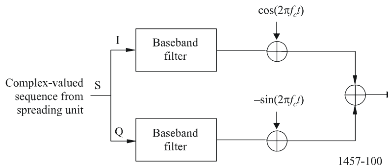
FIGURE 100 Uplink modulation
