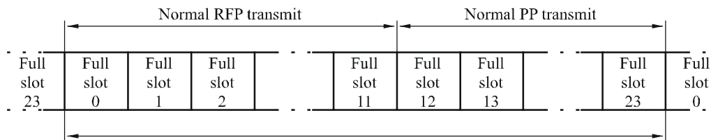
FIGURE 44 Frame structure using full slot format
