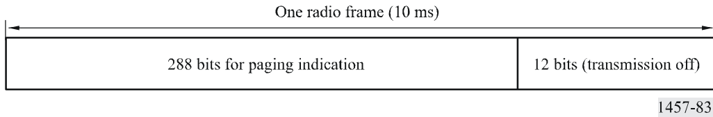
FIGURE 83 Structure of paging indicator channel (PICH)
