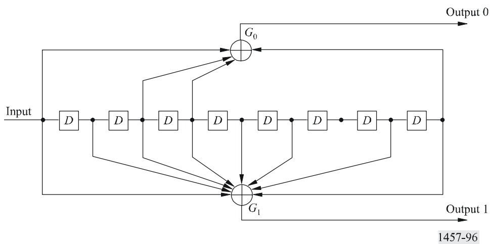
FIGURE 96 Rate 1/2, constraint length = 9 convolutional code generator
