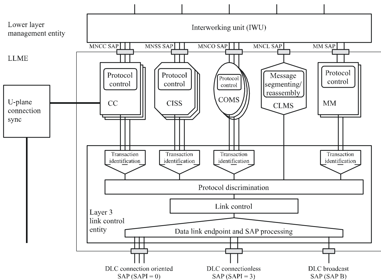
FIGURE 49 Network layer
