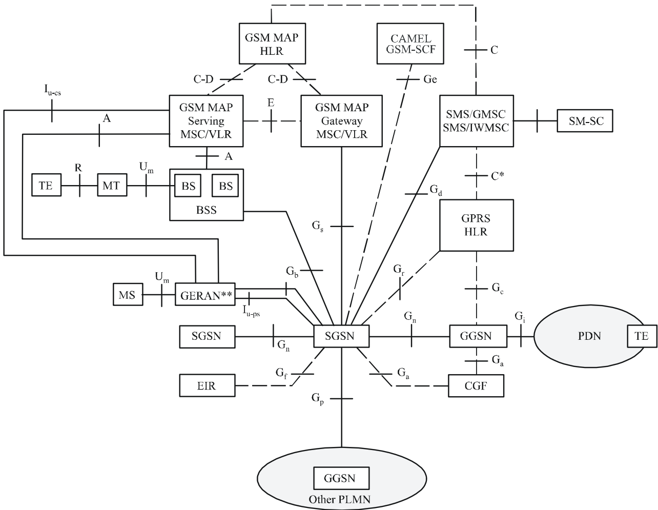
FIGURE 40b Network elements and associated reference points
