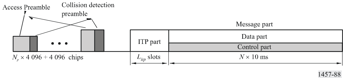
FIGURE 88 Structure of the CPCH access transmission
