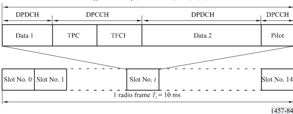
FIGURE 84 Frame structure of downlink DPCH T_{slot} = 2\ 560 chips, 10 \times 2^k bits ( k = 0, \dots, 7 )
