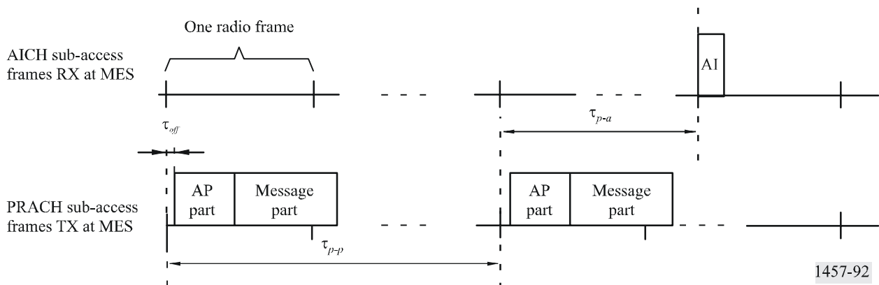
Timing relation between PRACH and AICH as seen at the MES
