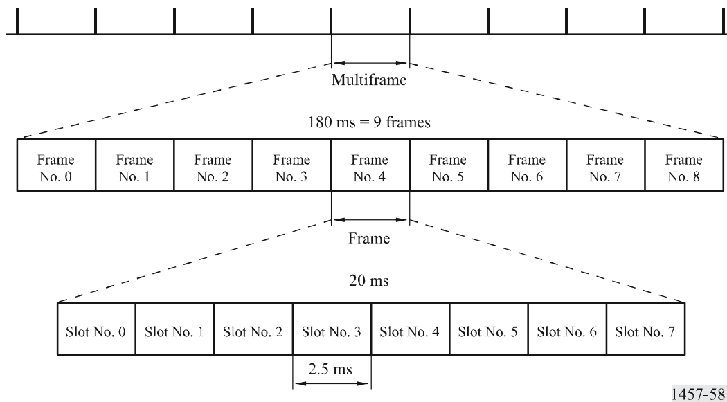
FIGURE 58 Forward and return link frame structure
