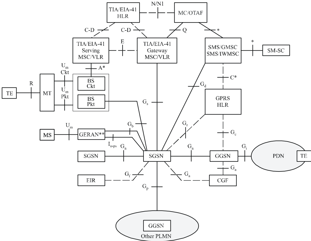
FIGURE 40a Network elements and associated reference points
