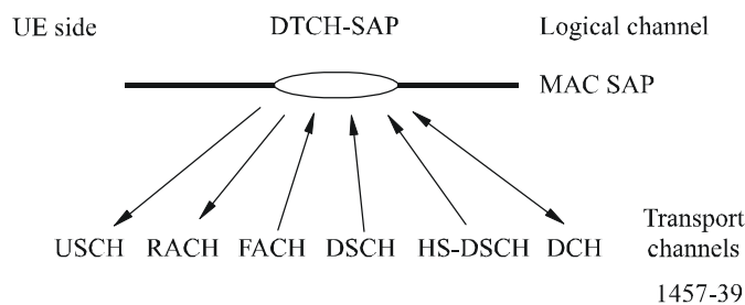
The possible transport channel mappings of the dedicated traffic channel (DTCH) (The arrows show the direction of the channel (UE side). The directions are reversed from the network side)
