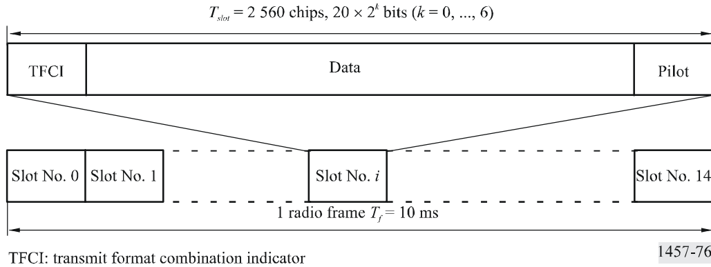
FIGURE 76 Frame structure for secondary common control physical channel (S-CCPCH)
