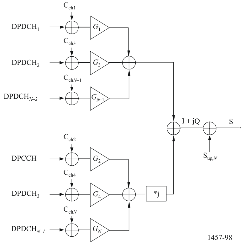
FIGURE 98 Spreading for uplink DPDCH/DPCCH
