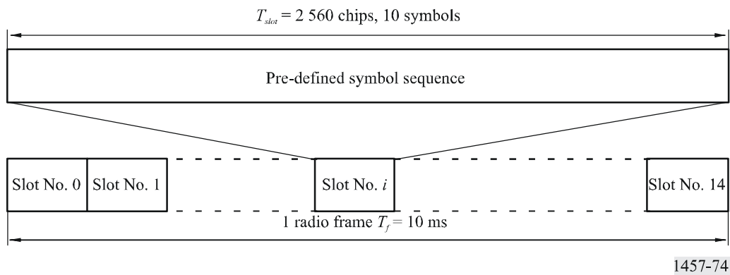
FIGURE 74 Frame structure for common pilot channel (CPICH)
