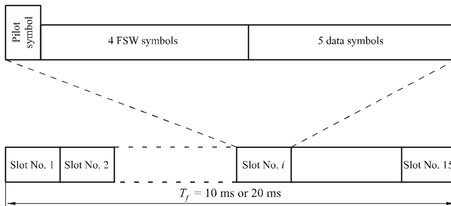
FIGURE 52 Frame structure for the common control physical channels (CCPCH)
