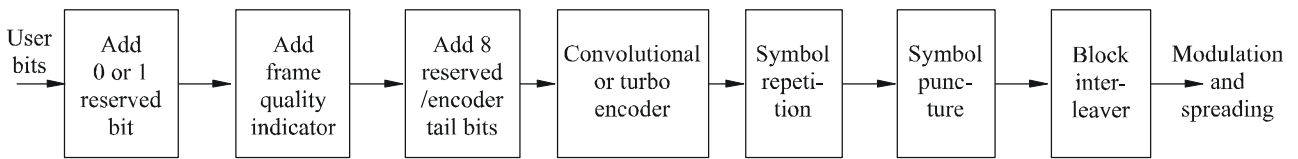
FIGURE 15 Reverse channels structure (except the pilot channel)
