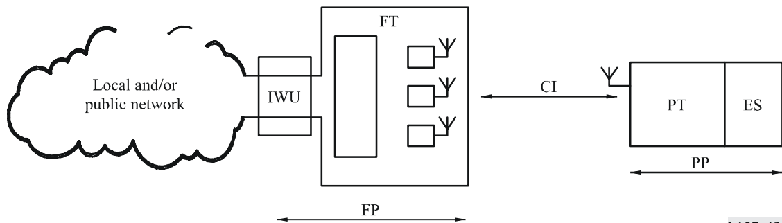
FIGURE 43 The CI structure
