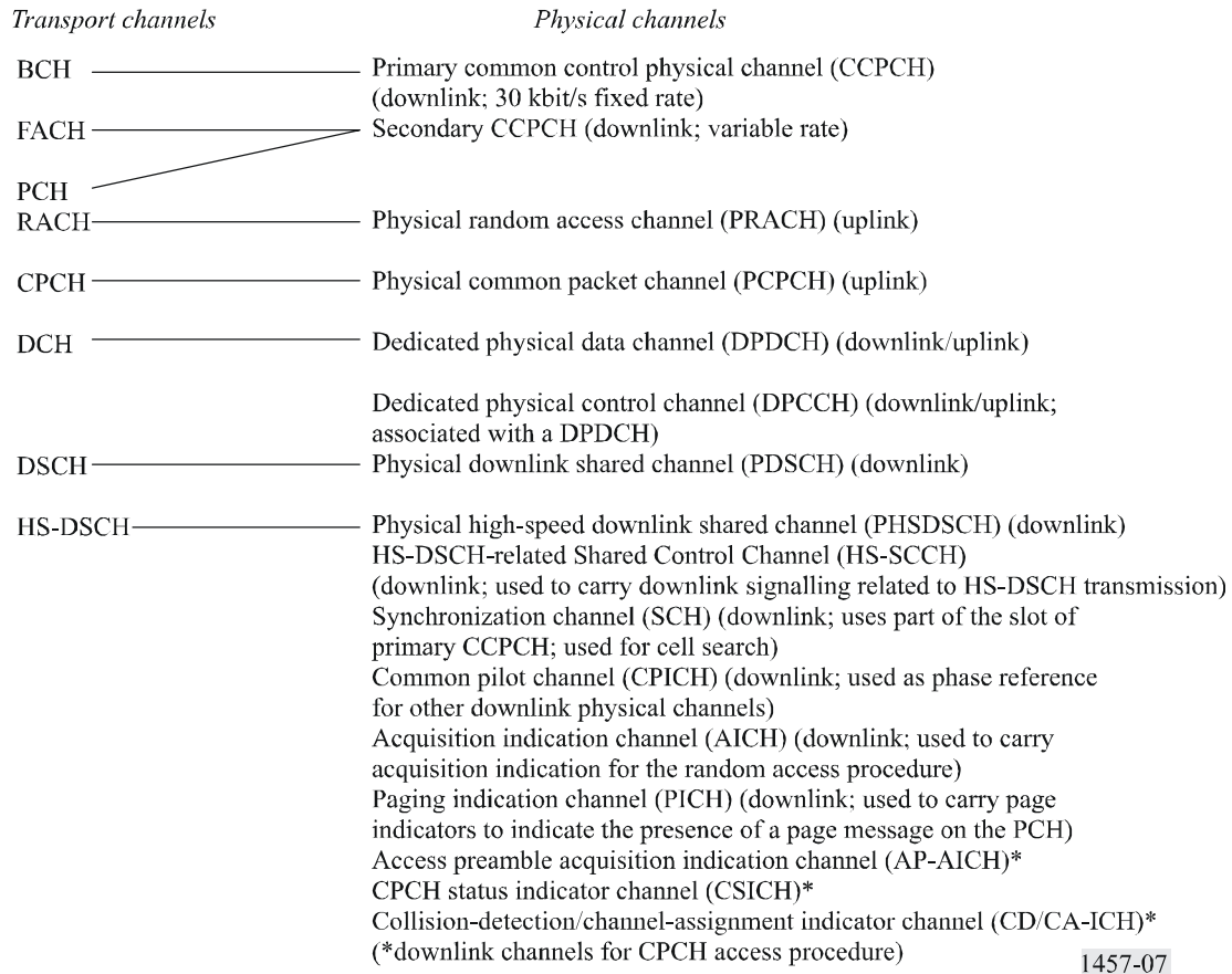
FIGURE 7 Transport channels, physical channels and their mapping
