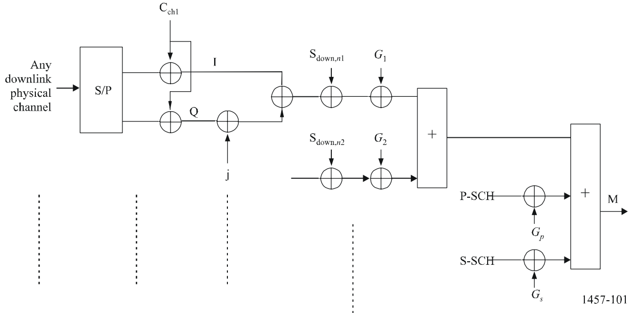
FIGURE 101 Spreading for downlink physical channels
