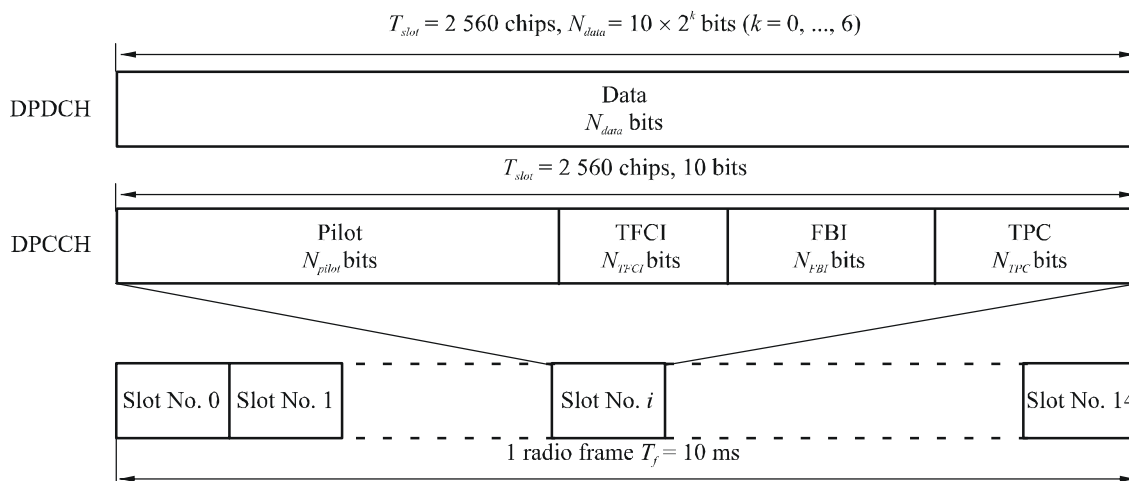
FIGURE 90 Frame structure of uplink DPCH
