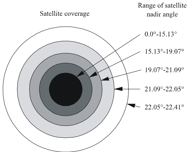
Definition of e.i.r.p. specification areas from a satellite
