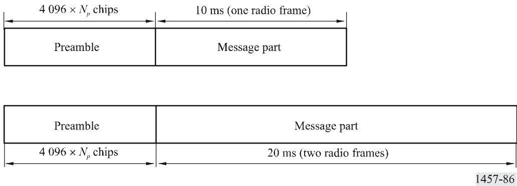
FIGURE 86 Structure of the random access transmission
