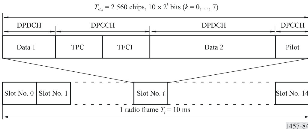
FIGURE 84 Frame structure of downlink DPCH
