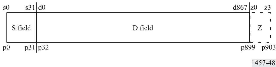
FIGURE 48 Packet P80
