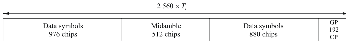
FIGURE 34 Burst structure of the burst type 3 (GP denotes the guard period and CP the chip periods)
