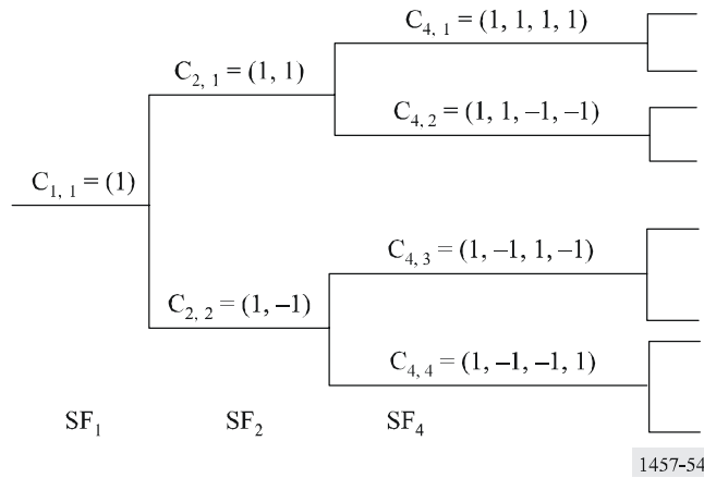
FIGURE 54 Code tree generation for OVSF codes
