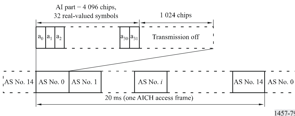
FIGURE 79 Structure of acquisition indicator channel (AICH)
