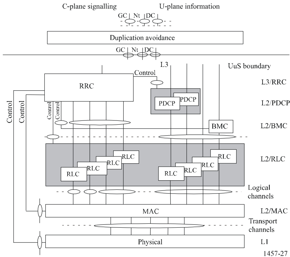
FIGURE 27 Radio interface protocol architecture of the RRC sub-layers (L2 and L1)
