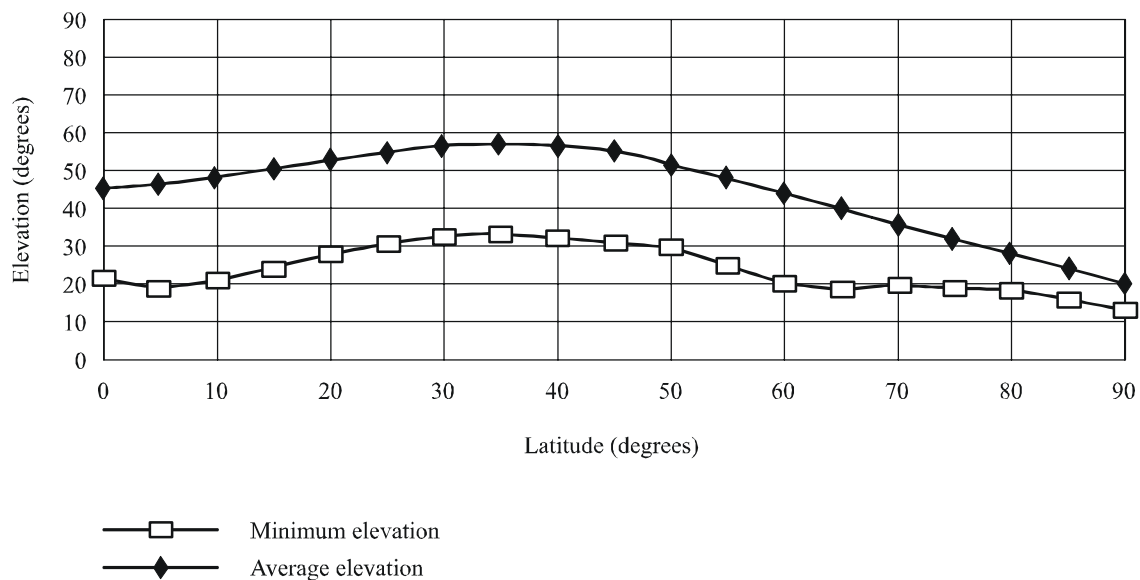
FIGURE 106 Typical minimum and average elevation angles of the nearest satellite (10 satellites)
