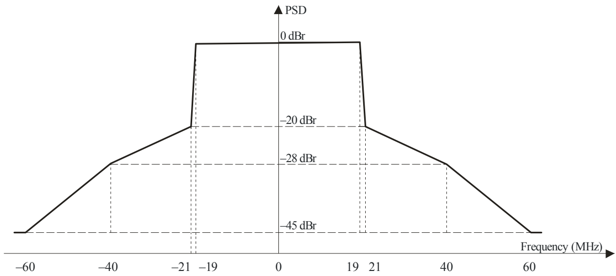
FIGURE 3 Transmit spectral mask for a 40 MHz 802.11n channel
