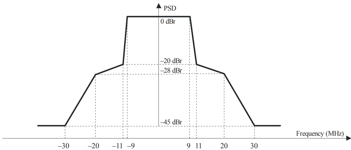
FIGURE 2 Transmit spectral mask for 20 MHz 802.11n transmission
