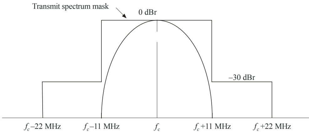
FIGURE 4 Transmit spectrum mask for 802.11b
