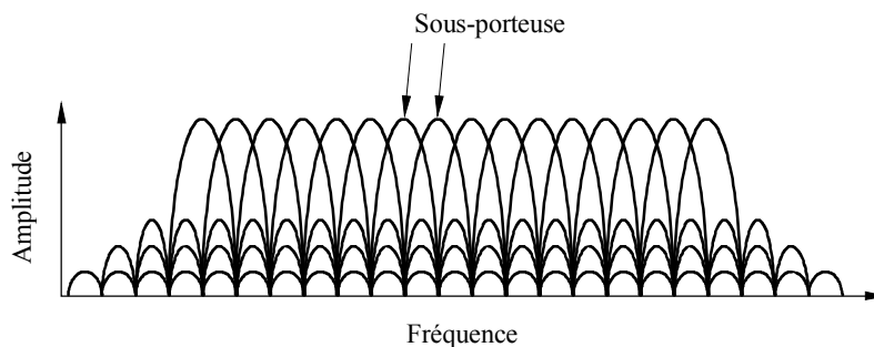
FIGURE 2 Spectre du multiplexage MRFO
