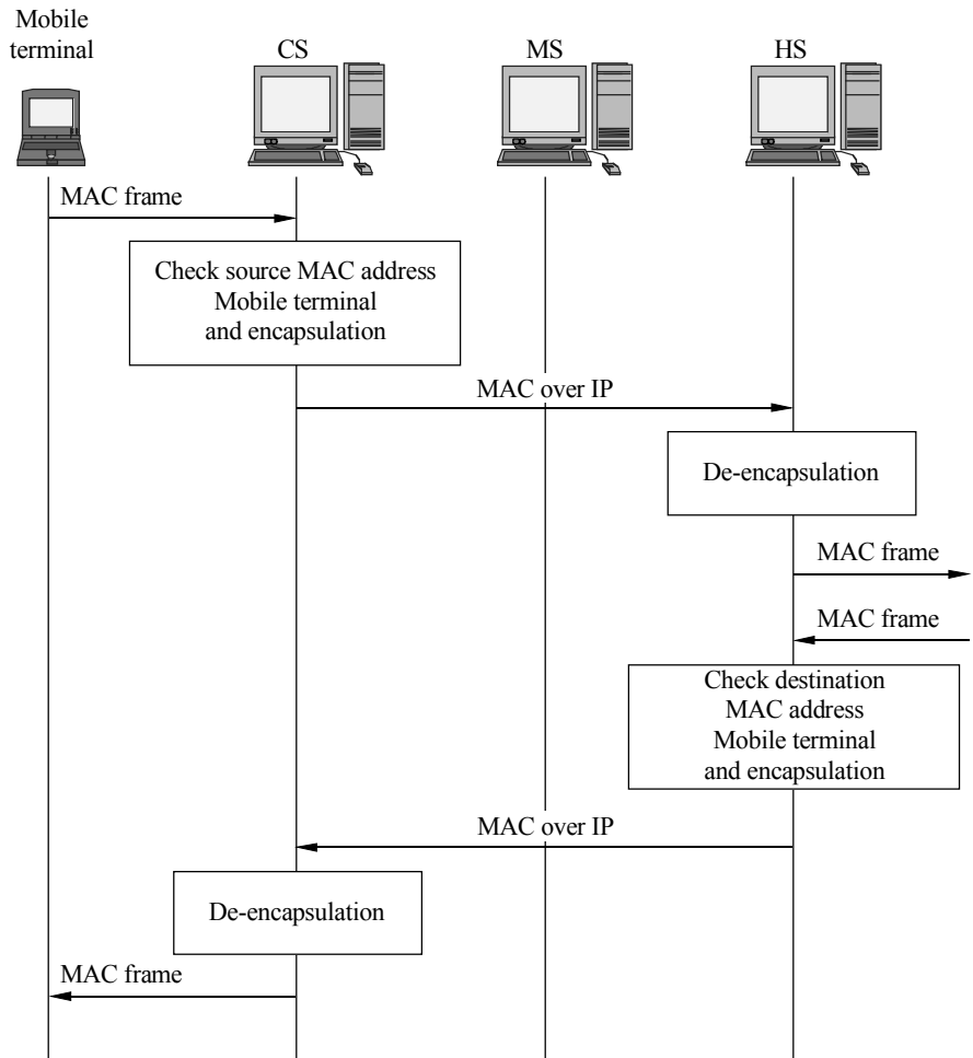
FIGURE 8 Sequence chart for encapsulation/de-encapsulation
