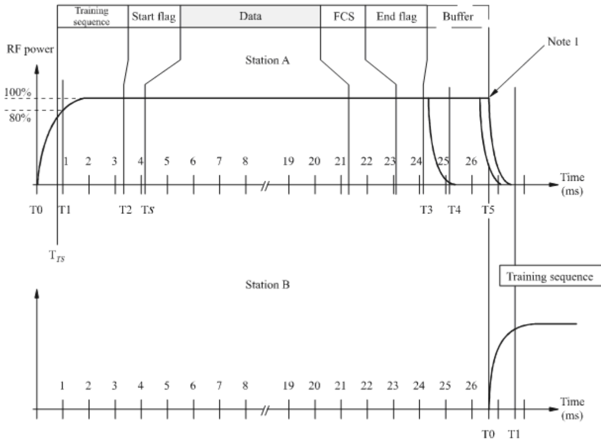
FIGURE 8 Transmission timing
