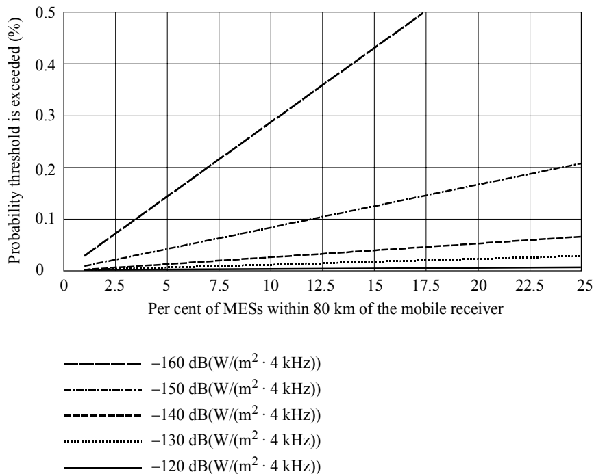
FIGURE 11 Probability that threshold is exceeded as a function of the percentage of the MSS users population within 80 km of the mobile receiver
