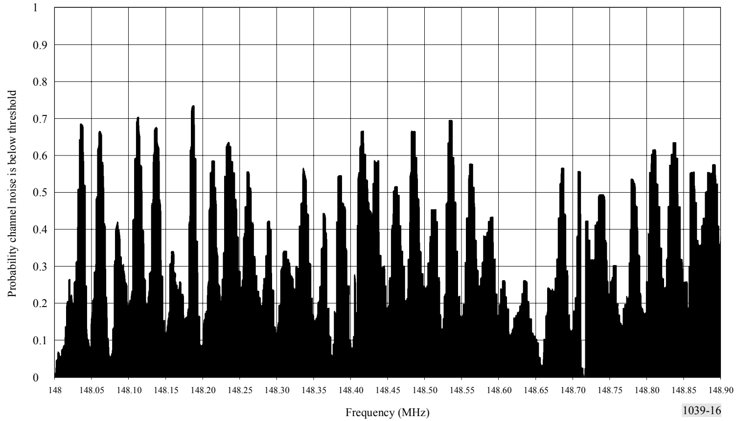
FIGURE 16 Probability of interference-free channels
