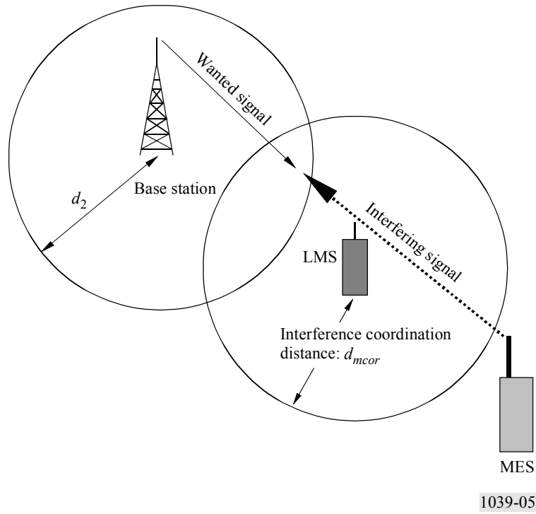
FIGURE 5 Interference coordination distance for LMS in the communications mode
