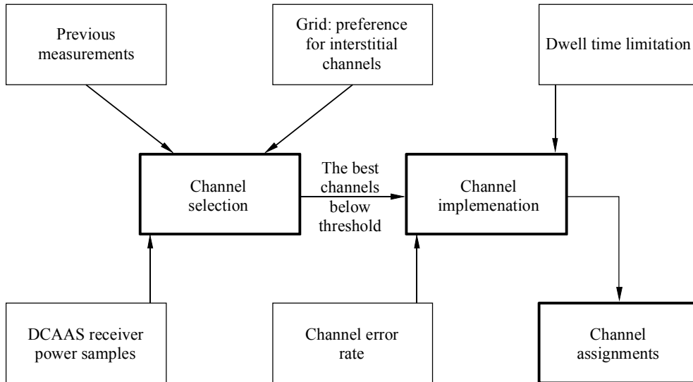
FIGURE 14 DCAAS operation
