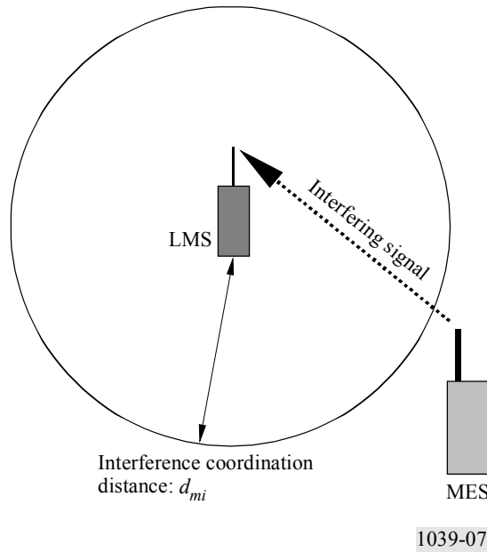
FIGURE 7 Interference coordination distance for LMS in the waiting mode
