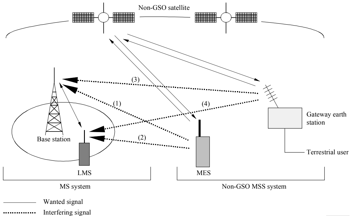
FIGURE 1 Interference model between non-GSO MSS and MS systems
