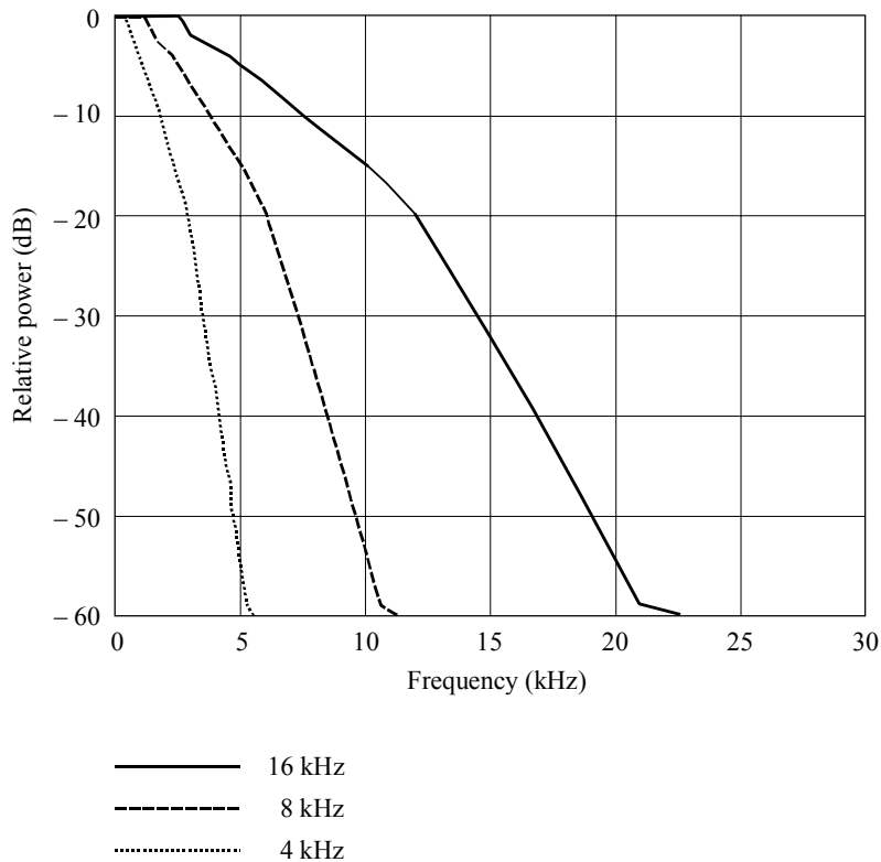
Mobile service station transmit signal masks
