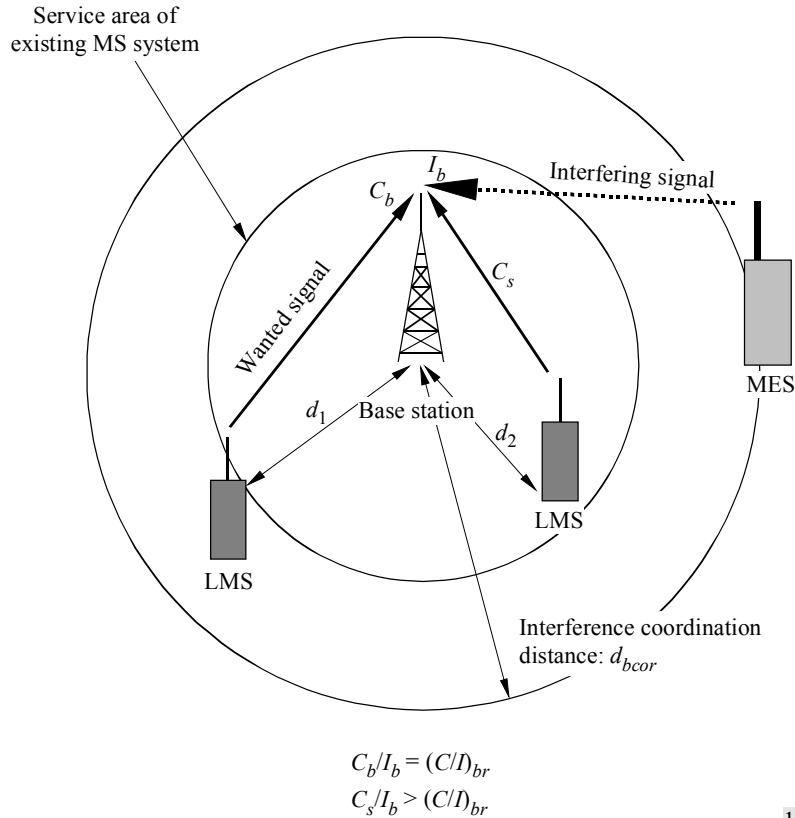
FIGURE 4 Interference coordination distance for base station in the communications mode
