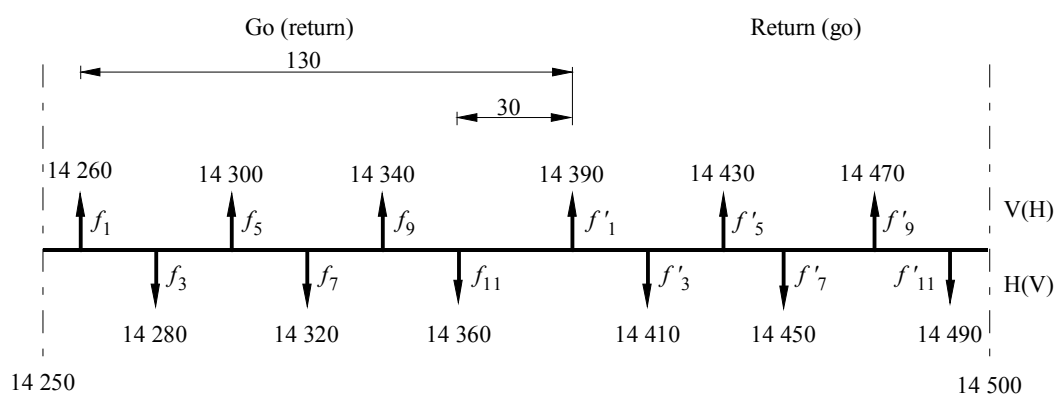
FIGURE 5 Radio-frequency channel arrangement for FWSs operating in the 14 GHz band with 20 MHz spacing (All frequencies in MHz)
