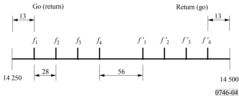
FIGURE 4 Radio-frequency channel arrangement in the frequency band 14.25-14.5 GHz (All frequencies in MHz)
