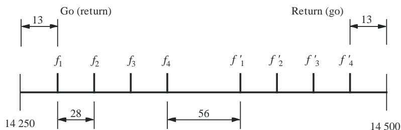
FIGURE 3 Radio-frequency channel arrangement in the frequency band 14.25-14.5 GHz (All frequencies in MHz)
