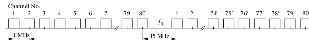
Radio-frequency channel arrangement for up to 300 telephone channel FWSs operating in the 2 300-2 500 MHz band
