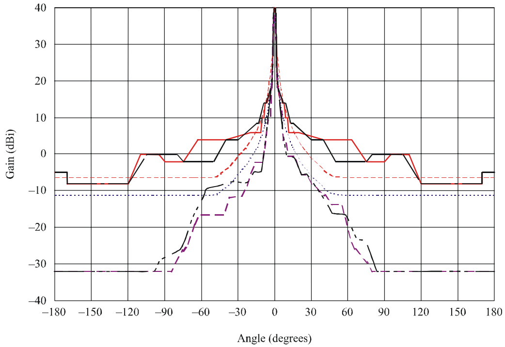
FIGURE 5 10.5 GHz P-P antenna of 1.2 m diameter ( D/\lambda = 43 ; gain = 39.9 dBi) (H: horizontal polarization, V: vertical polarization)
