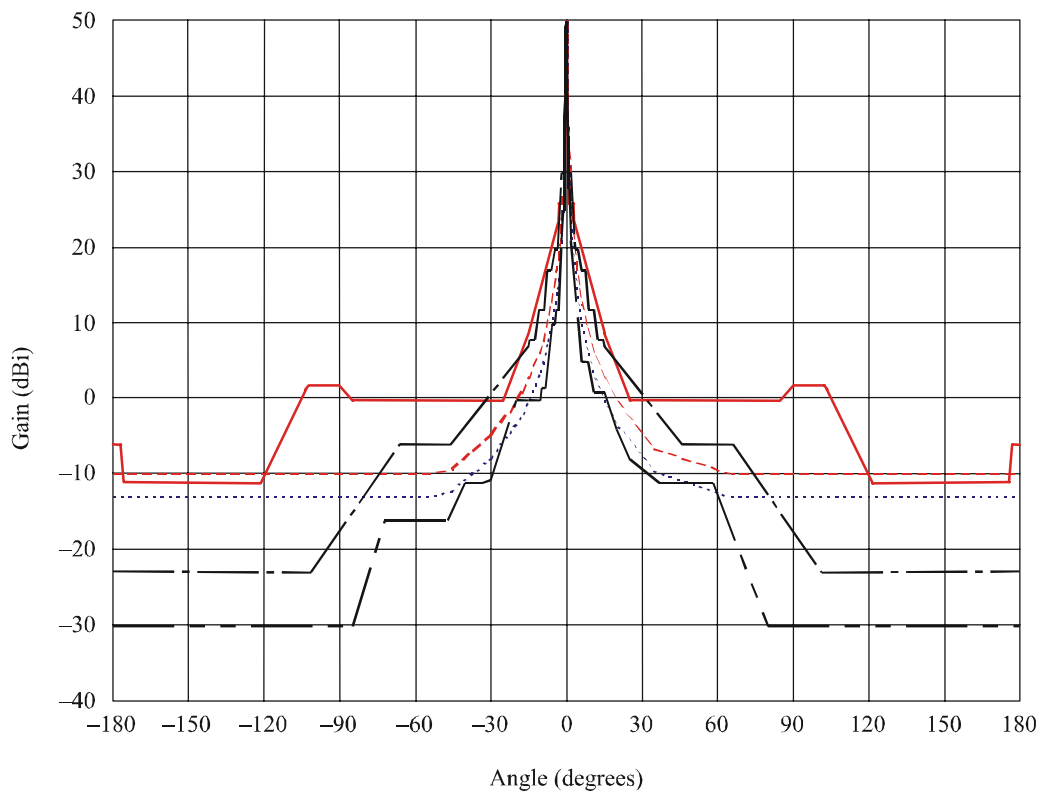
FIGURE 3 10.7 GHz point-to-point (P-P) antenna of 3 m diameter ( D/\lambda = 114 ; gain = 49.8 dBi) (H: horizontal polarization, V: vertical polarization)
