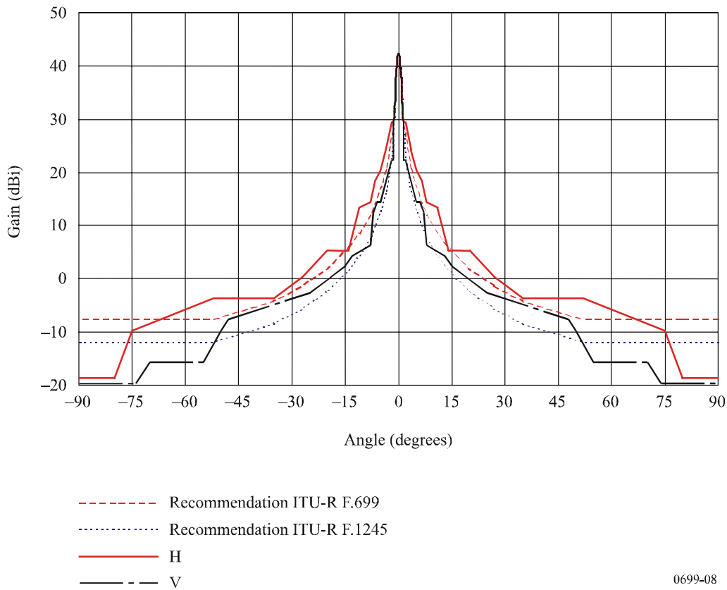
FIGURE 8 55 GHz P-P antenna of 0.3 m diameter ( D/\lambda = 57 ; gain = 42.4 dBi) (H: horizontal polarization, V: vertical polarization)
