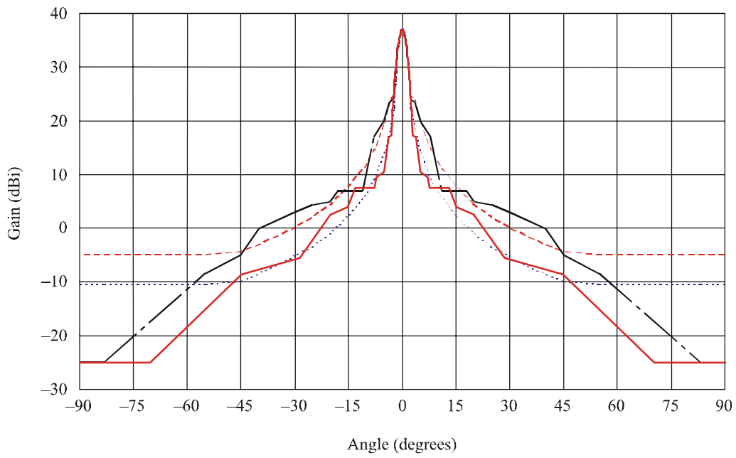
FIGURE 7 31 GHz P-P antenna of 0.3 m diameter ( D/\lambda = 32 ; gain = 36.9 dBi) (H: horizontal polarization, V: vertical polarization)
