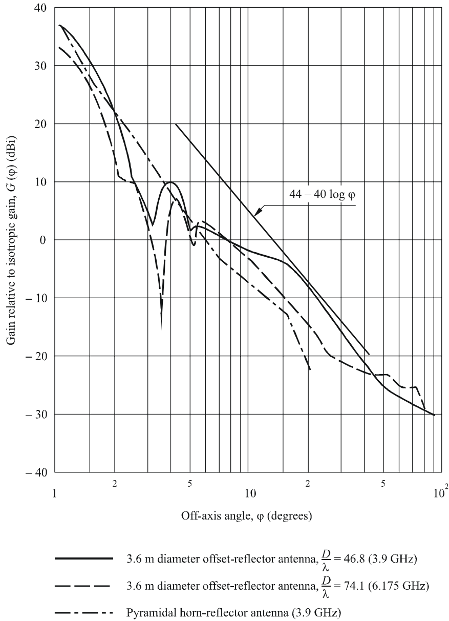
FIGURE 2 The radiation pattern of high performance antennas
