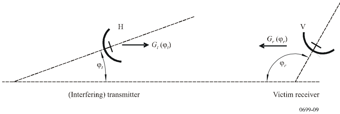
FIGURE 9 Generic example of mutual situation and orientation of transmitting antenna and victim receiving antenna
