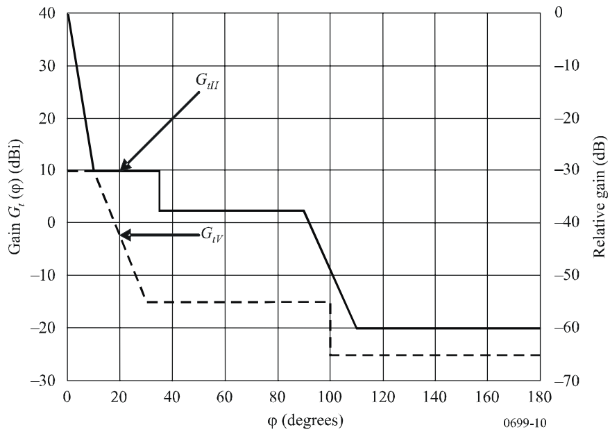
FIGURE 10 Example of transmitter antenna mask for co- and cross-polarization
