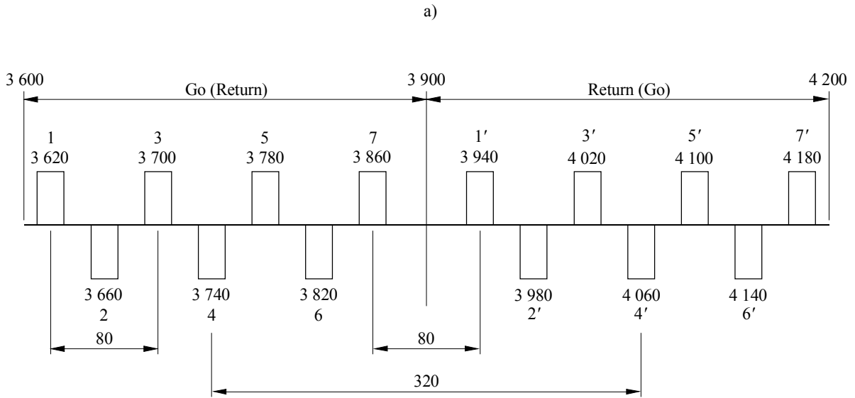
FIGURE 3 Radio-frequency channel arrangement for the 4 GHz band (All frequencies in MHz)
