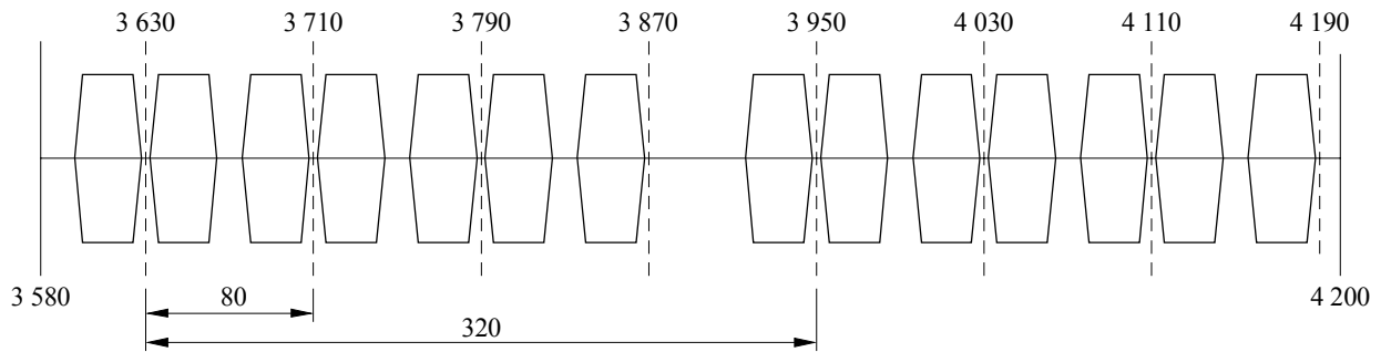
a) Channel arrangement in the band 3 580-4 200 MHz using a 2-carrier system transmitting (12 + 2) \times 155.52 Mbit/s ( 14 \times STM-1) in CCDP mode as available in Germany
