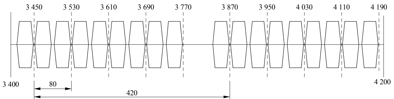
b) Possible channel arrangement in the band 3 400-4 200 MHz using a 2-carrier system transmitting (16 + 2) \times 155.52 Mbit/s ( 18 \times STM-1) in CCDP mode
