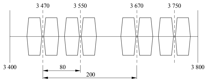
c) Channel arrangement in the band 3 400-3 800 MHz using a 2-carrier system transmitting 8 \times 155.52 Mbit/s ( 8 \times STM-1) in CCDP mode as used in Switzerland
