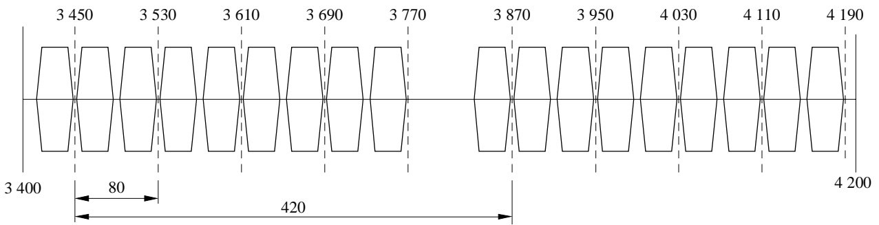
b) Possible channel arrangement in the band 3 400-4 200 MHz using a 2-carrier system transmitting (16 + 2) \times 155.52 Mbit/s ( 18 \times STM-1) in CCDP mode
