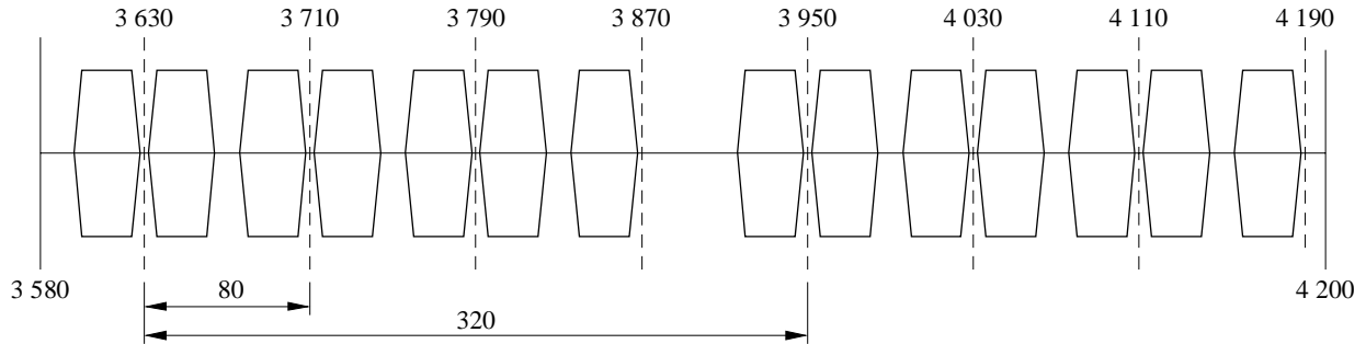
a) Channel arrangement in the band 3 580-4 200 MHz using a 2-carrier system transmitting (12 + 2) \times 155.52 Mbit/s ( 14 \times STM-1) in CCDP mode as available in Germany
