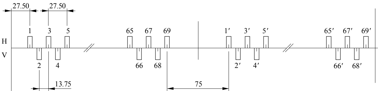
FIGURE 7b Radio-frequency channel arrangement for medium capacity radio-relay systems with 27.5 MHz channel spacing in interleaved channel arrangement (All frequencies in MHz)
