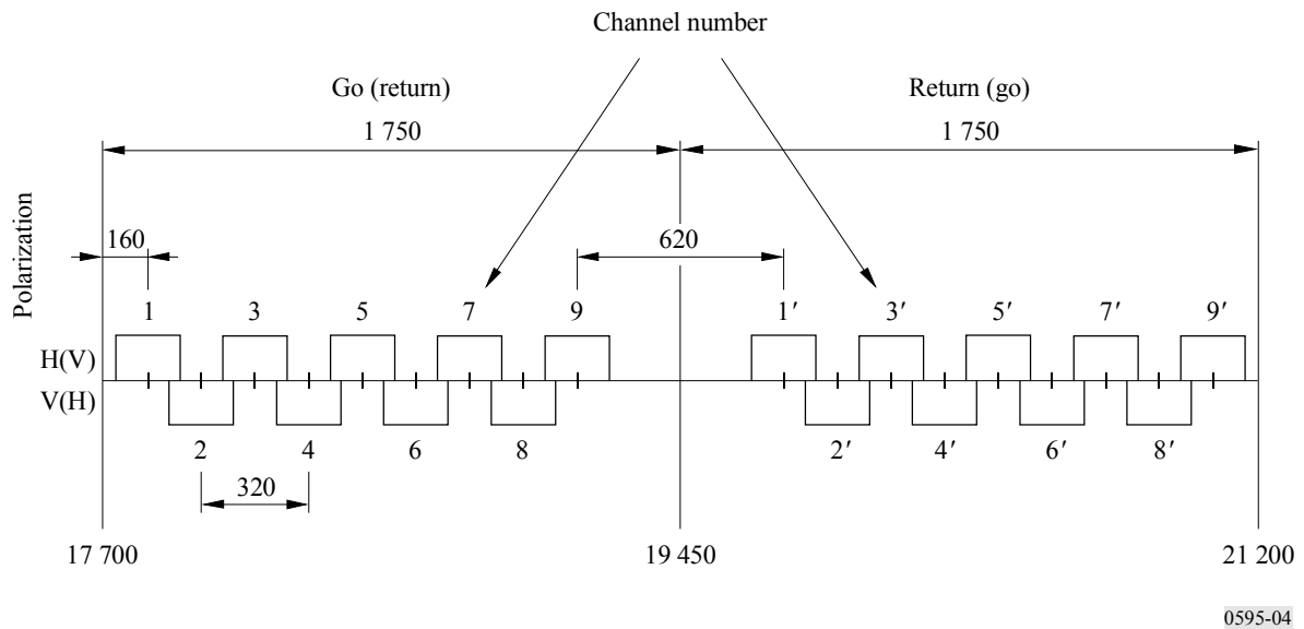
FIGURE 4 Radio-frequency channel arrangements for digital radio-relay systems operating in the 17.7 to 21.2 GHz band (Japan) (All frequencies in MHz)
