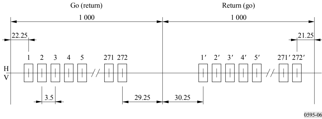
FIGURE 6 Radio-frequency channel arrangement for low capacity radio-relay systems operating in the 18 GHz band (United Kingdom) (All frequencies in MHz)
