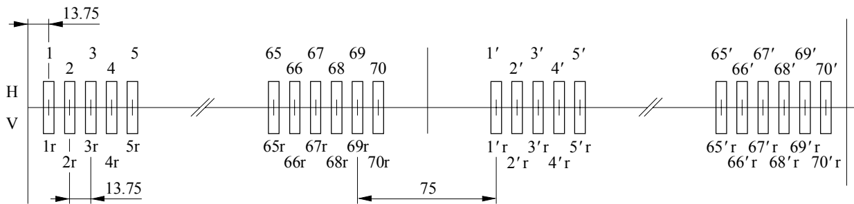
FIGURE 7a Radio-frequency channel arrangement for medium capacity radio-relay systems with 13.75 MHz channel spacing in co-channel arrangement (All frequencies in MHz)
