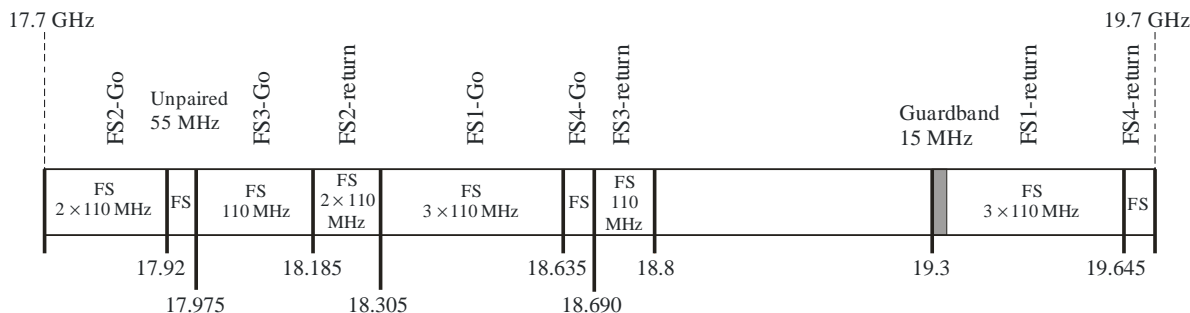
Channelization plan for the 17.7-19.7 GHz band of Annex 6
