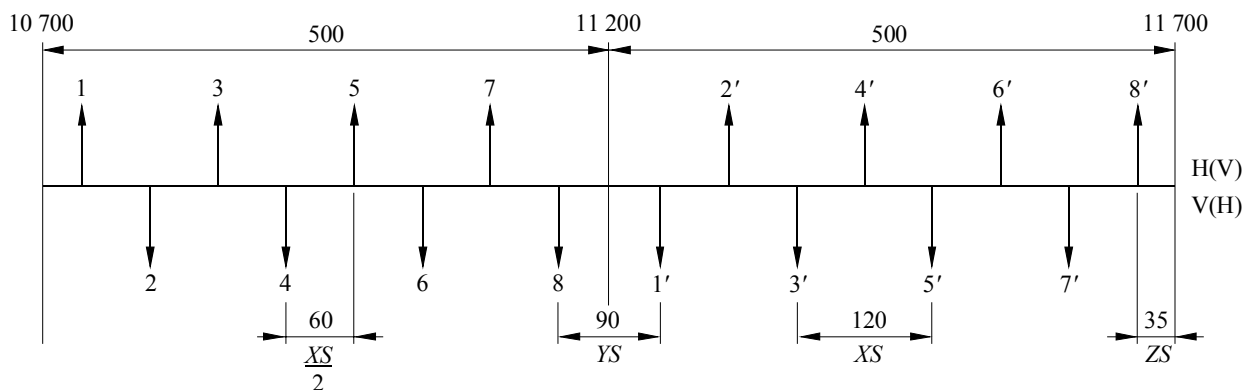
Radio-frequency channel arrangement for a 140 Mbit/s radio-relay system operating in the 10.7-11.7 GHz band (All frequencies in MHz)
