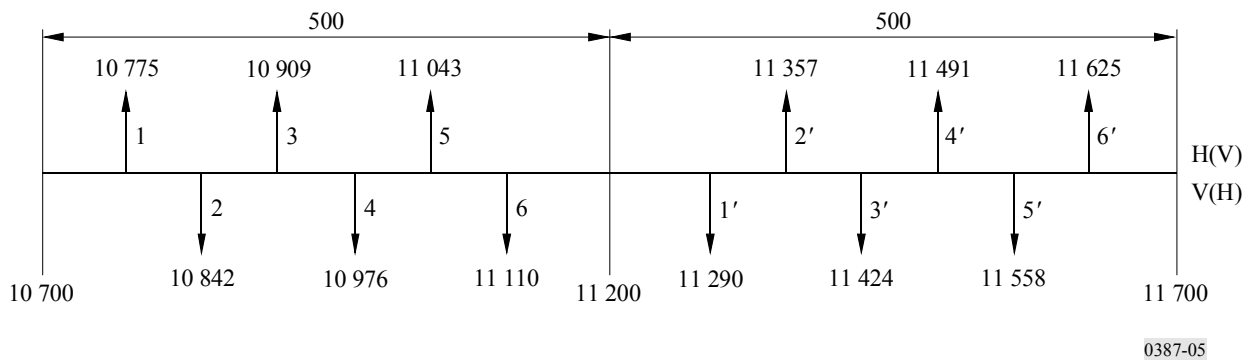
Radio-frequency channel arrangement for a 4-PSK digital radio-relay system (All frequencies in MHz)
