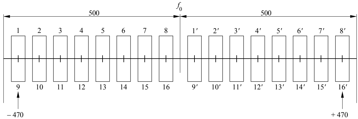
FIGURE 8 Radio-frequency channel arrangement for high capacity digital radio-relay systems operating in the 11 GHz band (All frequencies in MHz)
