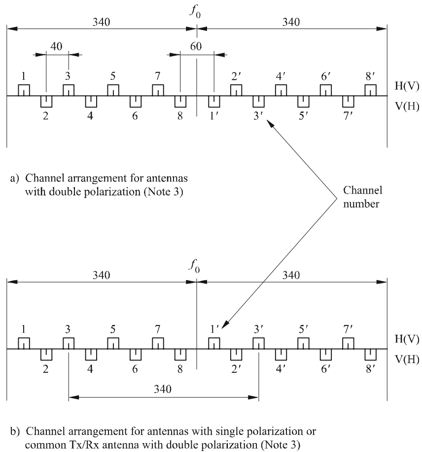
FIGURE 1 Channel arrangement for antennas with single and double polarizations (All frequencies in MHz)
