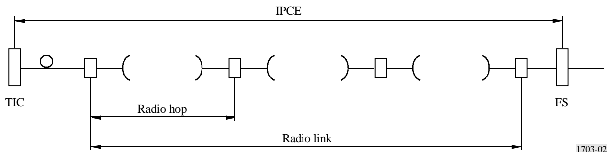
FIGURE 3 Example of a radio link implementing a portion of IPCE
