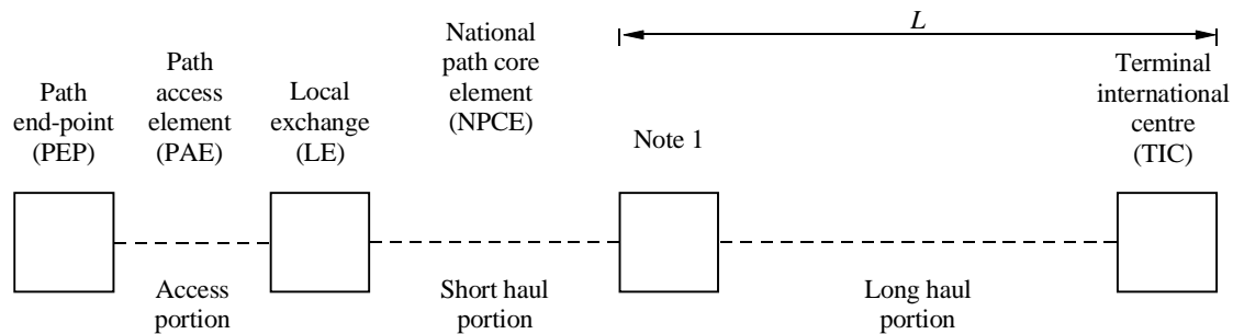
FIGURE 1 Basic sections of the national portion of the HRP
