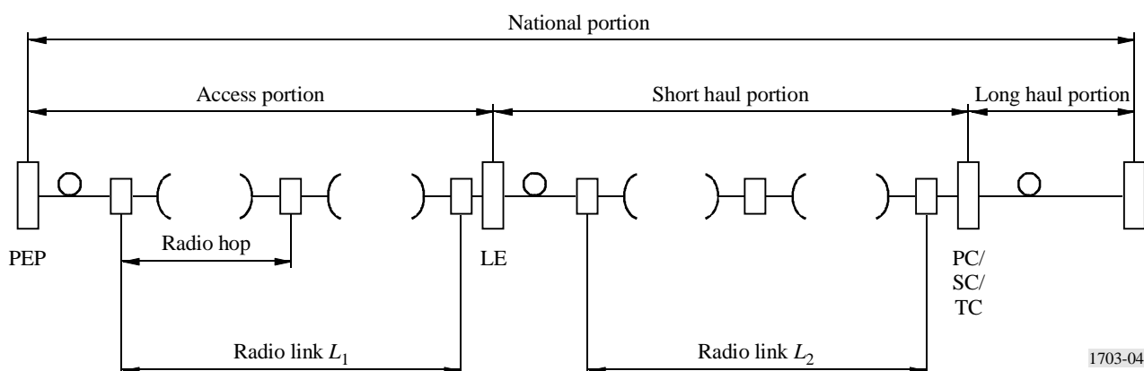
FIGURE 4 Example of radio links used in access portion and short haul portion of NPE
