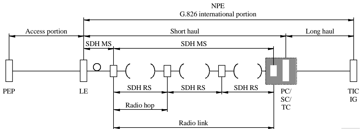
FIGURE 6 Example of a radio link implementing a portion of the NPE
