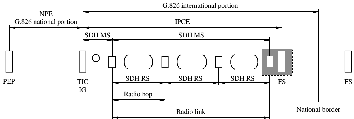
FIGURE 5 Example of a radio link implementing a portion of the IPCE
