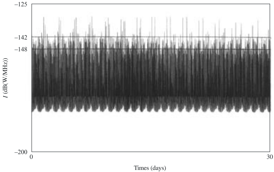
Interference into 41° W DRS while tracking the international space station
