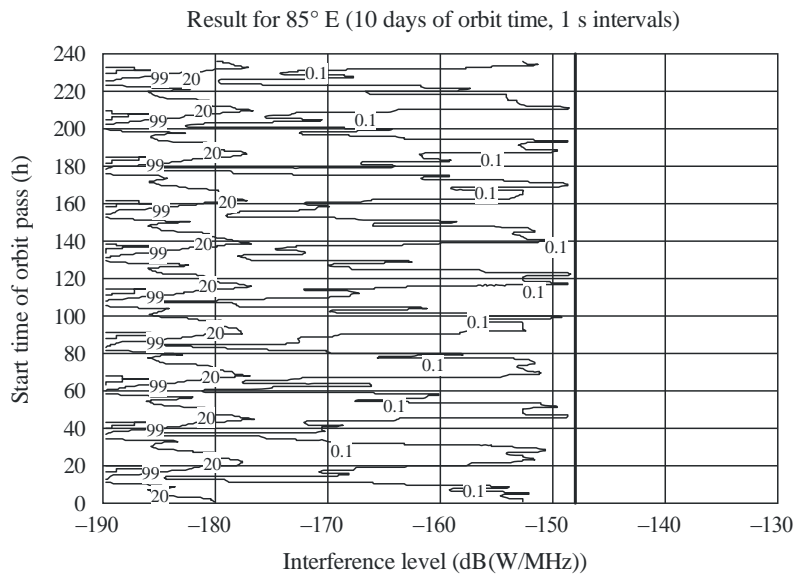
FIGURE 9 Temporal characteristics of the interference to a DRS located at 85° E while tracking a low-orbiting user satellite in an international space station type orbit
