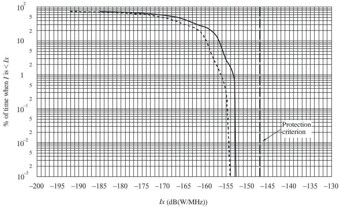
FIGURE 17 Cumulative interference into an international space station POCS over 30 days
