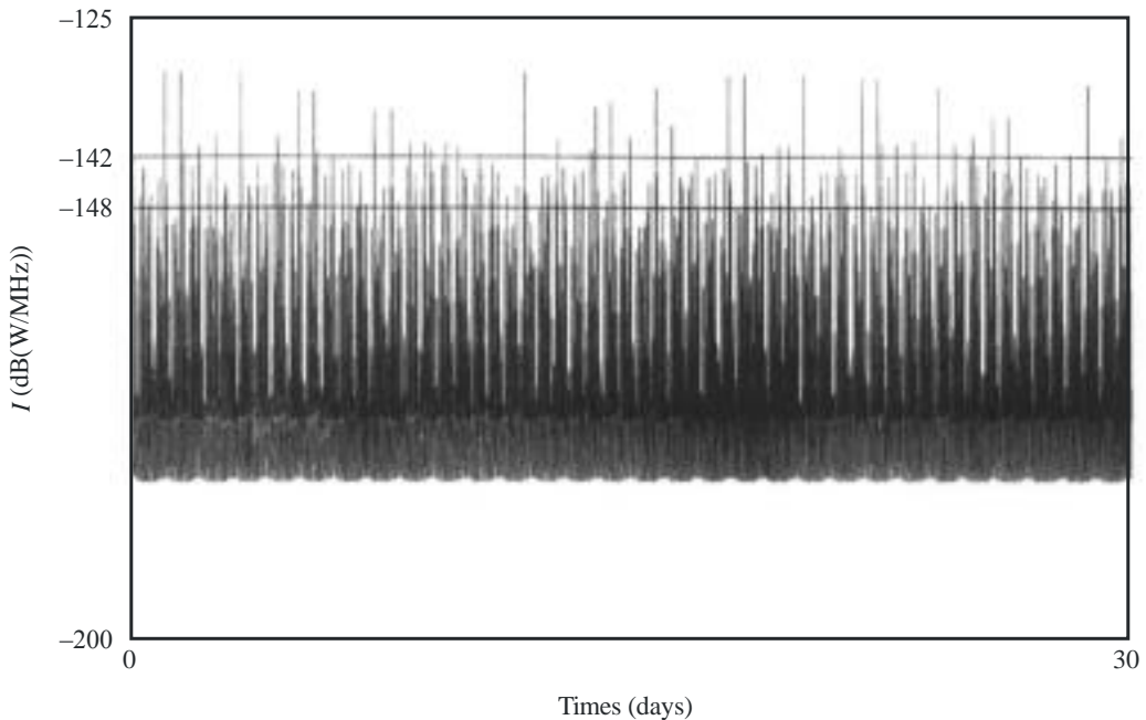
Interference into 41° W DRS while tracking the EOS
