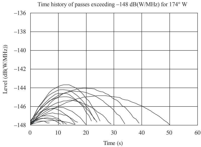
FIGURE 8 Examples interference to a DRS located at 174° W while tracking a low-orbiting user satellite in an international space station type orbit (see § 3.2)
