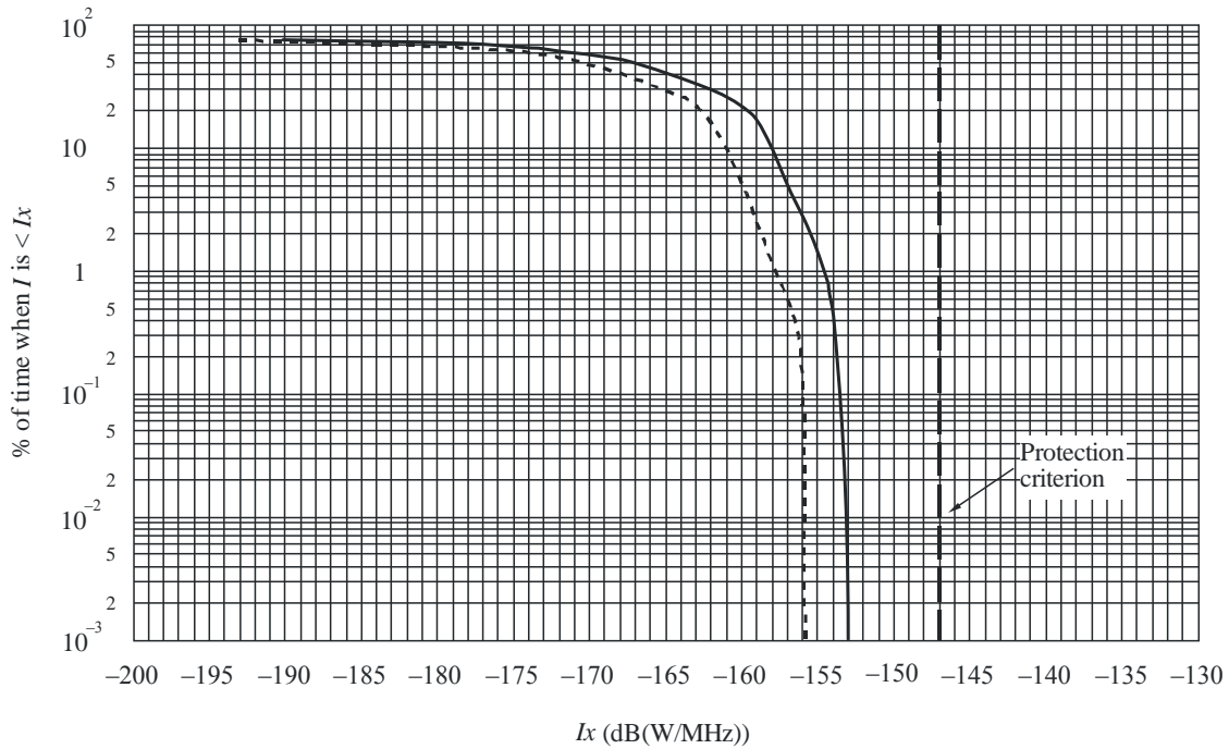
FIGURE 18 Cumulative interference into a space shuttle orbiter POCS over 30 days
