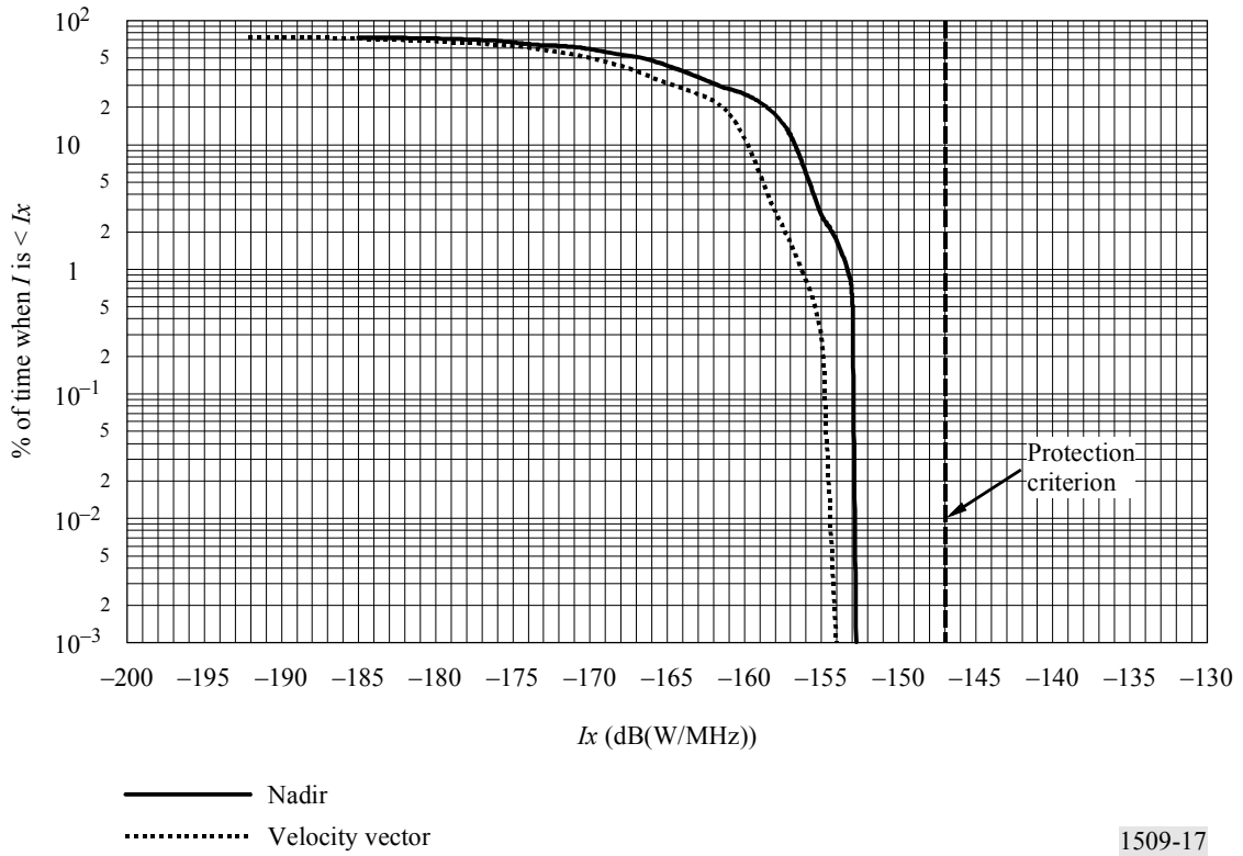
FIGURE 17 Cumulative interference into an international space station POCS over 30 days
