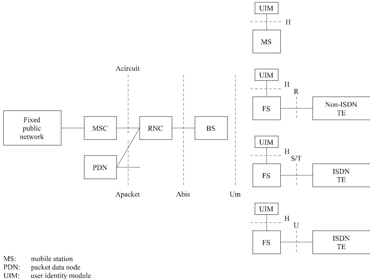
FIGURE 1 A reference model of the FWA supported from a mobile network
