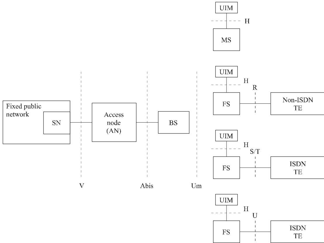
FIGURE 2 A reference model of the FWA supported from a PSTN access network
