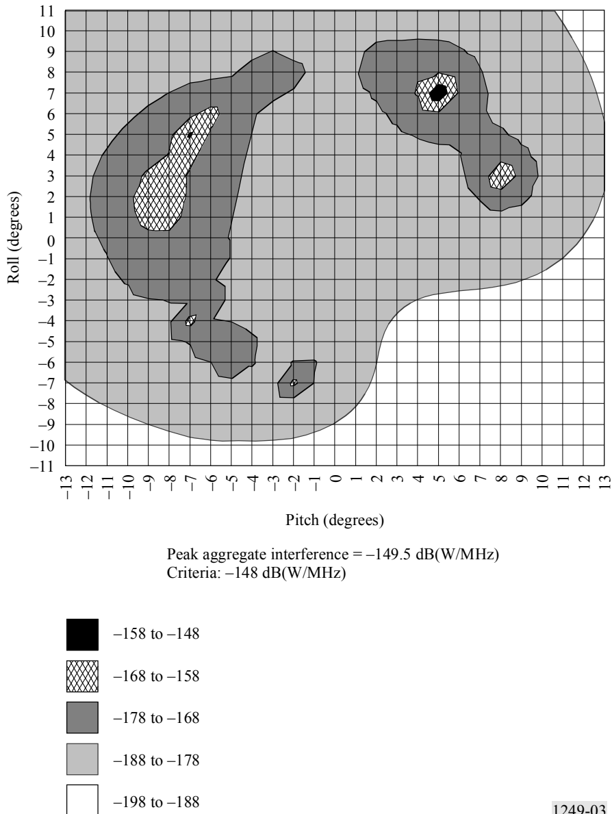
FIGURE 3 Aggregate interference (dB(W/MHz)) to DRS located at 174° W, as a function of spacecraft antenna pointing angles
