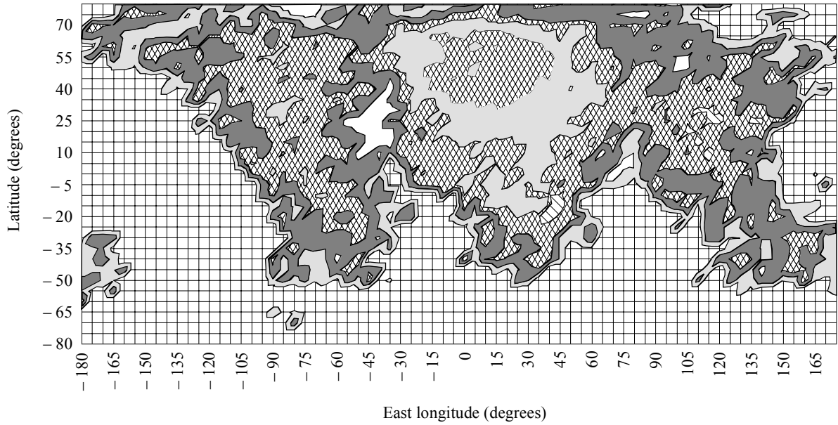
FIGURE 1 Contour plot of the geographical distribution of interference to satellites at orbital altitudes of 300 km
