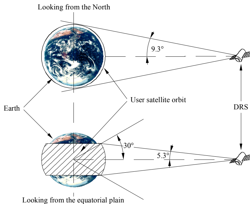
FIGURE 3 DRS service area for a user satellite in a 30° inclined orbit
