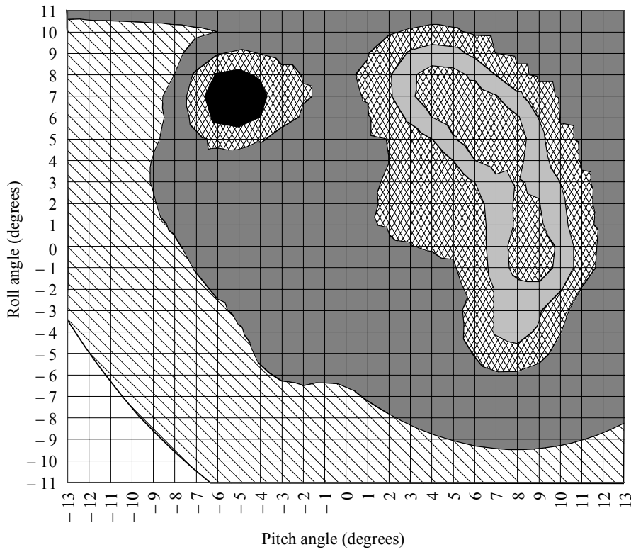
Contour plot of the interference to DRS satellite antenna as a function of the roll and pitch angle: DRS at 41° W longitude; and the SSA antenna
