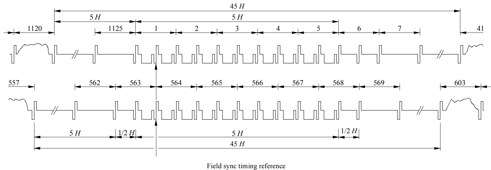
FIGURE 5 Field synchronizing signal waveform for the 1125/60/2:1 system
