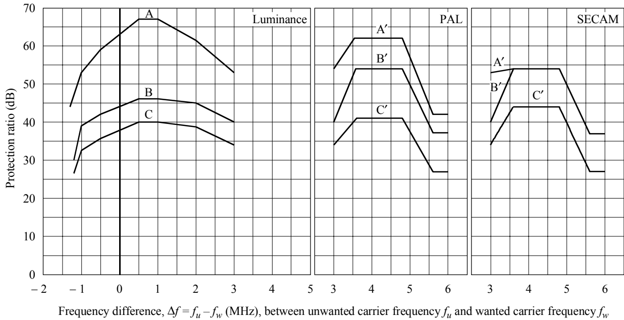
FIGURE 5 and TABLE 14 625-line systems – Limit of perceptibility (for information only)
