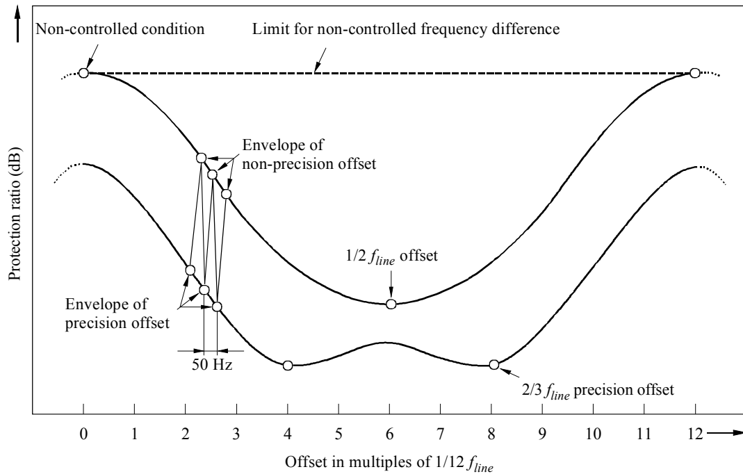
FIGURE 8 Schematic protection ratio curves with different offset positions
