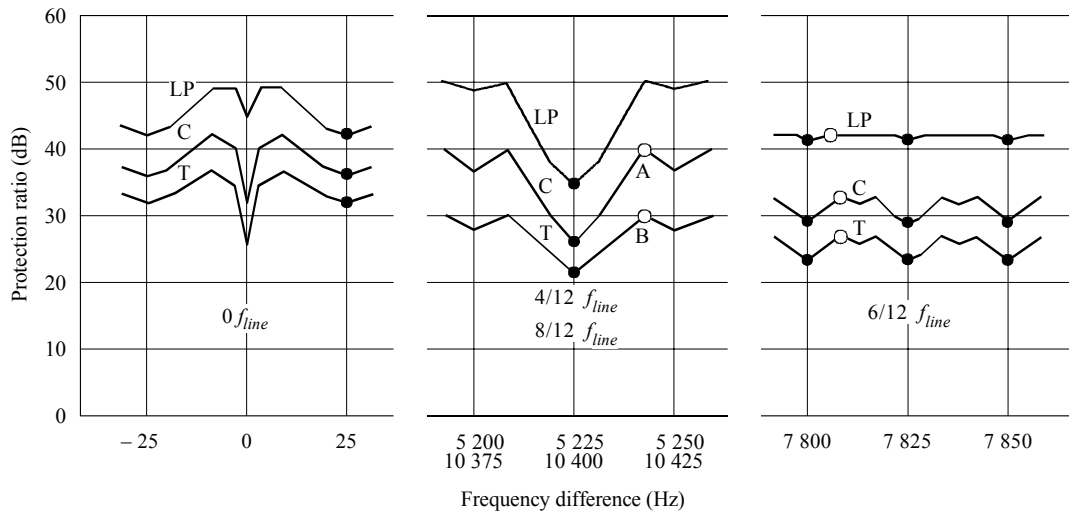
FIGURE 9 Precise structure of the protection ratio curves for different offset positions
