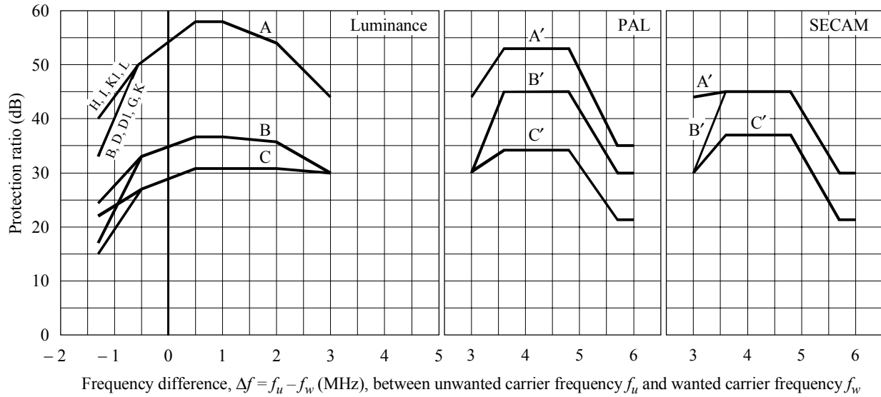
FIGURE 4 and TABLE 13 625-line systems – Continuous interference
