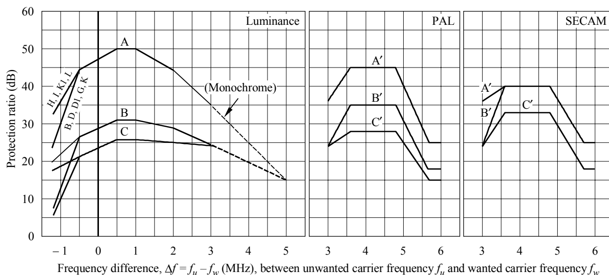
FIGURE 3 and TABLE 12 625-line systems – Tropospheric interference
