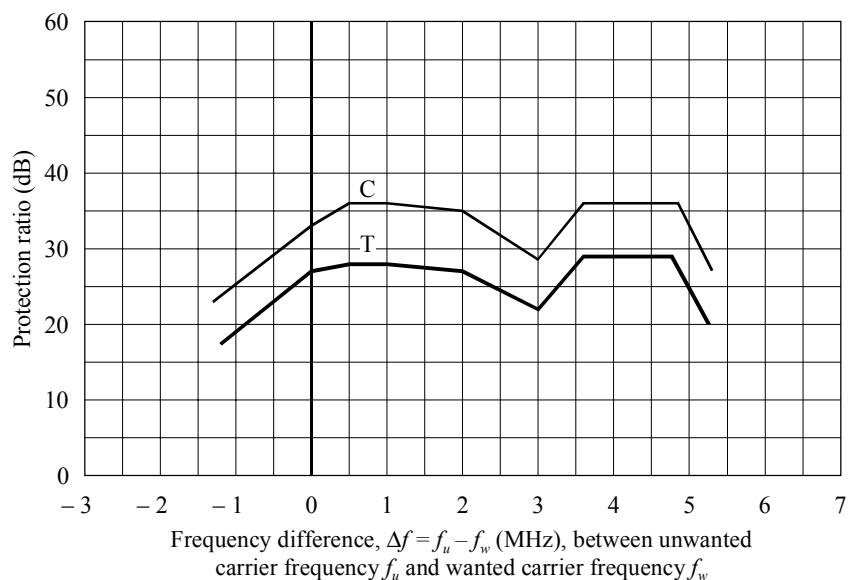
FIGURE 7 and TABLE 16 625-line systems – B/PAL and G/PAL – Protection from full-field data signals
