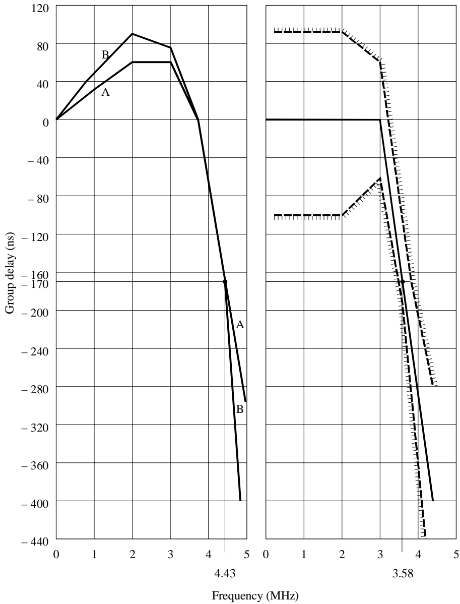
FIGURE 3 Curve of pre-correction for receiver group-delay characteristics
