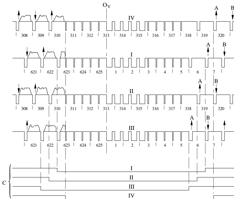
FIGURE 5a Burst-blanking sequence in the B, B1, D, G, H, K and I/PAL systems
