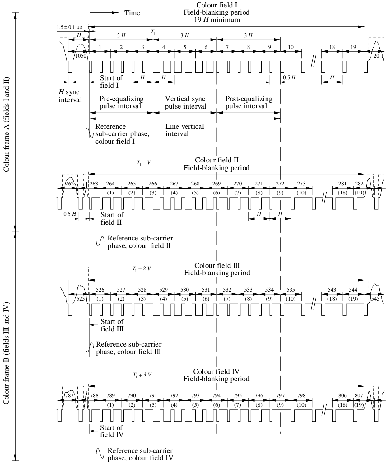
FIGURE 5c Burst-blanking sequence in M/NTSC system
