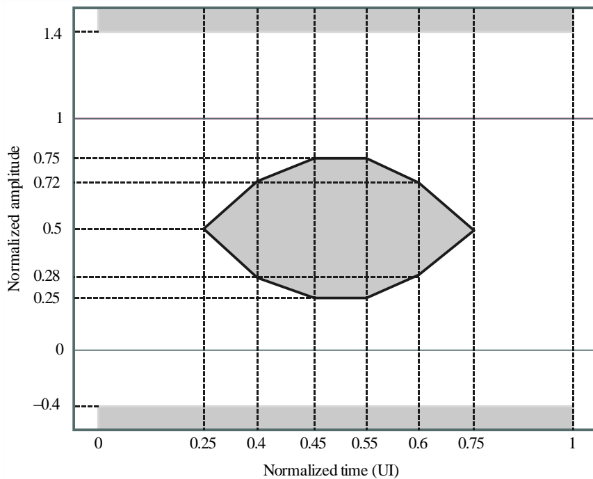
Transmitter output optical eye mask
