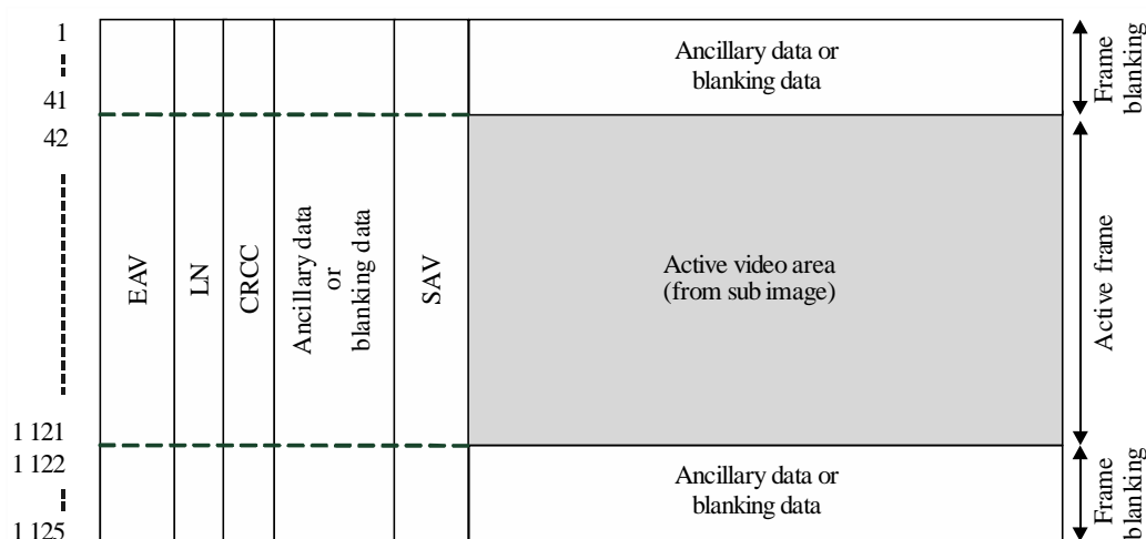
Frame structure of data stream
