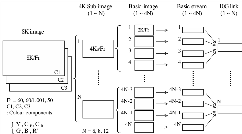
Mapping overview of 8K images with 60 Hz, 60/1.001 Hz or 50 Hz frame frequency
