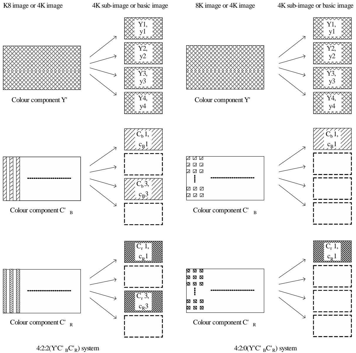
Image division of 4:2:2 (Y'C'B'C'R) and 4:2:0 (Y'C'B'C'R) systems
