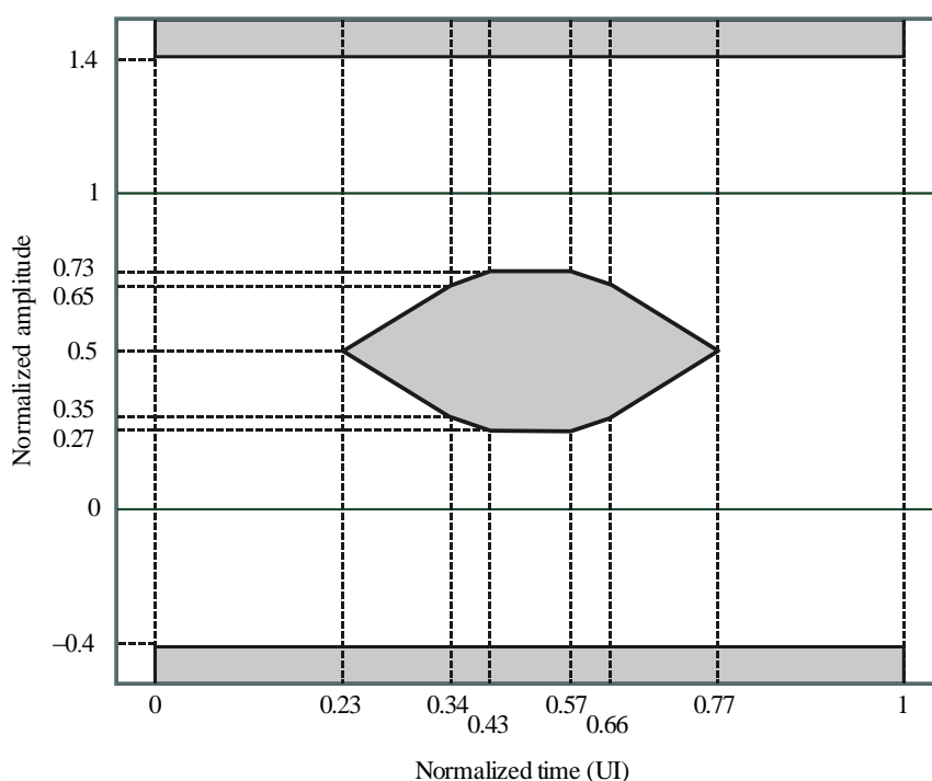
Transmitter output optical eye mask
