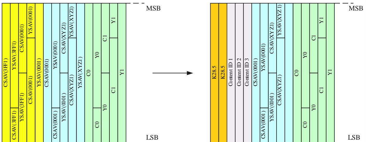
FIGURE 1-B4 SAV data replacement for CH1 data
