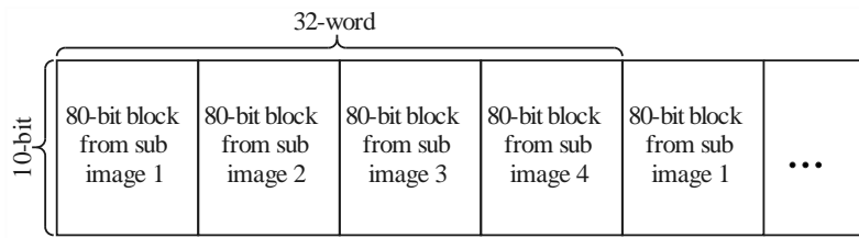
FIGURE 1-B12 80-bit array interleaving derived from basic stream pair
