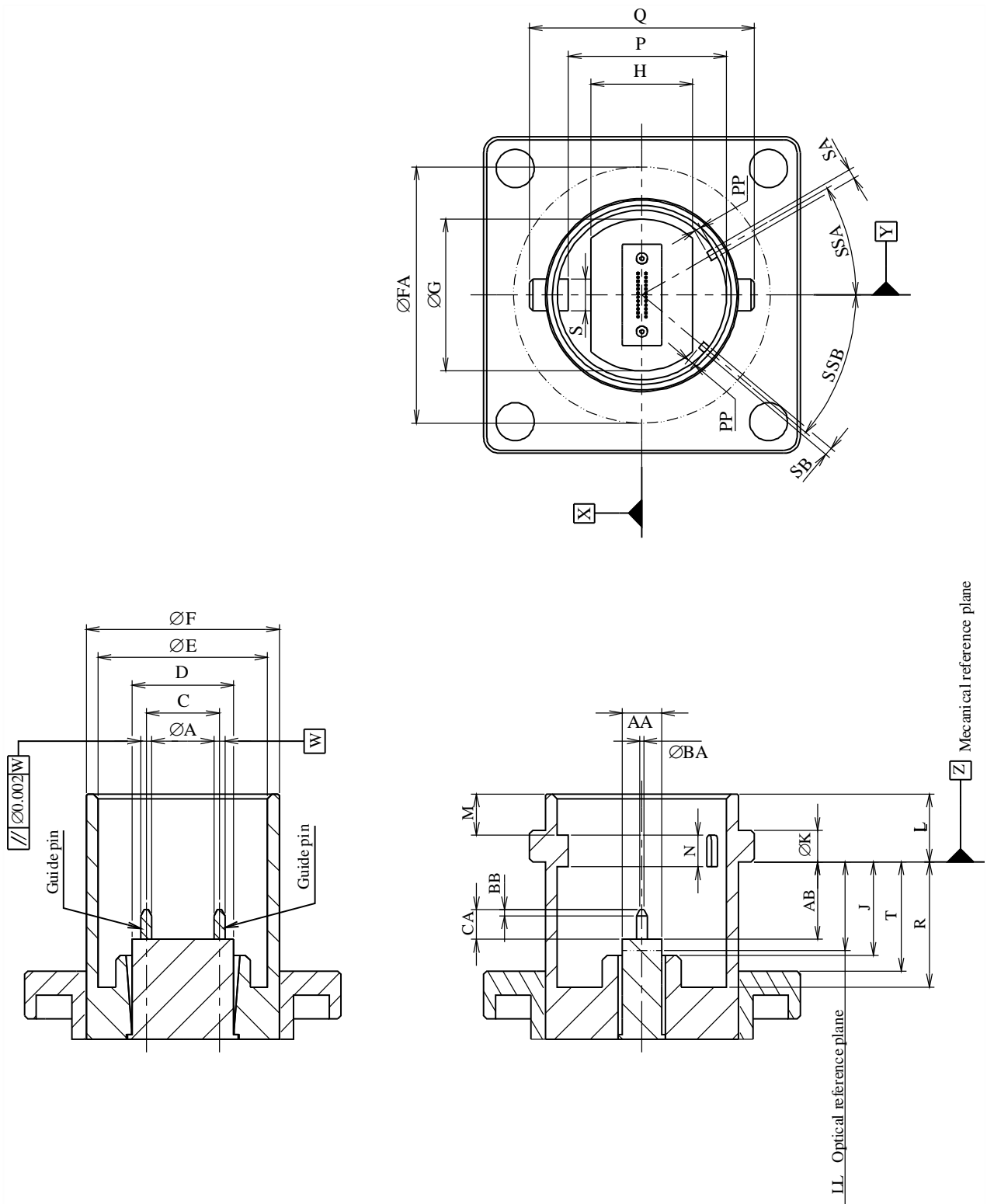
FIGURE 2-29 Receptacle connector with equipment
