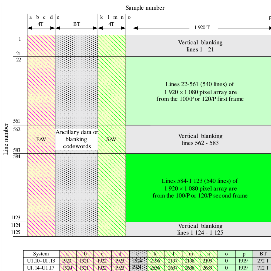
Image mapping structure and digital timing reference sequences of 1 920 × 1 080/50/P or 60/P images
