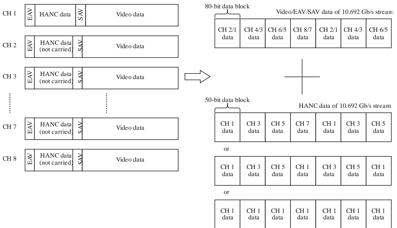
FIGURE 1-B8 Basic stream interleaving for Mode D
