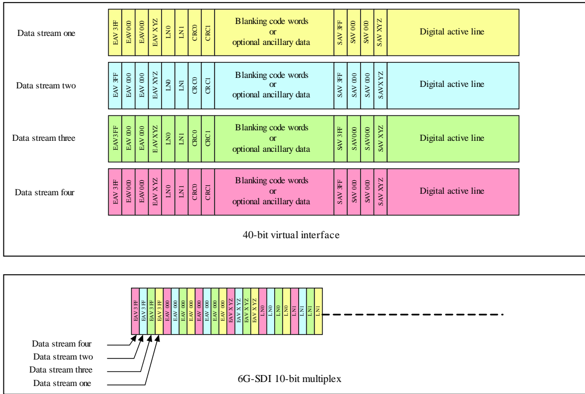
FIGURE 3-10 6G-SDI 10-bit Multiplex – Type 1
