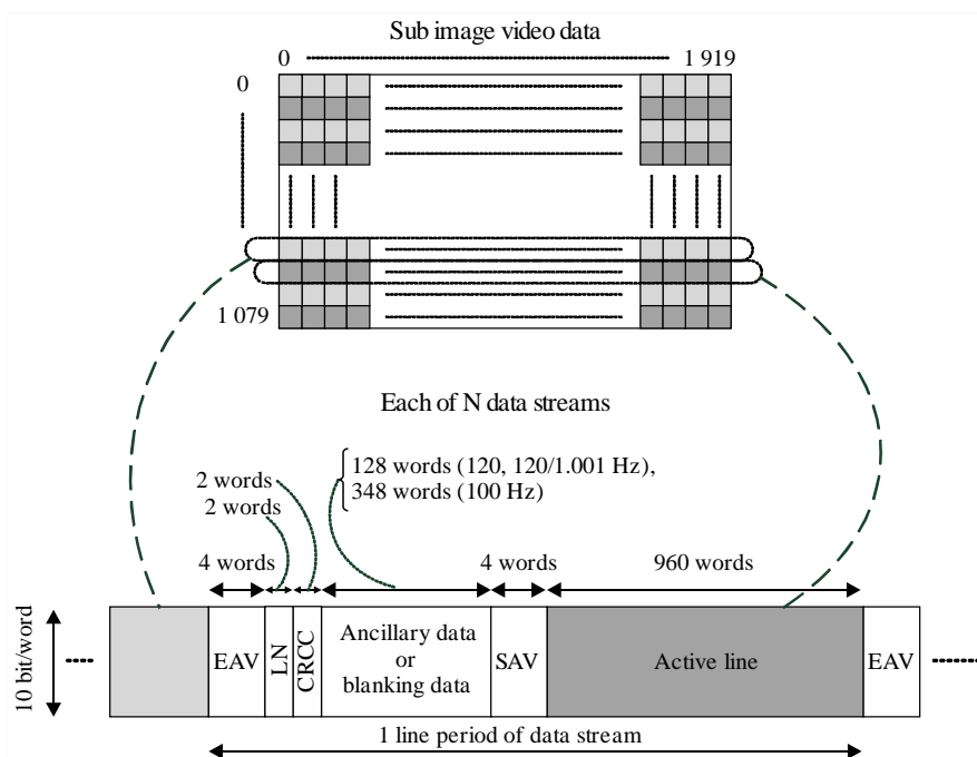
Line structure of each data stream for 120 Hz, 120/1.001 Hz or 100 Hz frame frequencies
