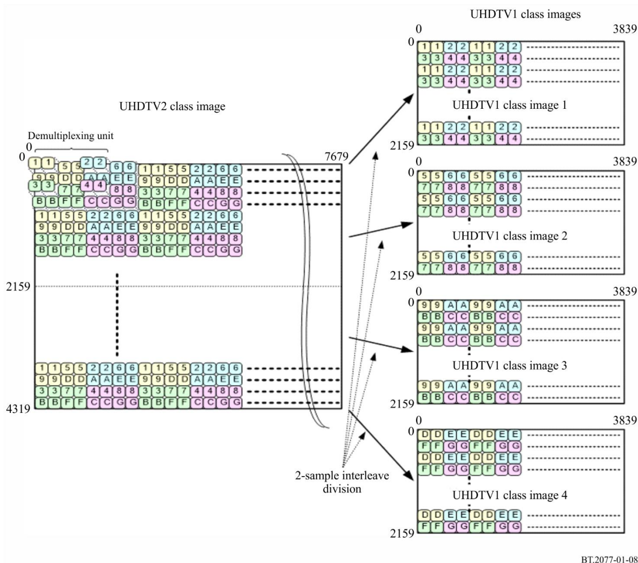
2-sample interleave division of UHDTV2 image into UHDTV1 images
