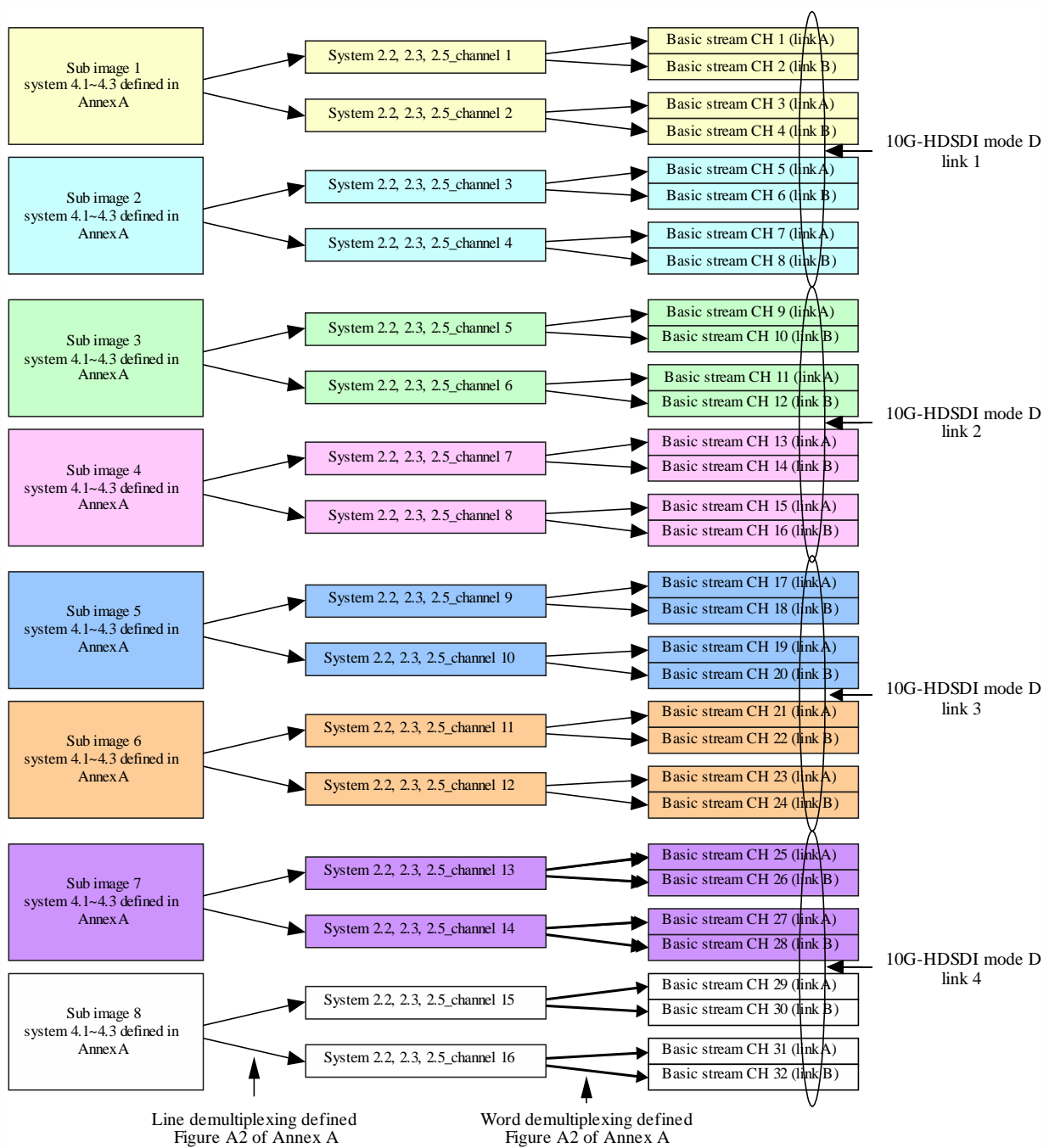
FIGURE 1-7 32 way division for Systems U1.11, U1.12 and U1.13
