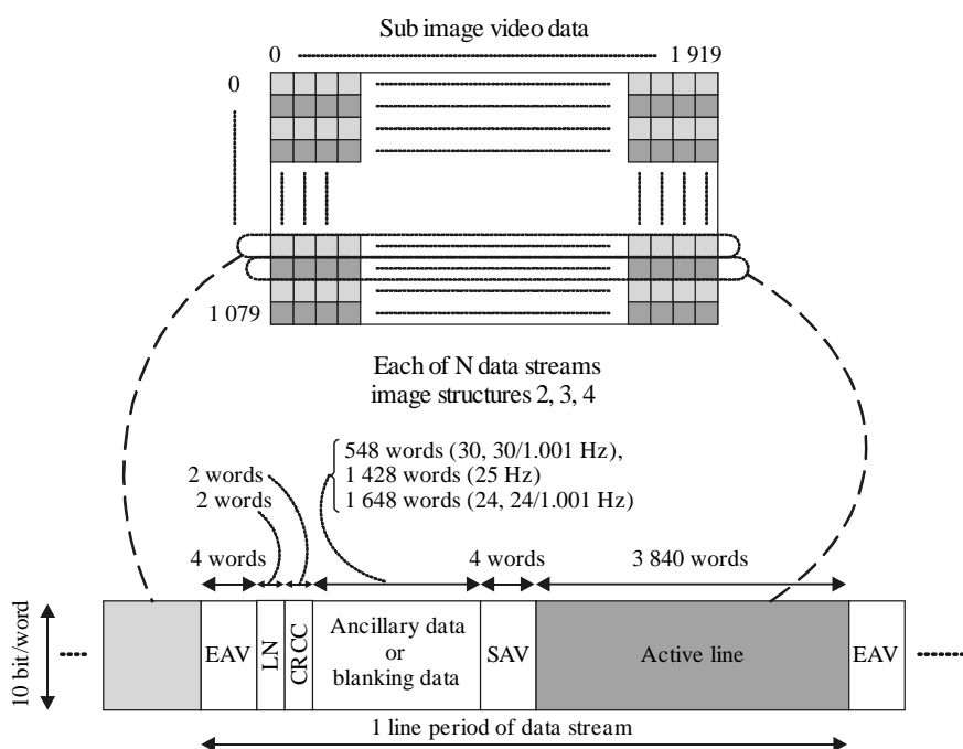
Line structure of each Data Stream for 30 Hz, 30/1.001 Hz, 25 Hz, 24 Hz and 24/1.001 Hz frame frequencies – Image Structures 2, 3 and 4
