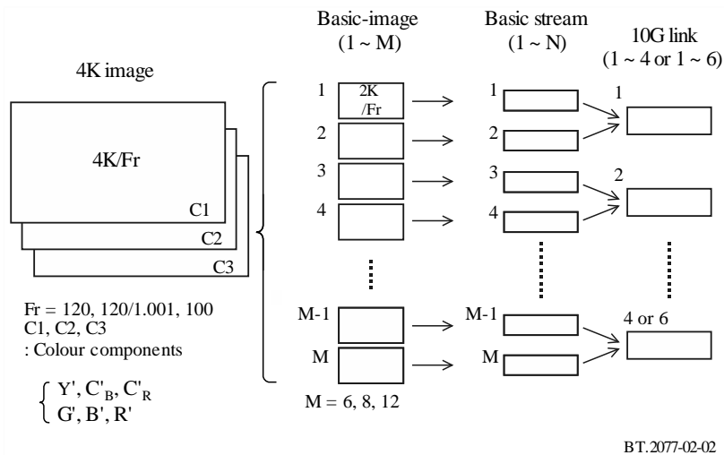
Mapping overview of 4K images with 120 Hz, 120/1.001 Hz or 100 Hz frame frequency
