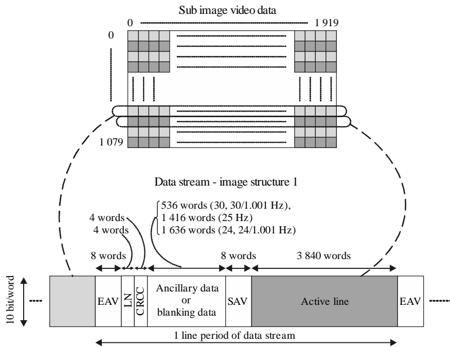
Line structure of each Data Stream for 30 Hz, 30/1.001 Hz, 25 Hz, 24 Hz and 24/1.001 Hz frame frequencies – Image Structure 1
