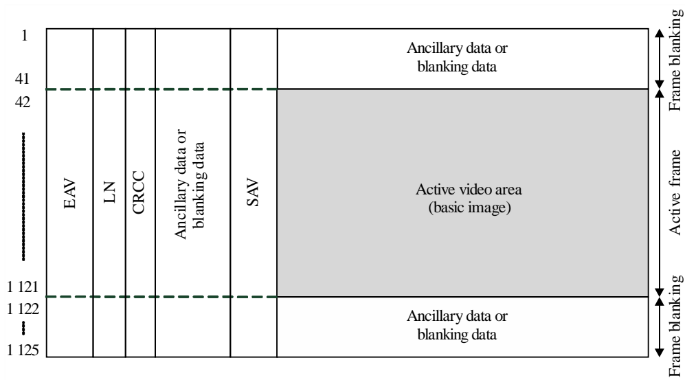
Frame structure of basic stream
