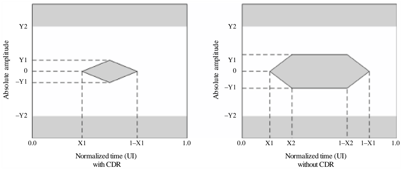
FIGURE 1-C2 Transmitter differential input electrical eye mask
