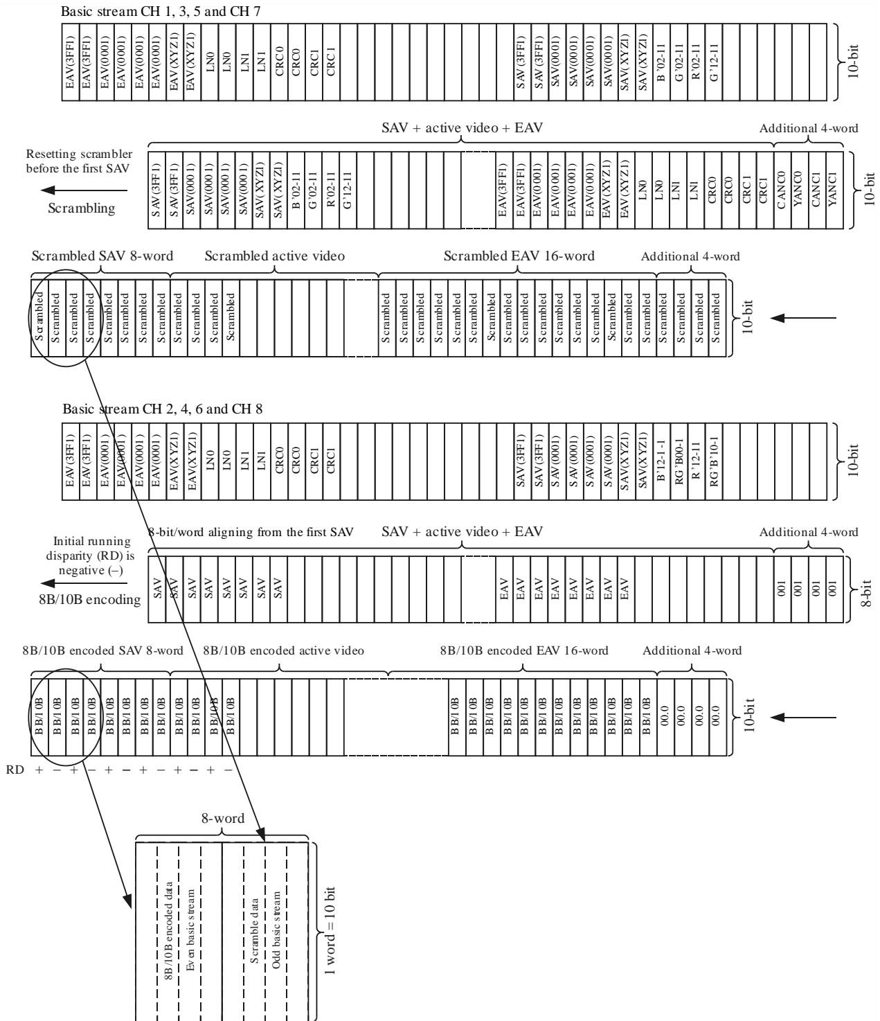
FIGURE 1-B9 80-bit blocking in Mode D
