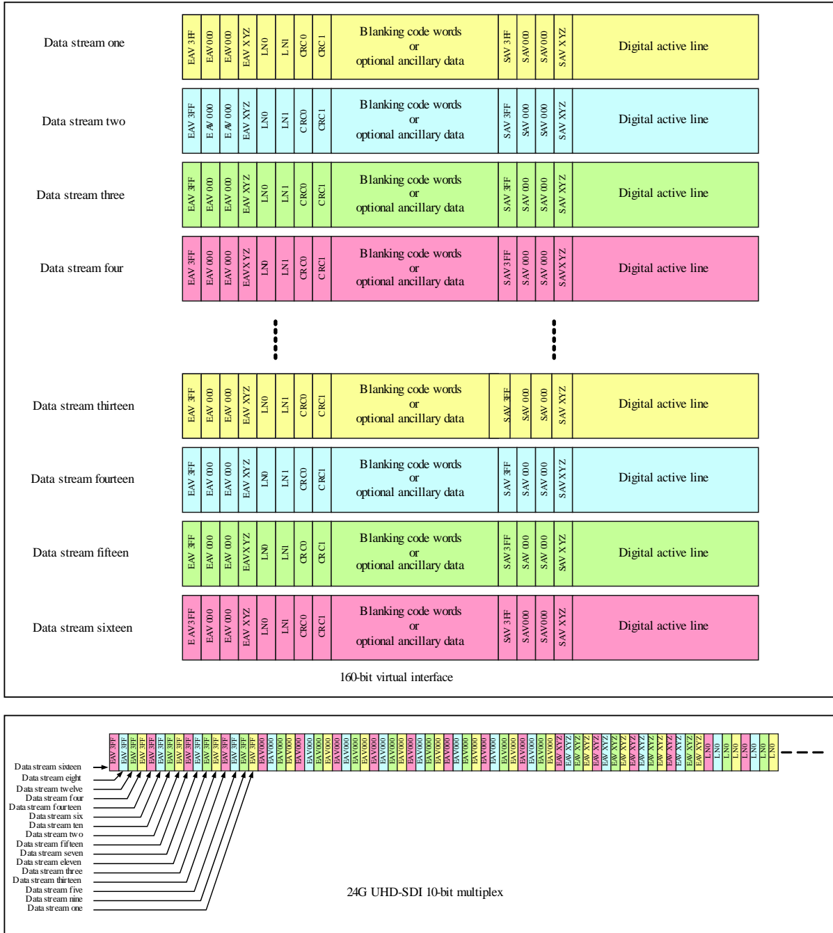
FIGURE 3-16 24G-SDI 10-bit Multiplex – Type 1
