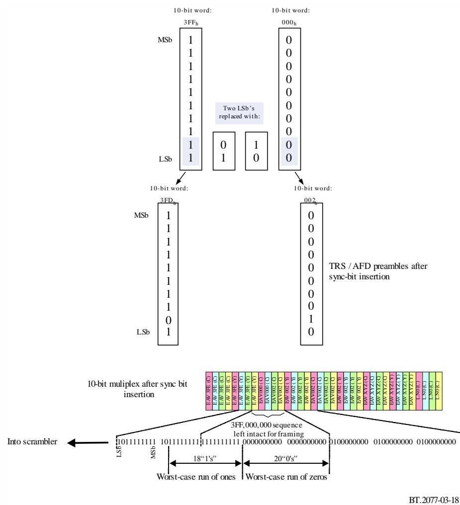
FIGURE 3-18 Sync-bit insertion process
