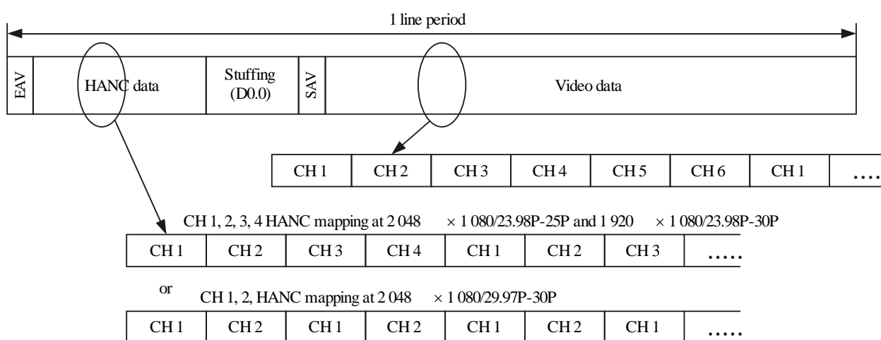
Data alignment structure of Mode B stream
