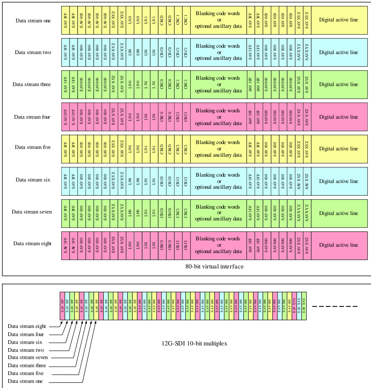
FIGURE 3-14 12G-SDI 10-bit Multiplex – Type 2
