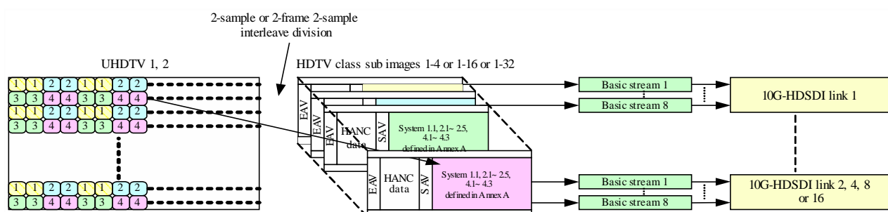
FIGURE 1-1 UHDTV mapping overview
