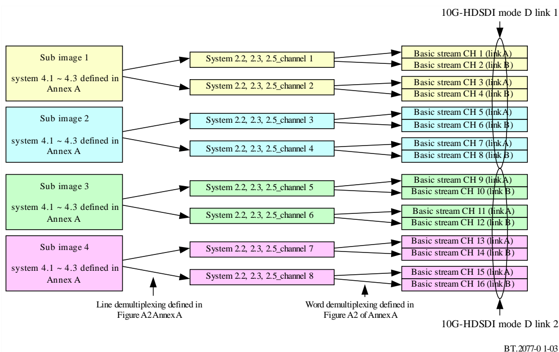
FIGURE 1-3 16 way division for Systems U1.7, U1.8 and U1.9
