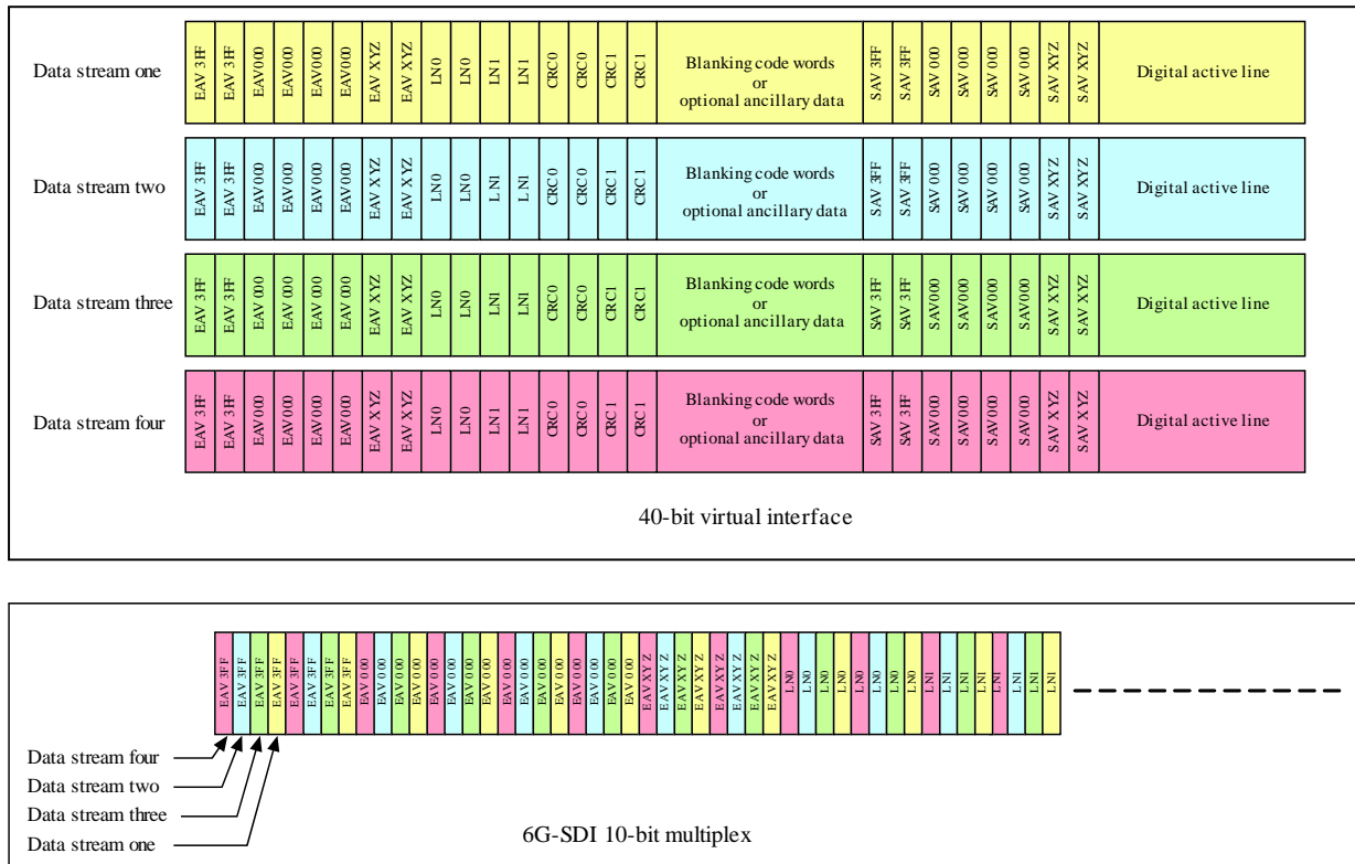
FIGURE 3-11 6G-SDI 10-bit Multiplex – Type 2
