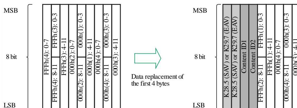
Multiplexed SAV and EAV data replacement with synchronization block (60, 60/1.001 or 50 Hz)
