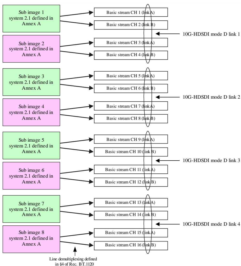
FIGURE 1-6 16 way division for System U1.6
