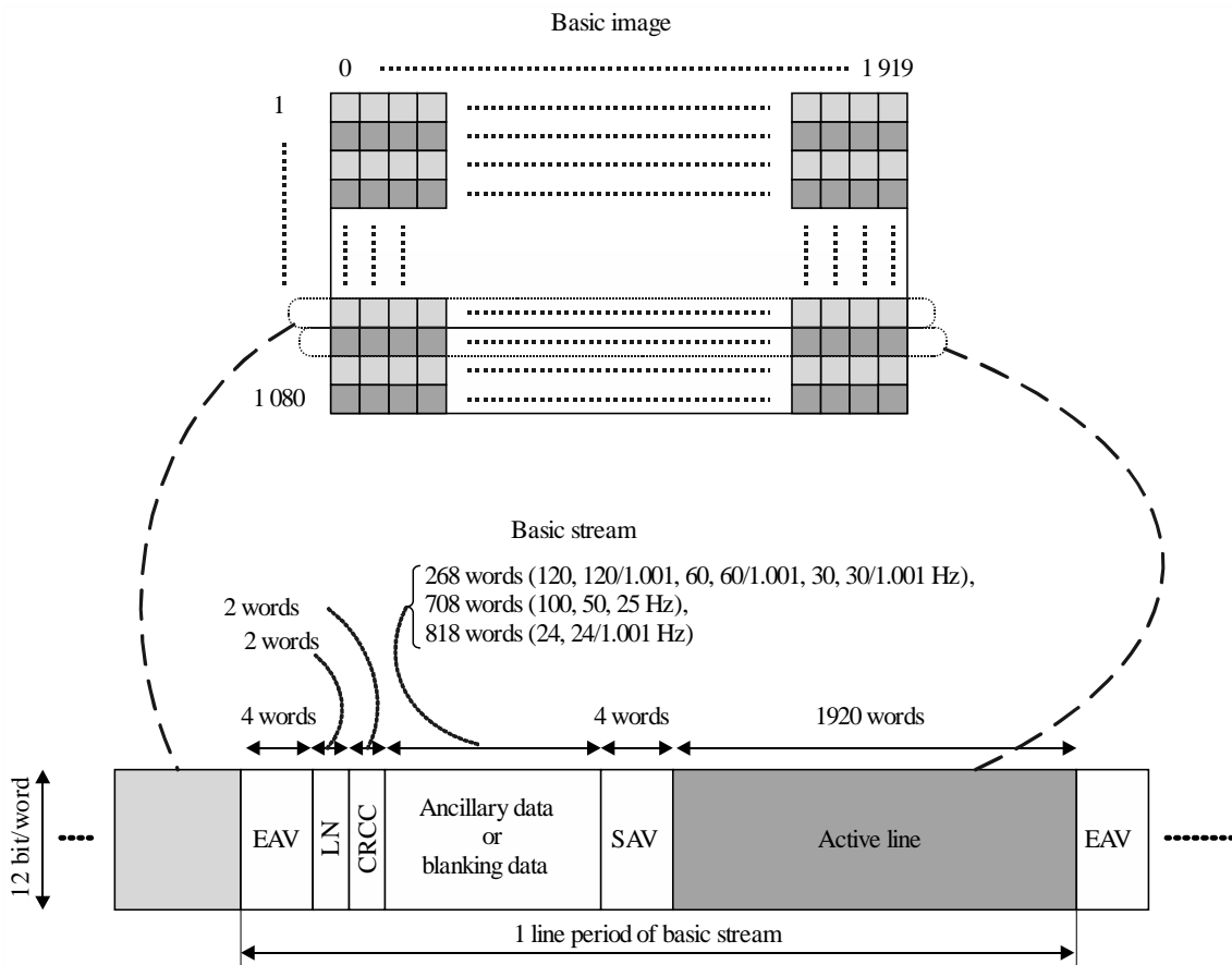
FIGURE 2-10 Line structure of basic stream
