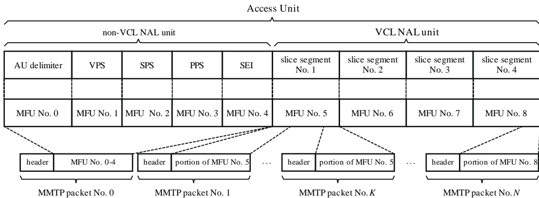
FIGURE 4 Overview of packetization of NAL units of HEVC streams
