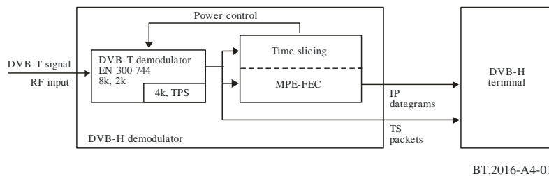
FIGURE A4-1 Conceptual structure of a DVB-H receiver
