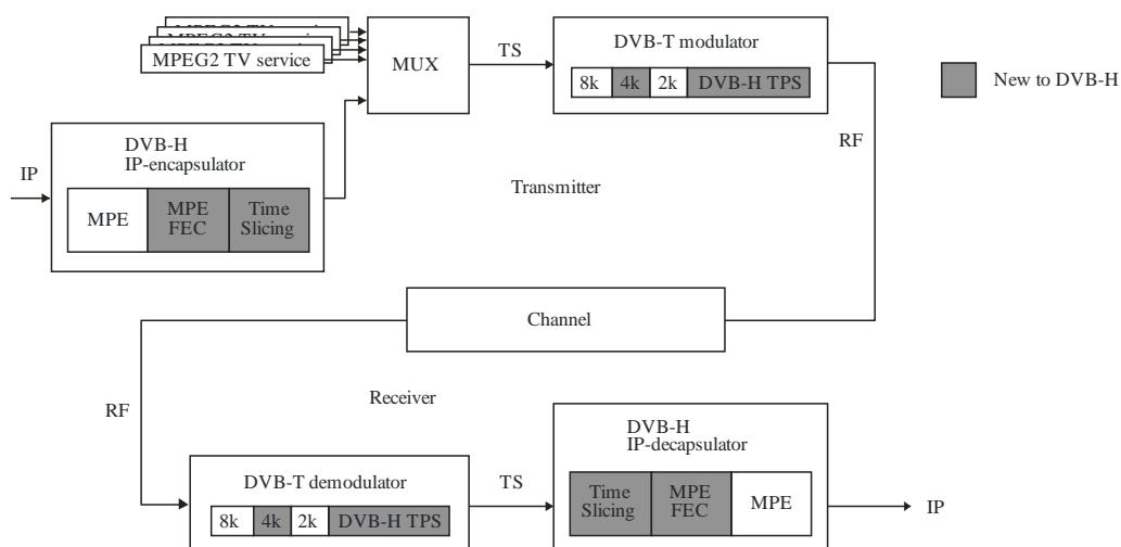
FIGURE A4-2 A conceptual description of using a DVB-H system (sharing a MUX with MPEG2 services)
