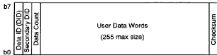
Figure 4 – Ancillary data packet format (Type 2 shown)
