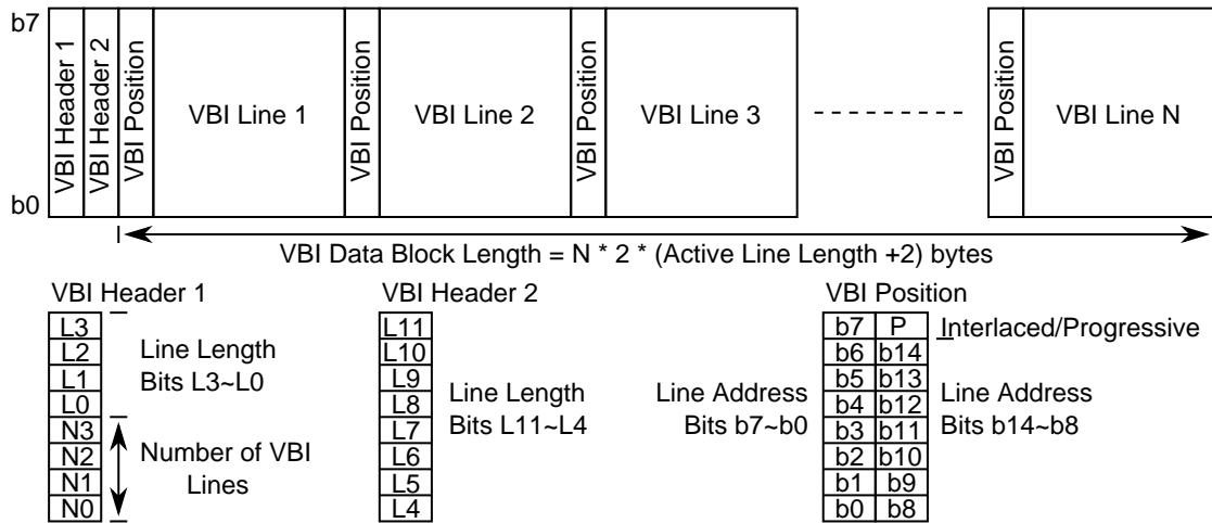
Figure 3 – VBI line format
