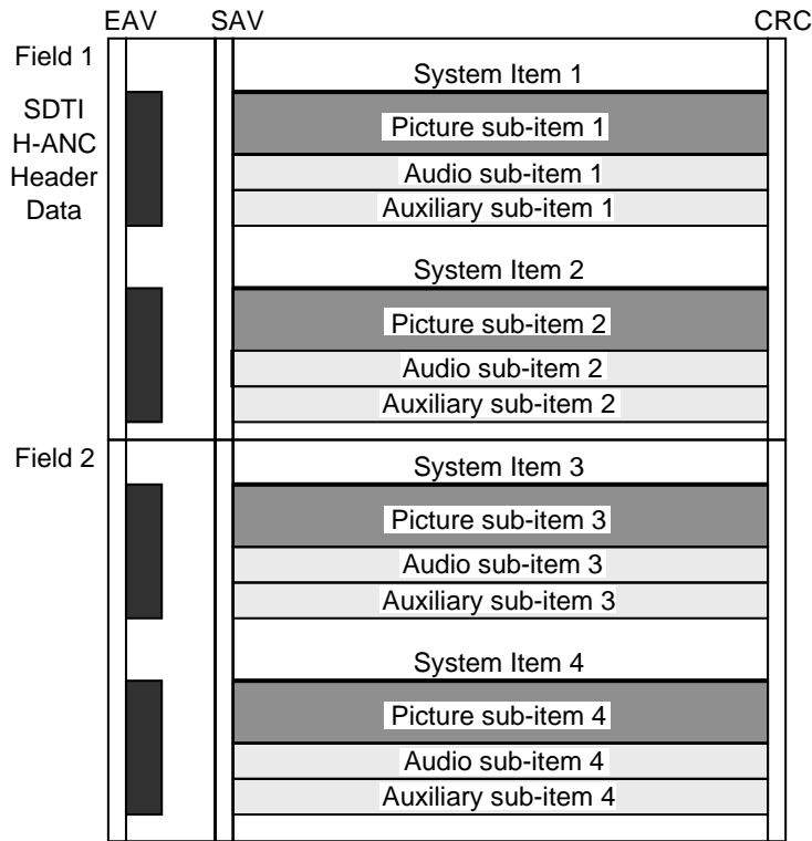
Figure 13 – Illustration of the low-latency transfer mode
