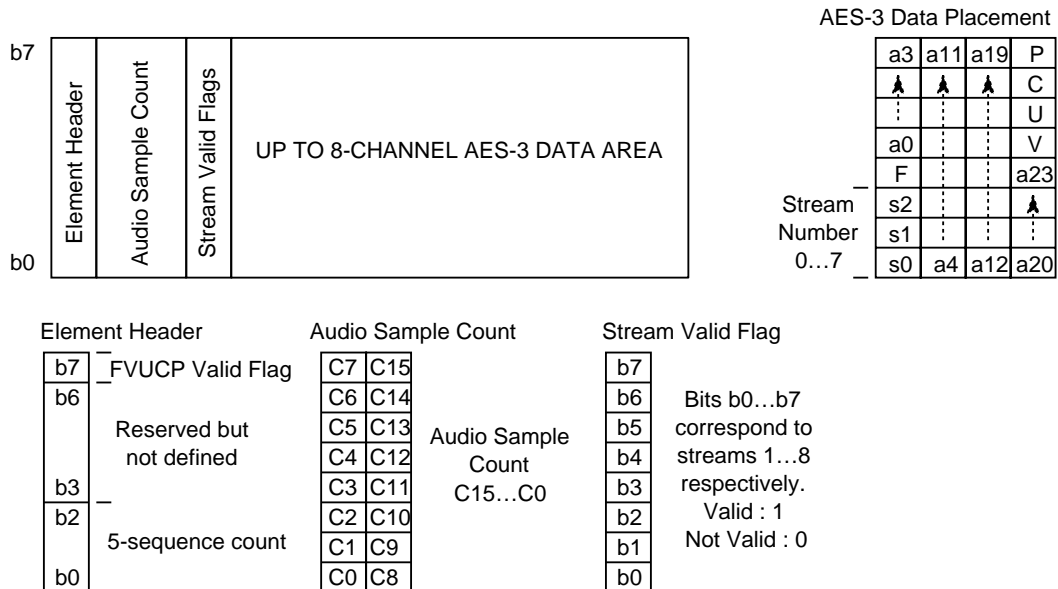
Figure 2 – Audio element format
