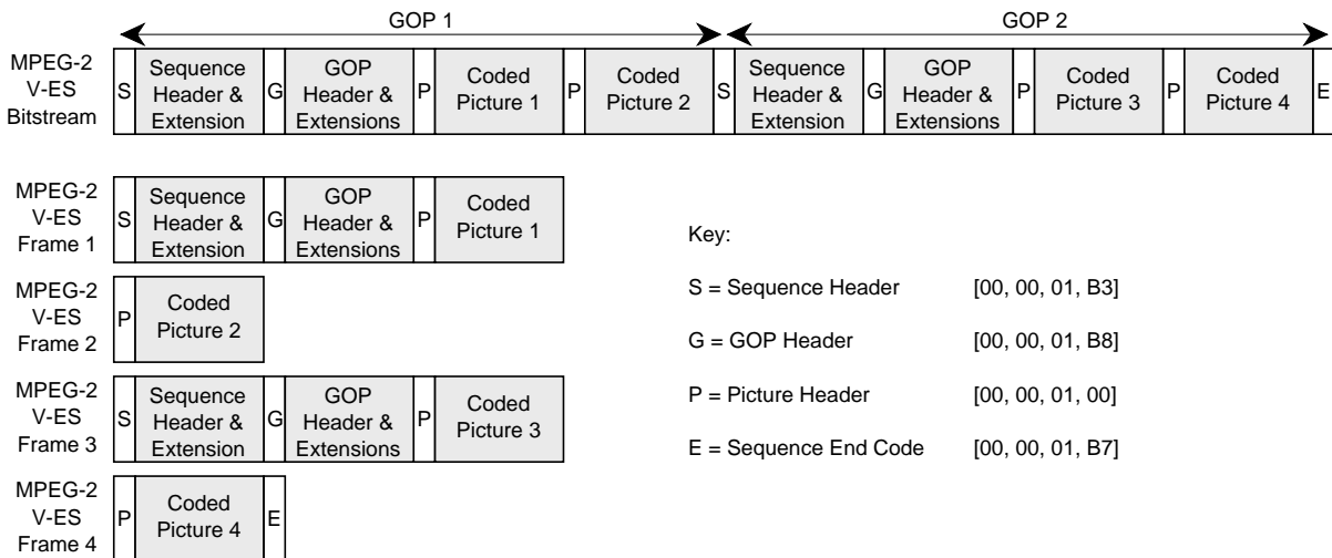
Figure 1 – Example formatting of a V-ES into SDTI-CP element frames
