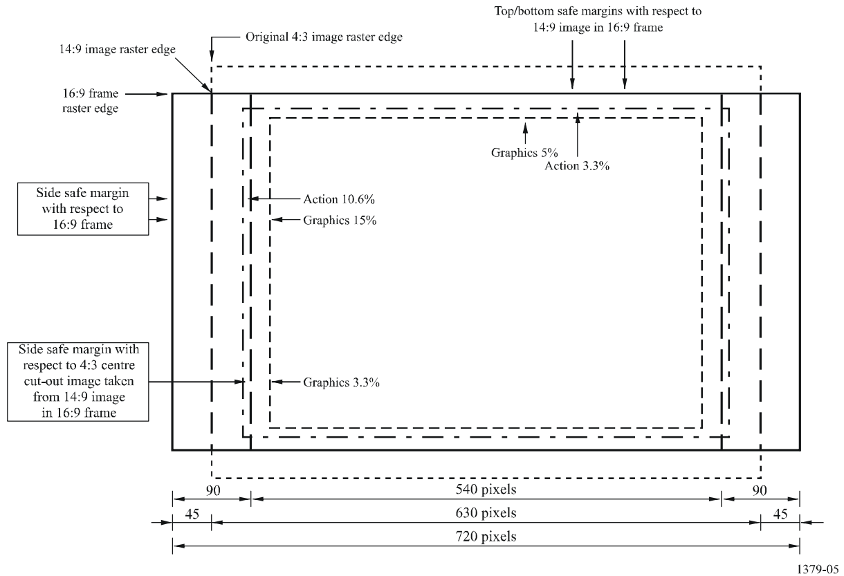
FIGURE 5 4:3 shoot-to-protect 14:9 action and graphics safe areas: resulting 14:9 image when transmitted within 16:9 frame
