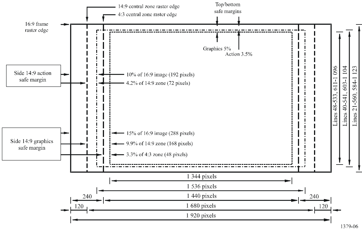
FIGURE 6 16:9 shoot-to-protect 14:9 action and graphics safe areas, 1080 lines
