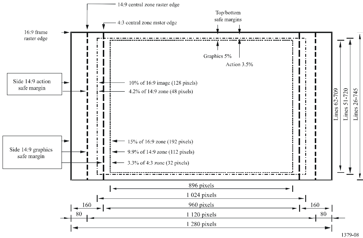
FIGURE 8 16:9 shoot-to-protect 14:9 action and graphics safe areas, 720 lines
