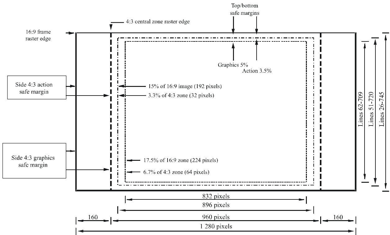
FIGURE 9 16:9 shoot-to-protect 4:3 action and graphics safe areas, 720 lines
