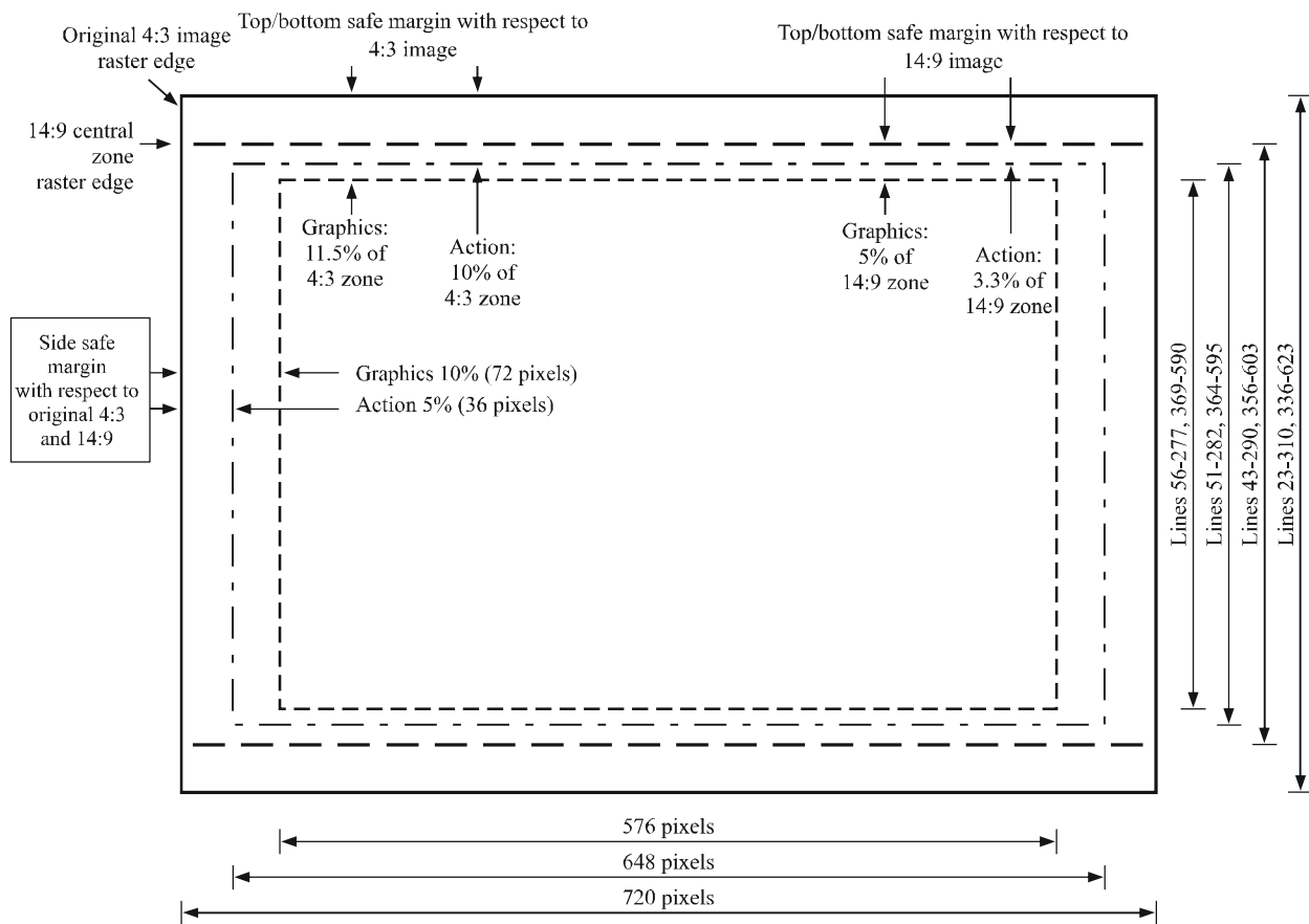
FIGURE 4 4:3 shoot-to-protect 14:9 action and graphics safe areas
