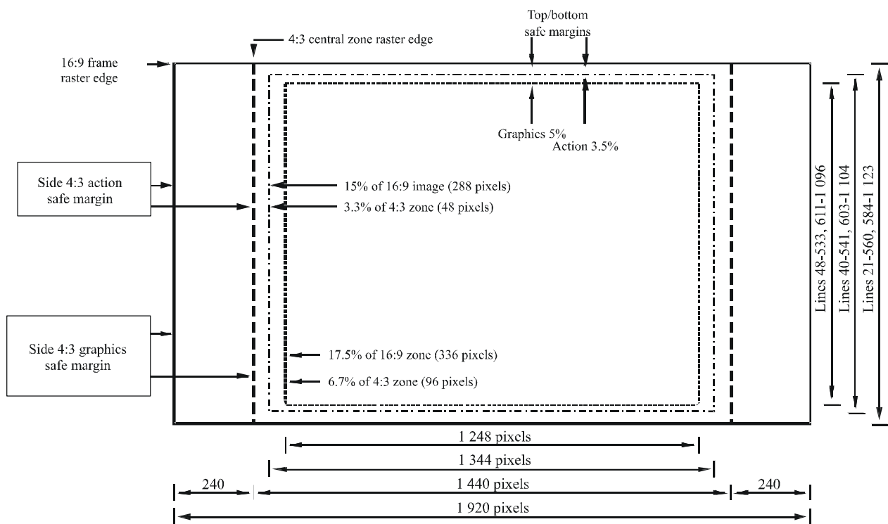
FIGURE 7 16:9 shoot-to-protect 4:3 action and graphics safe areas, 1080 lines
