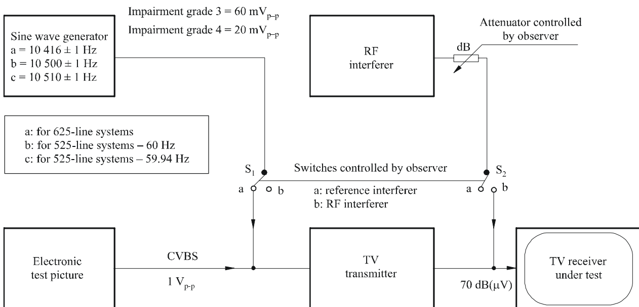
SCM for assessment of protection ratios
