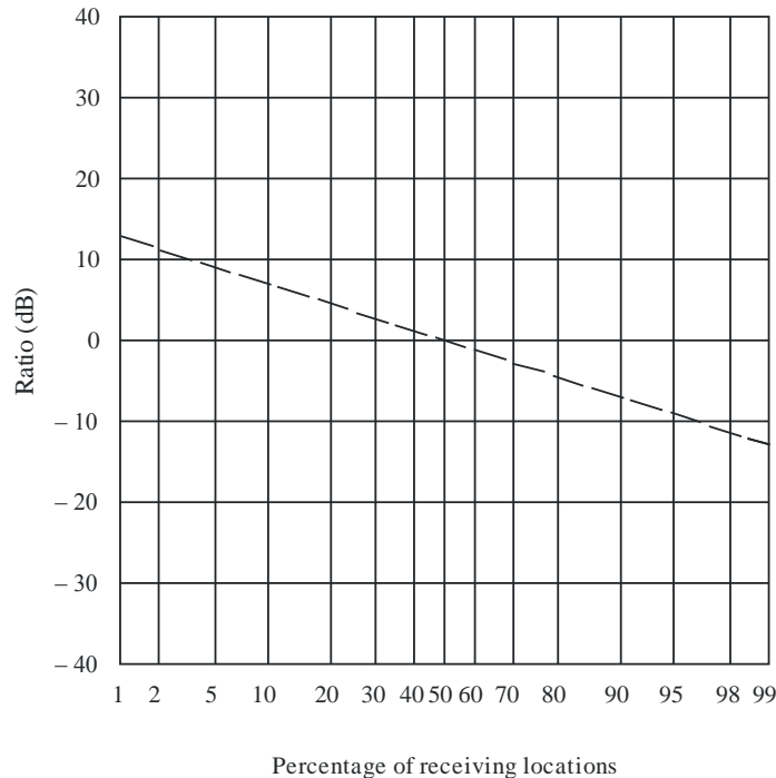
FIGURE 2 Ratio (dB) of the field strength for a given percentage of the receiving locations to the field strength for 50% of the receiving locations
