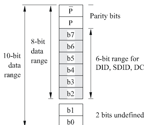
FIGURE 3 Coding range for 8-bit DID, SDID, DC
